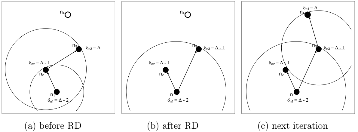
Figure 3.8: Illustrative Example for Restore Delay Procedure
