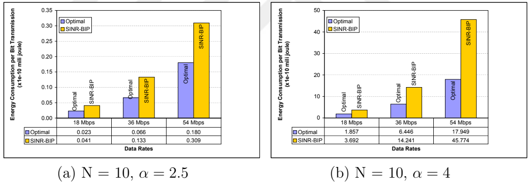
Figure 4.7: Energy Consumption per Bit Transmission of the Broadcast Trees Generated by SINR-BIP and the Optimal Solutions ( N = 10 )
