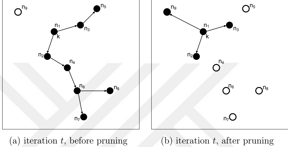
Figure 4.5: Illustrative Example for Cut_the_Branches ( v^* ) Procedure
