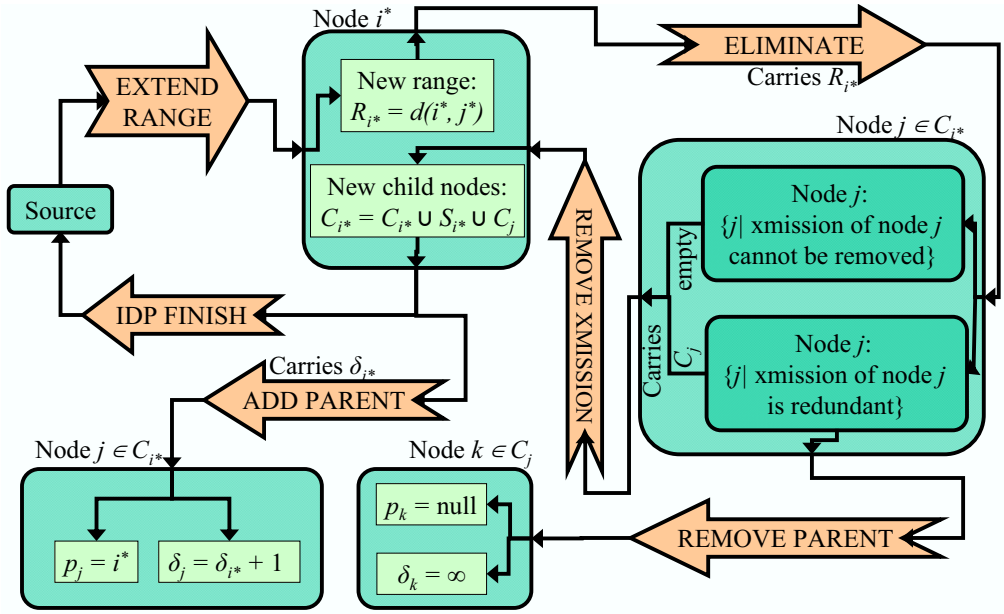
Figure 3.5: Information Dissemination Phase of DTE
