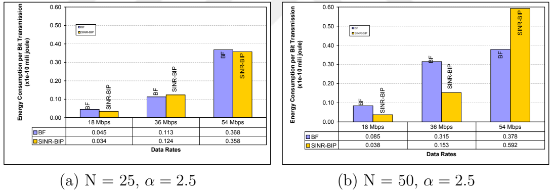
Figure 4.8: Energy Consumption per Bit Transmission of the Broadcast Trees Generated by SINR-BIP and the Best Feasible Solutions ( \alpha = 2.5 )
