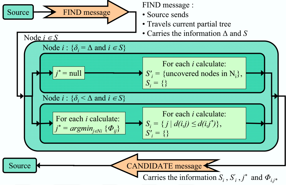
Figure 3.4: Information Collection Phase of DTE
