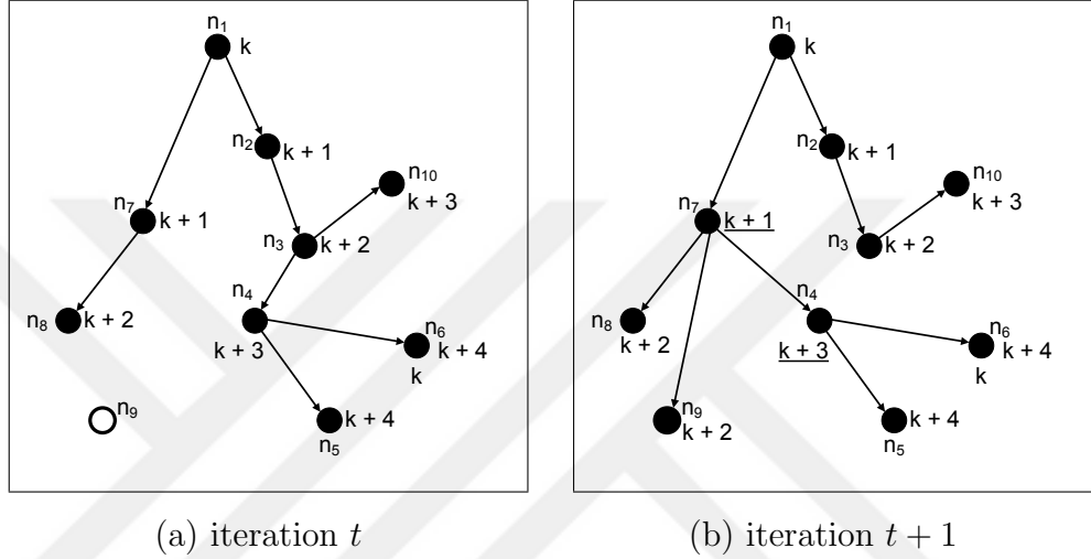
Figure 4.3: Illustrative Example for Level Update
