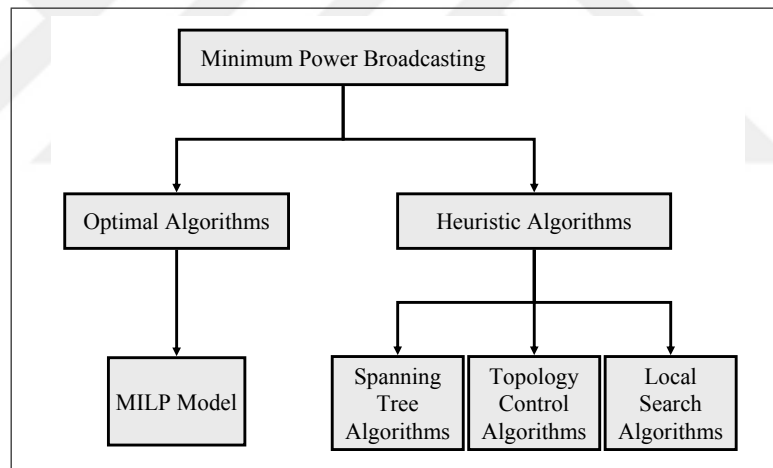
Figure 2.4: Classification for the Solution Methods of Minimum Power Broadcasting Problem
