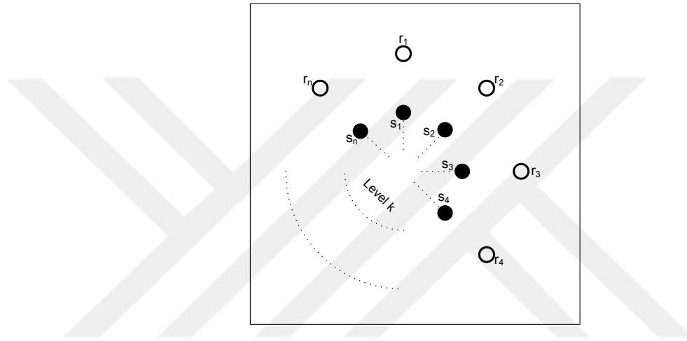
Figure 4.6: One-level Connectivity Problem; parent\_set and child\_set
