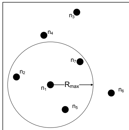
Figure 3.3: 1-hop Neighborhood of Node v ; N_{n_1} = \{n_2, n_5, n_7\}
