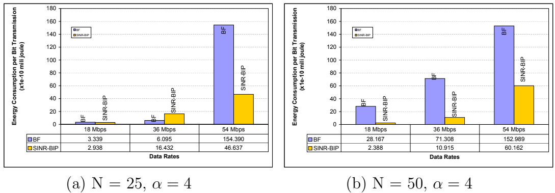
Figure 4.9: Energy Consumption per Bit Transmission of the Broadcast Trees Generated by SINR-BIP and the Best Feasible Solutions ( \alpha = 4 )
