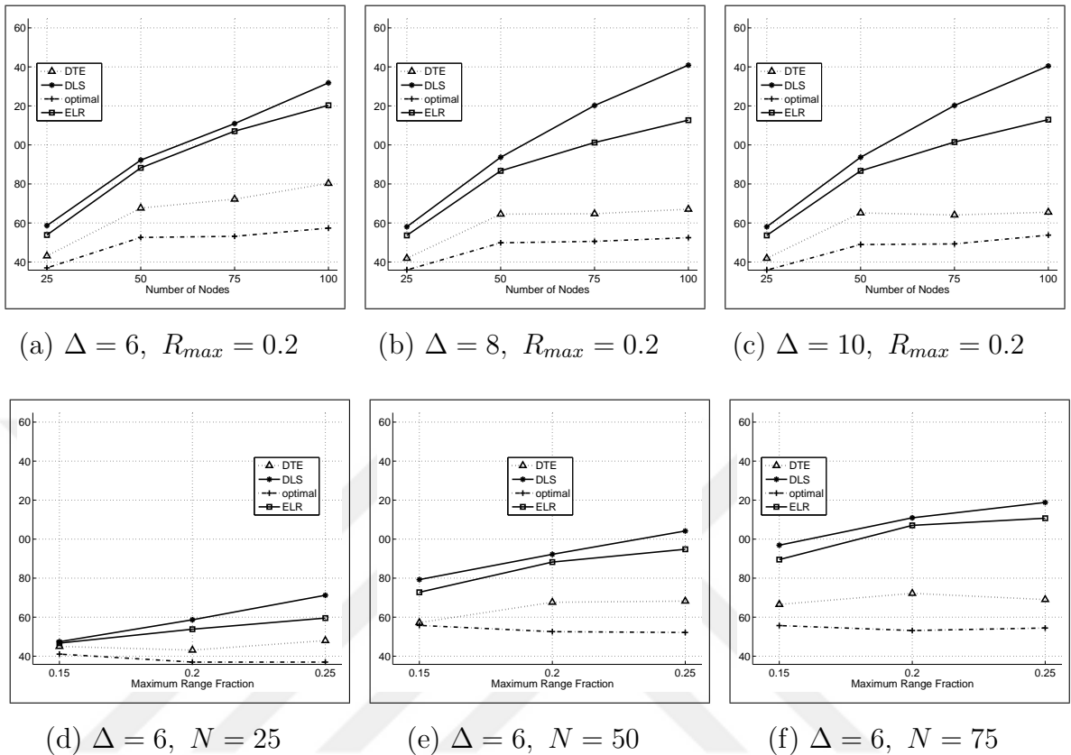
Figure 3.10: Total Transmission Power of Broadcast Trees Generated by Algorithms DTE, DLS, ELR and the Best Feasible Solution of IPs.
