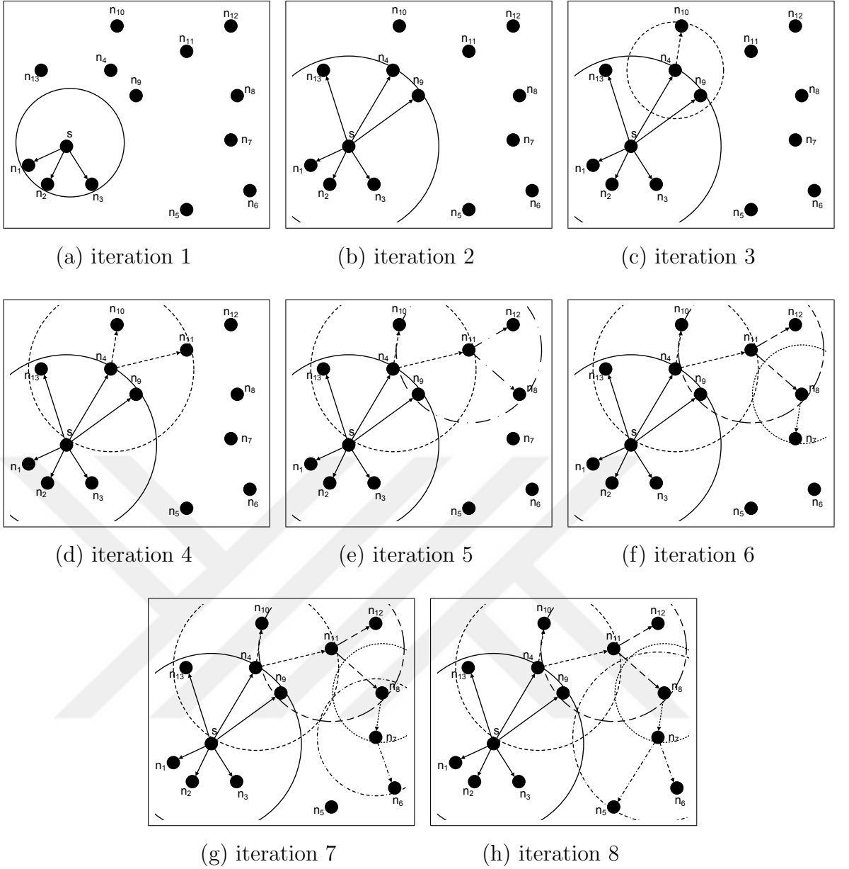
Figure 3.9: Illustrative Example for DTE
