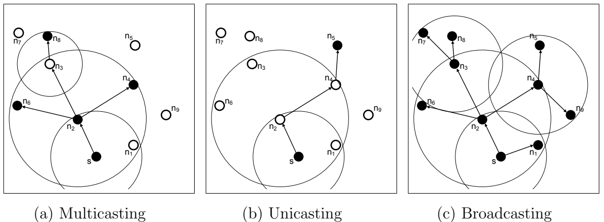
Figure 2.3: Data Dissemination Schemes
