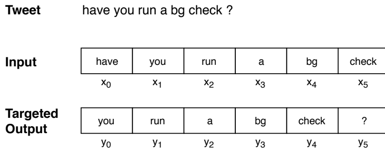
Figure 5.1: Training set prepared for next-word prediction task.
