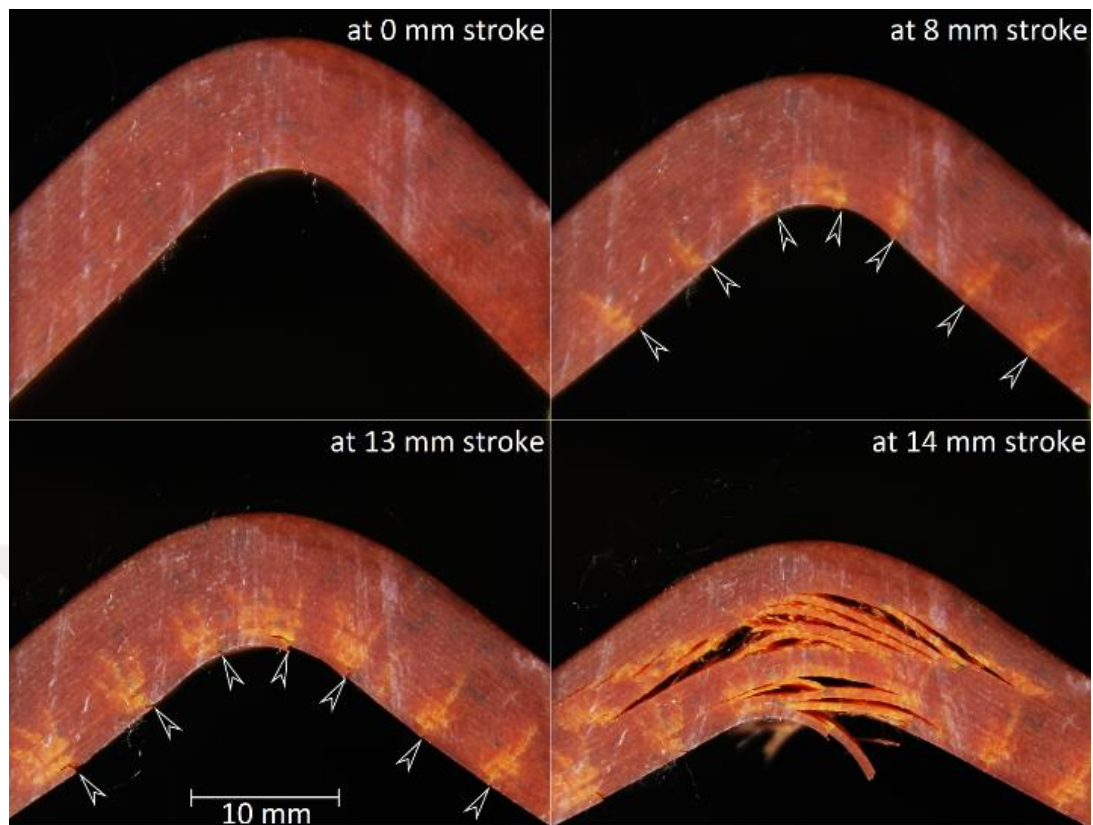
Figure 2.30. Matrix cracks formed and followed by delamination in GFRP [\pm 65]_{20} specimens
