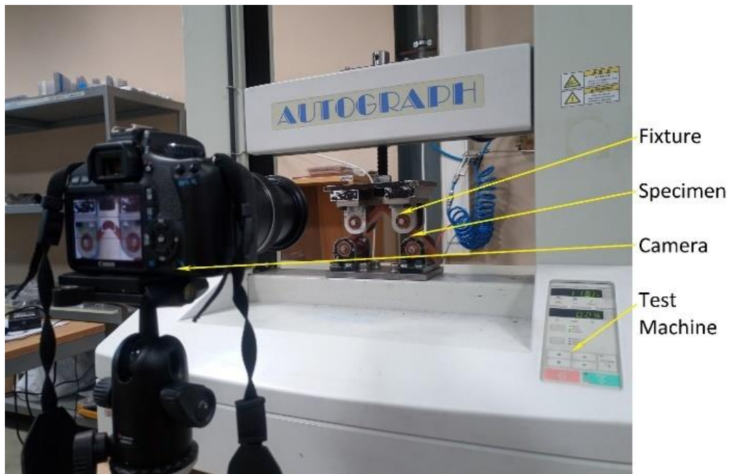
Figure 2.3. Experimental set-up
