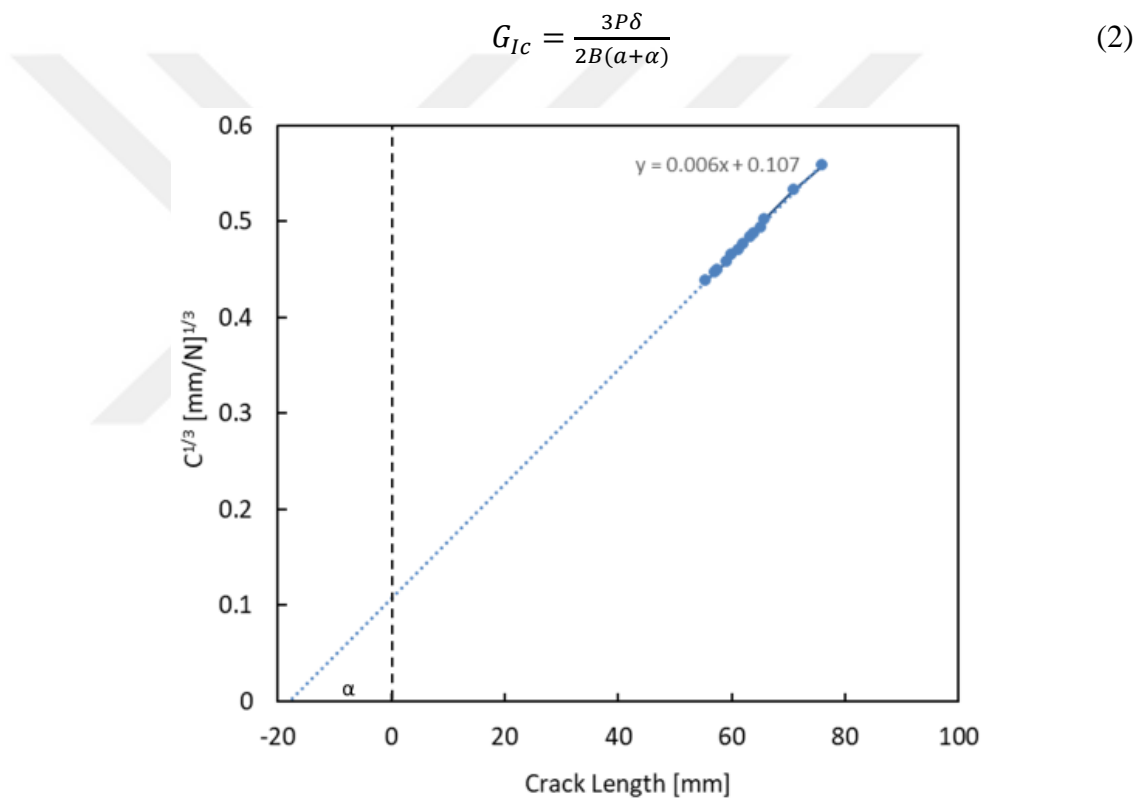
Figure 3.12. Graph of C^{1/3} vs crack length
