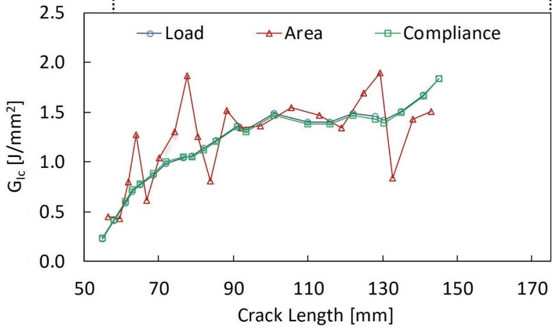
Figure 3.59. Fracture toughness results and fracture surface of specimen #1 (G-DCB-ENF-90-90-11-MF10723)
