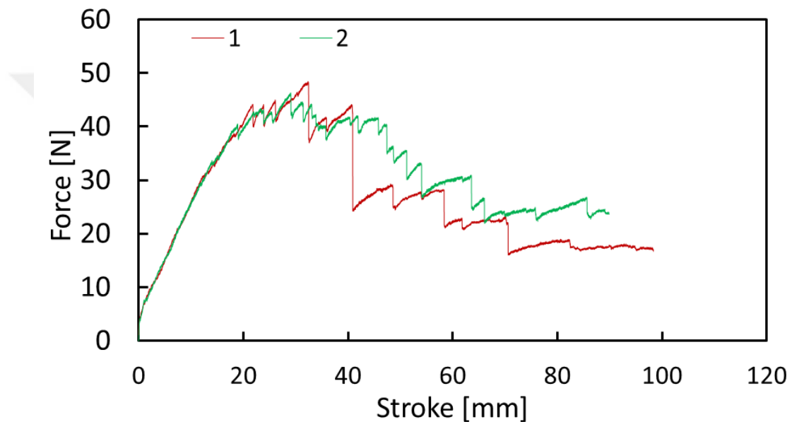
Figure 3.34. Load-displacement graph of CFRP 90//90 specimens
