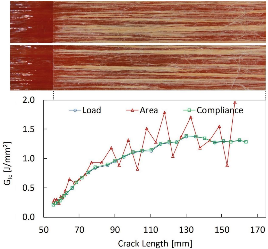
Figure 0.15. Fracture toughness results and fracture surface of (#1) G-DCB-ENF-0-0-5-MF11609
