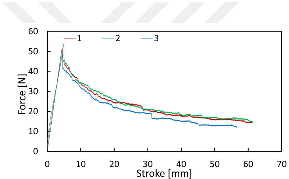
Figure 3.14. Load-displacement graph of CFRP 0//0 specimens
