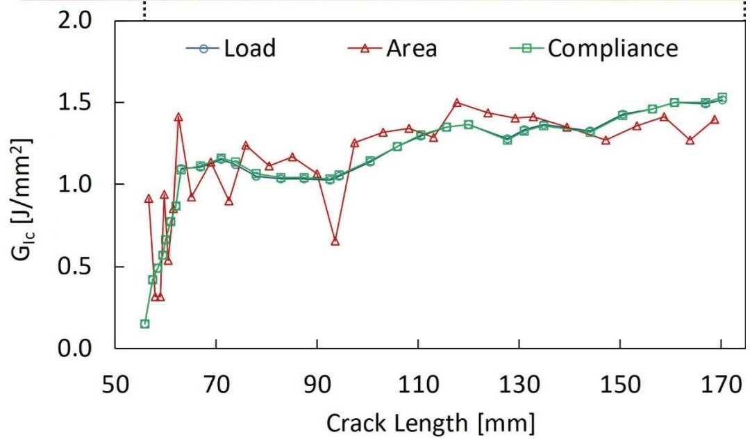
Figure 0.23. Fracture toughness results and fracture surface of (#1) G-DCB-ENF-65-65-1-MF12060
