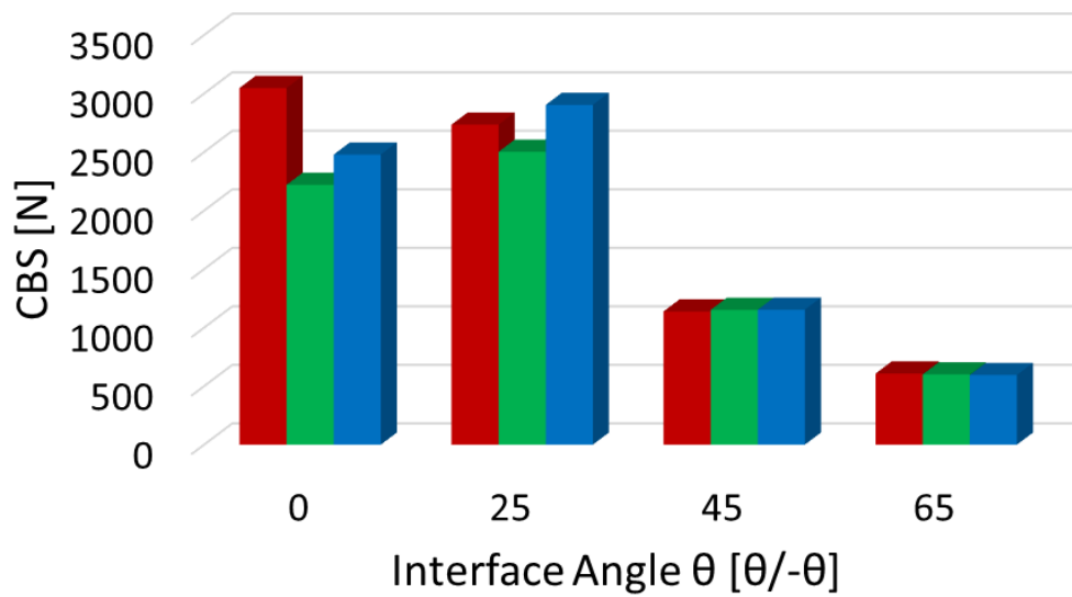
Figure 2.31. ILTS and CBS results for CFRP
