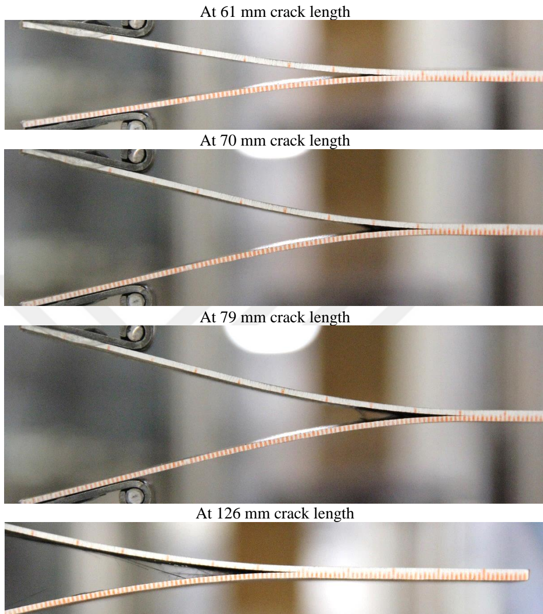
Figure 3.24. Side view of specimen #1 (C-DCB-ENF-45--45-1-MF11610) during DCB test
