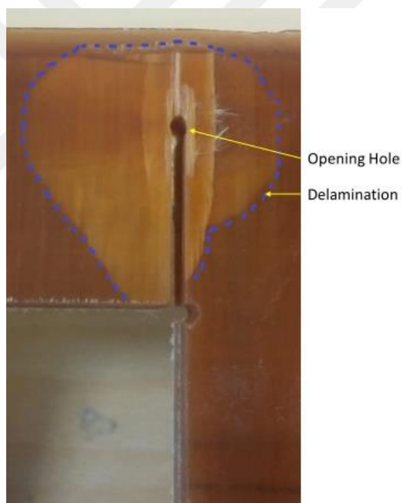
Figure 3.7. The delaminated hole opened with the water jet
