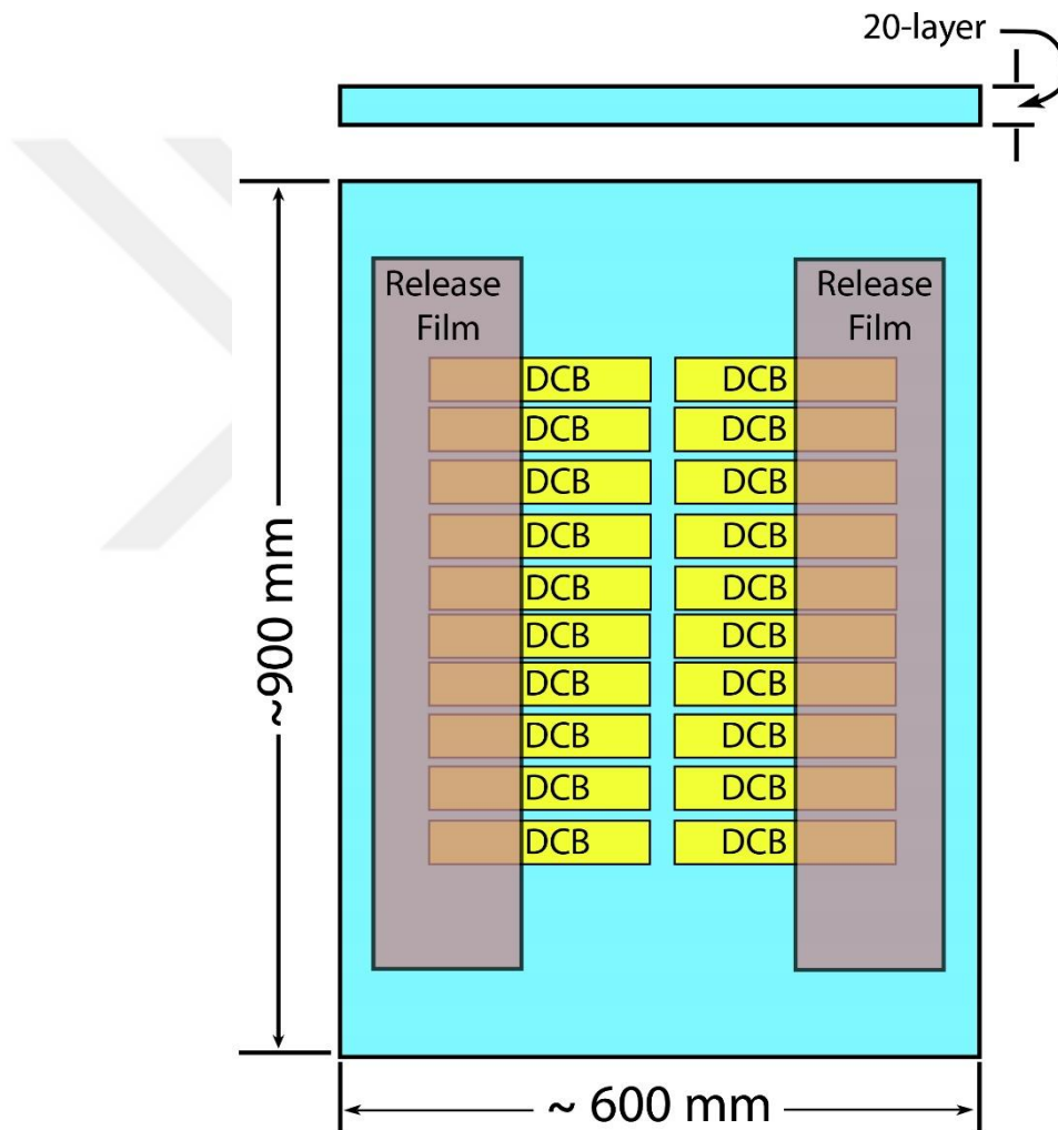
Figure 3.5. Produced laminate
