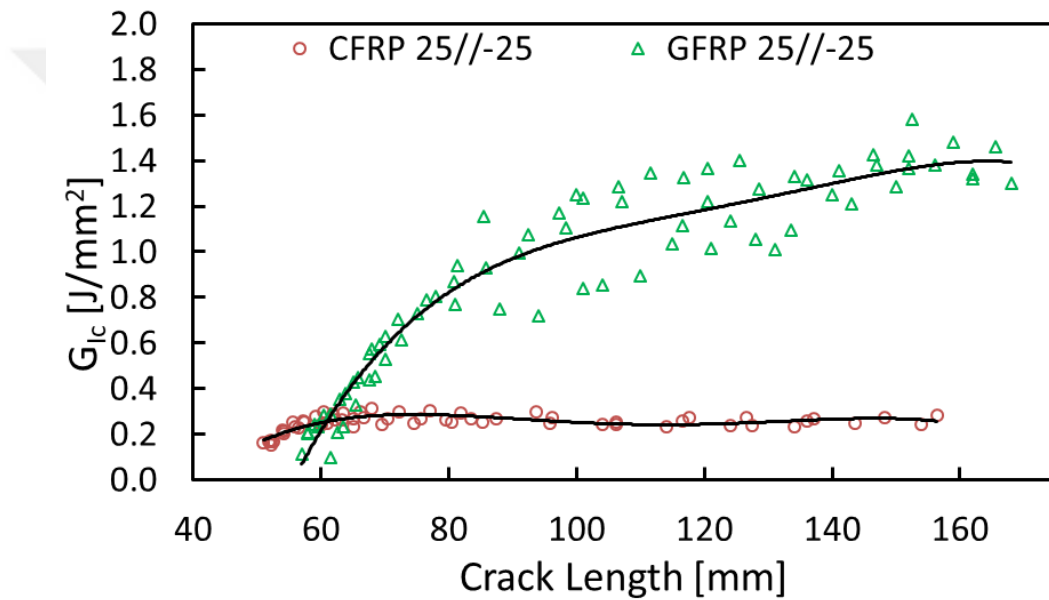
Figure 3.62. Comparison graph of CFRP and GFRP fracture toughness for 25// -25 interface
