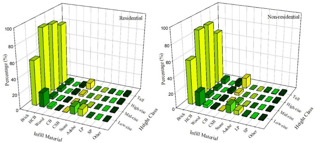
Figure B.18. Percentage of material of infill walls at residential and non-residential buildings with respect to height classes
