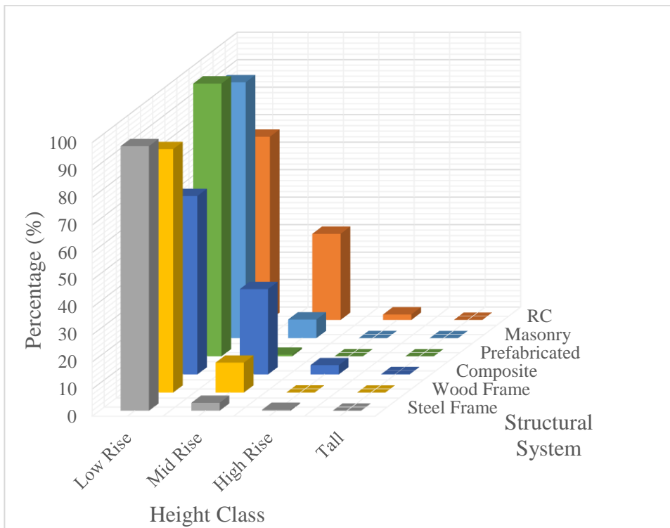
Figure 4.16. Variation of low, mid, high-rise and tall buildings in Turkey with respect to the structural system
