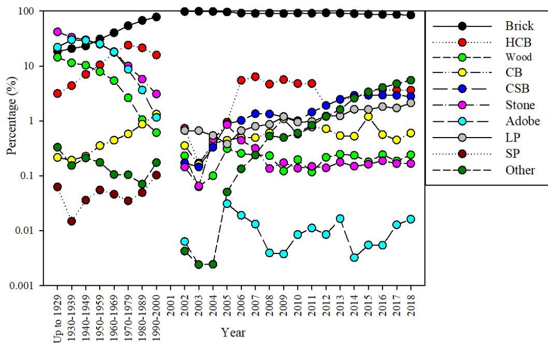
Figure 4.30. Annual variation of material of infill wall in Turkey
