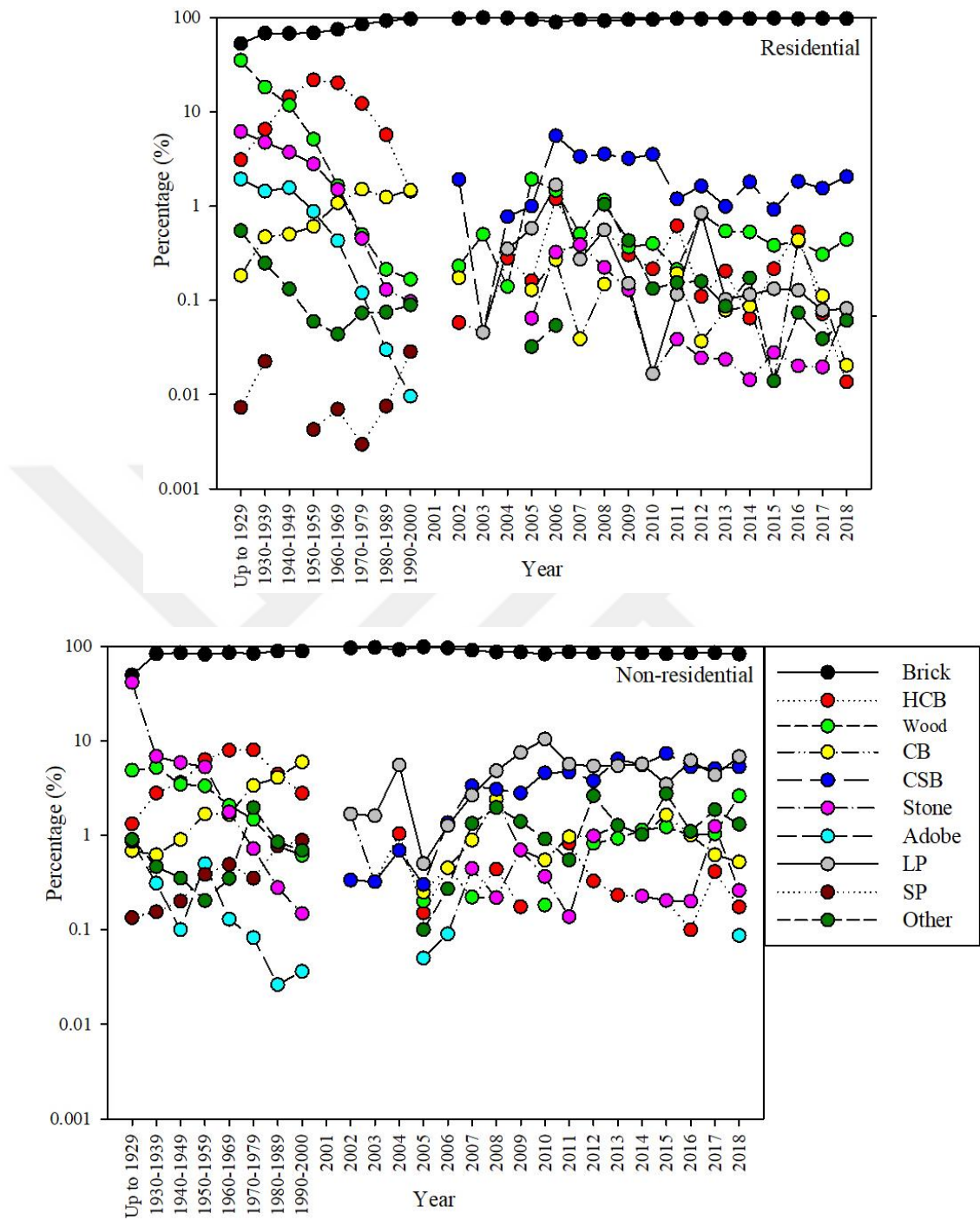
Figure B.20. Annual variation of material of infill wall percentage with respect to the use of building in İstanbul
