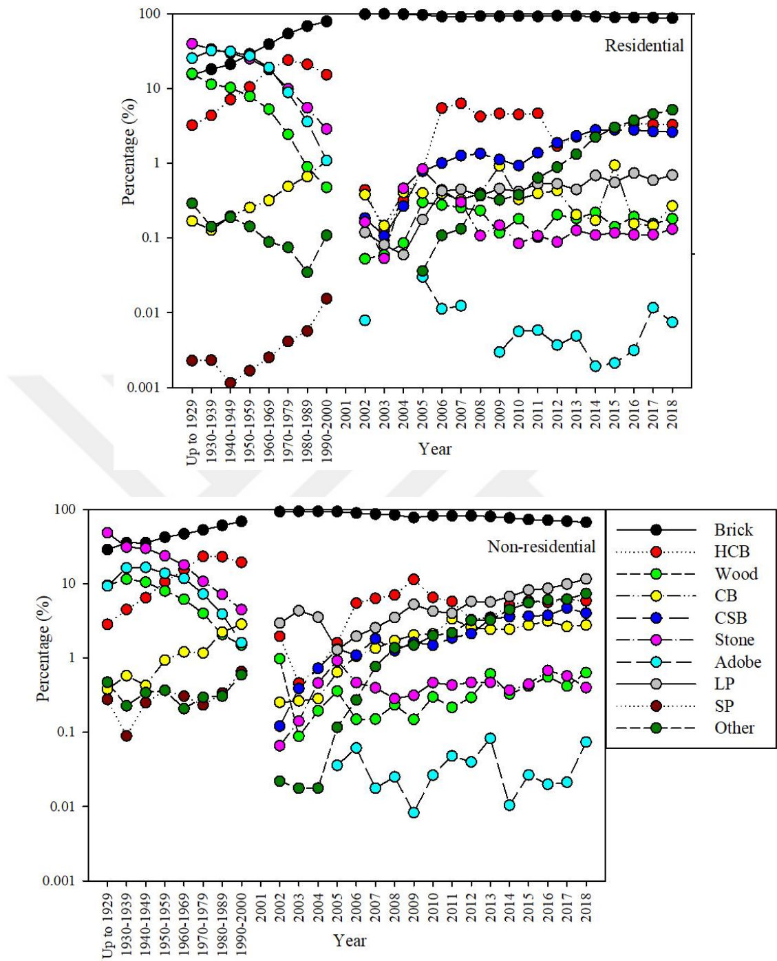
Figure B.17. Annual variation of material of infill wall in Turkey with respect to the use of building
