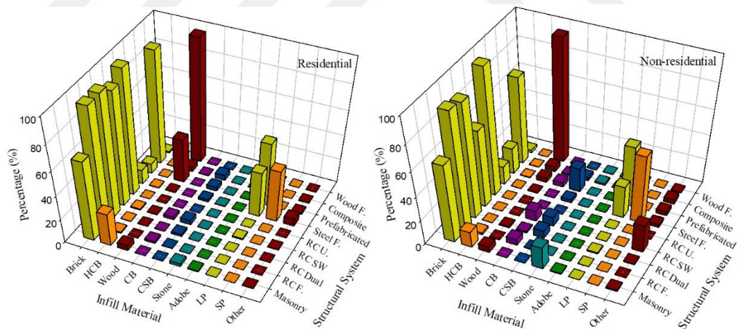
Figure 4.40. Percentage of material of infill walls at residential and non-residential buildings with respect to structural system in İstanbul
