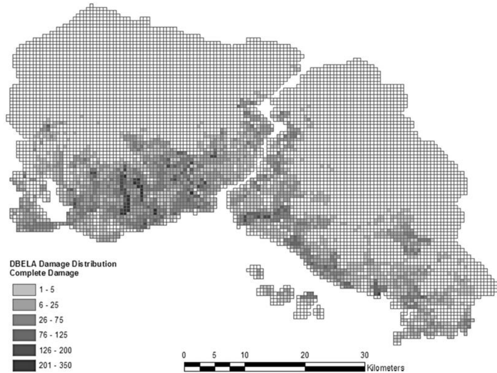
Figure 2.1. Spatial distribution of complete damage to all buildings in the Istanbul Metropolitan Municipality (Bal et al., 2008)
