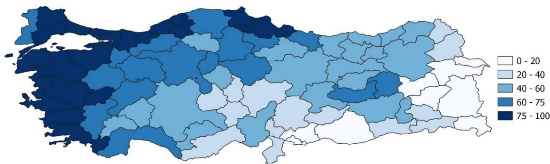
Figure 4.33. Percentage of brick for infill walls in Turkey at province level
