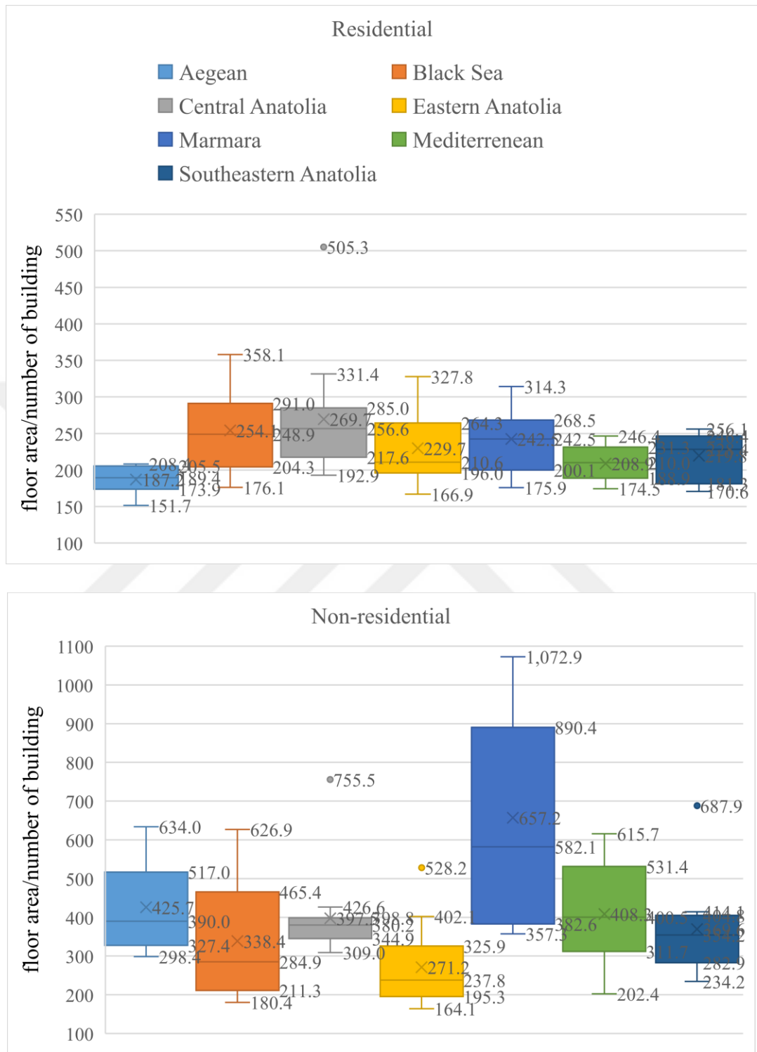
Figure 4.49. Ratio of total floor area (m 2 ) to number of building with respect to city administrative for residential and non-residential buildings in Turkish areas
