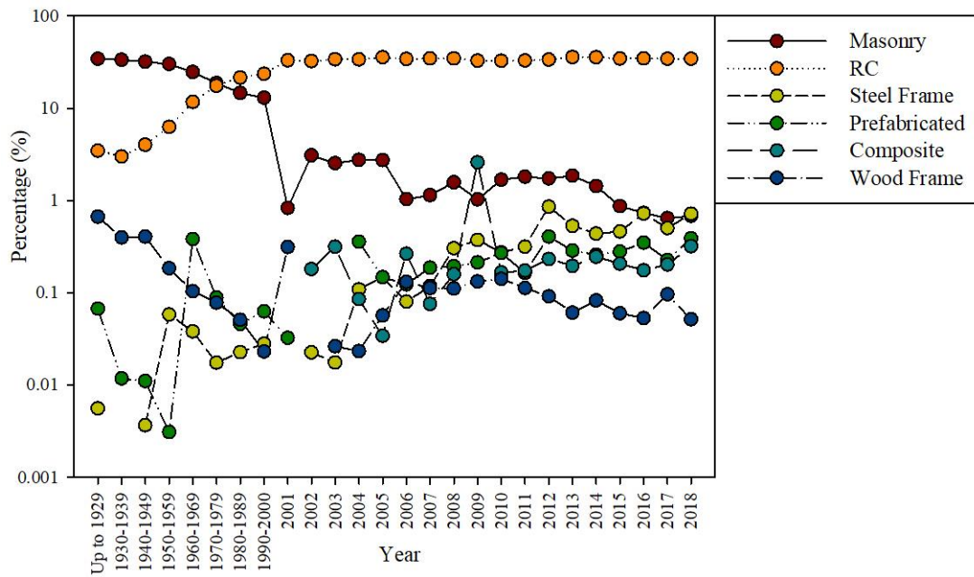
Figure 4.10. Annual structural system percentages in İstanbul
