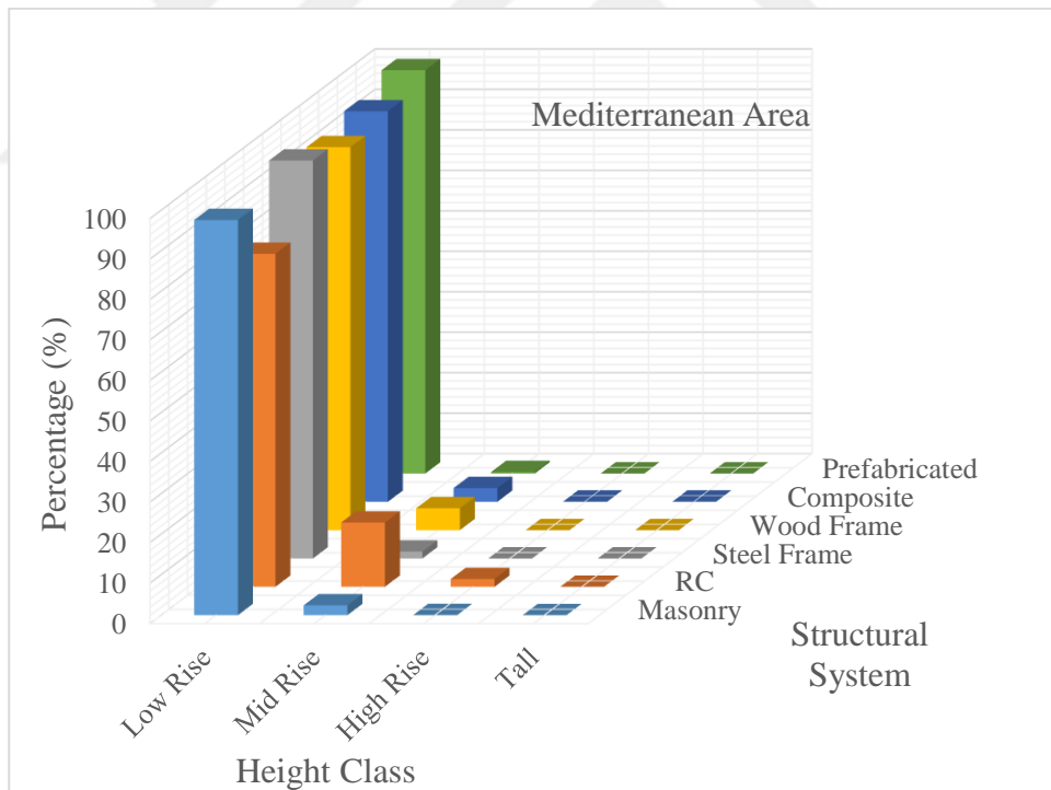
Figure B.13. Percentage of low, mid, high-rise and tall non-residential buildings with respect to structural system in Marmara and Mediterranean Areas
