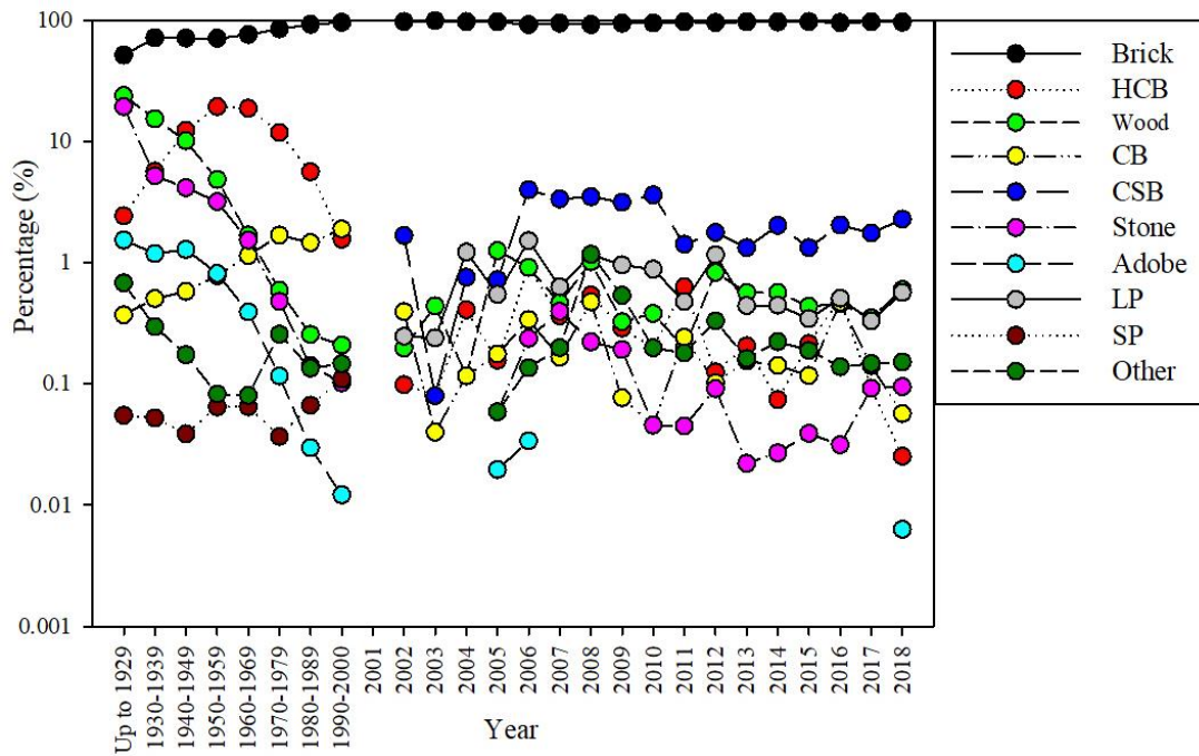
Figure 4.39. Annual variation of material of infill wall percentage in İstanbul
