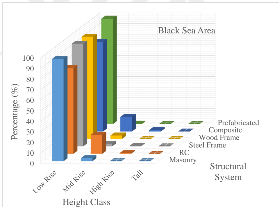
Figure B.11. Percentage of low, mid, high-rise and tall non-residential buildings with respect to structural system in Aegean and Black Sea Areas
