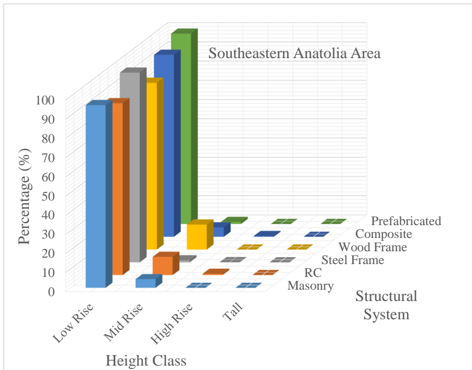
Figure B.14. Percentage of low, mid, high-rise and tall non-residential buildings with respect to structural system in Southeastern Anatolia Area
