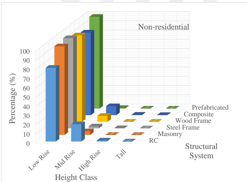
Figure B.4. Variation of low, mid, high-rise and tall buildings in Turkey with respect to the structural system for residential and non-residential buildings
