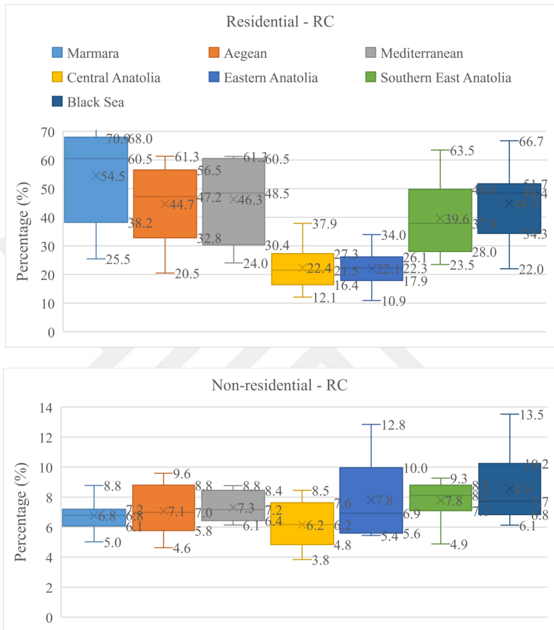
Figure B.1. The percentage of RCF structural system for residential and non-residential buildings with respect to Turkish regions
