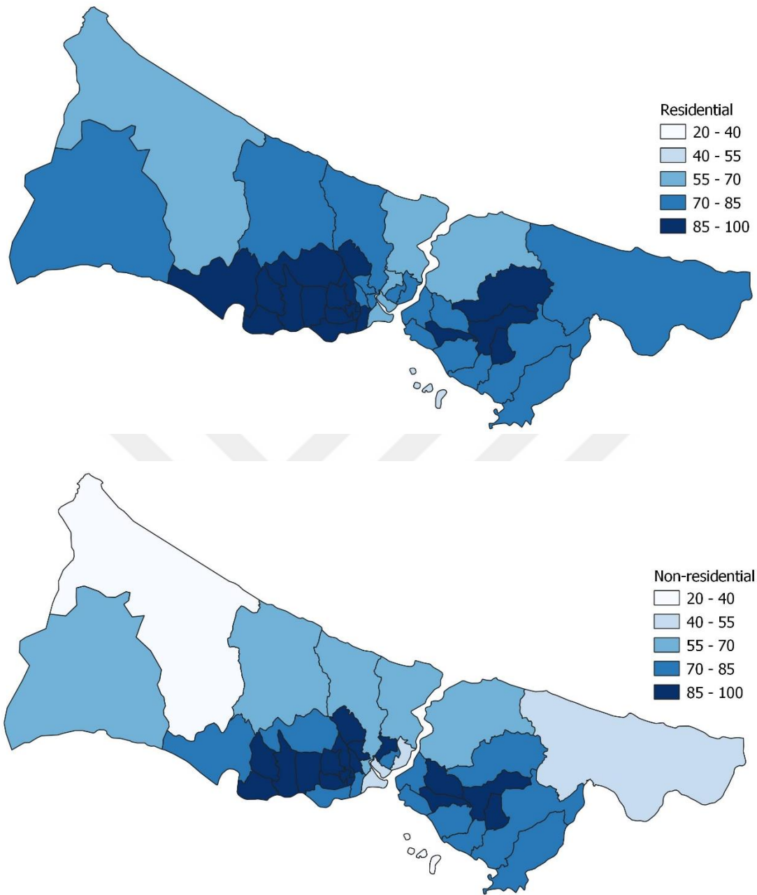
Figure 4.13. RC structural system percentages in residential and non-residential buildings in İstanbul at district level
