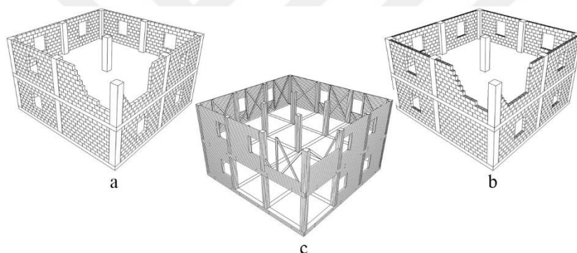
Figure 4.31. Sketches about common structural system and infill wall material in Turkey
