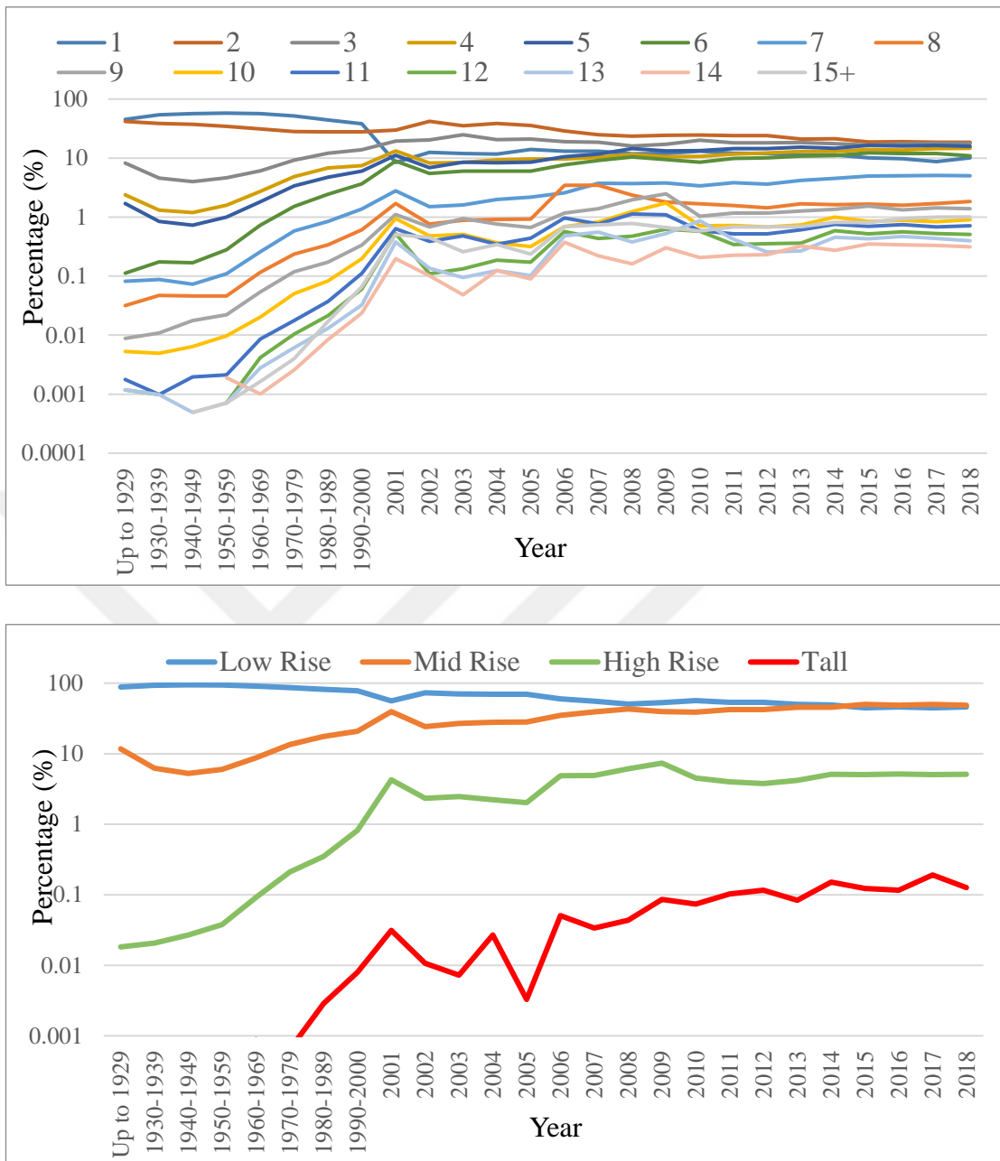
Figure B.3. Annual variation of Turkish building number of stories percentages
