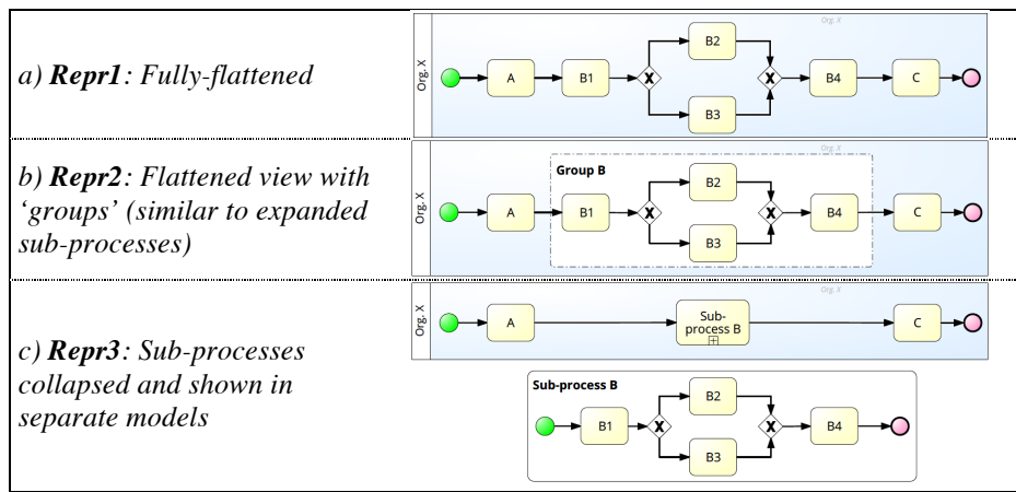
Figure 9 Three modularity representations: a) Fully-flattened [Repr1], b) Flattened view with groups [Repr2], and c) Sub-processes collapsed and shown in separate models [Repr3]
