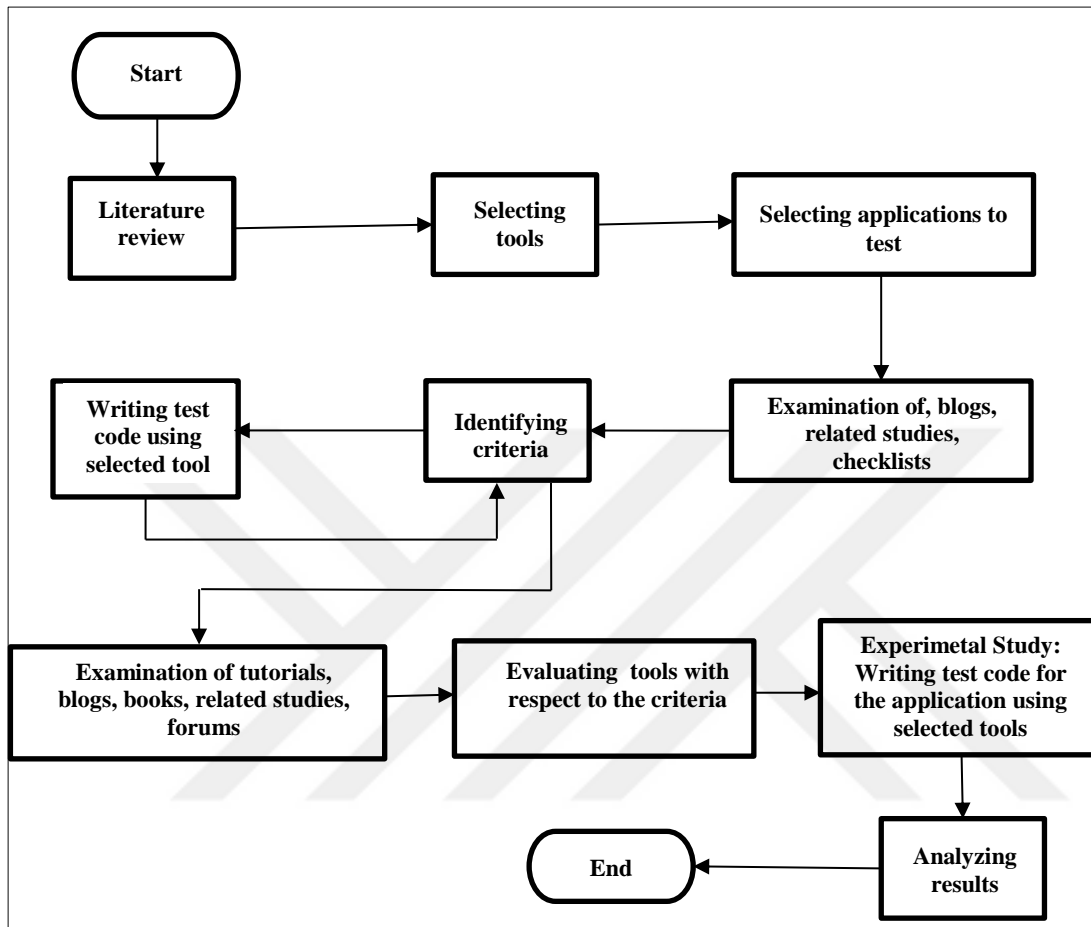
Figure 3.1: Research Methodology
