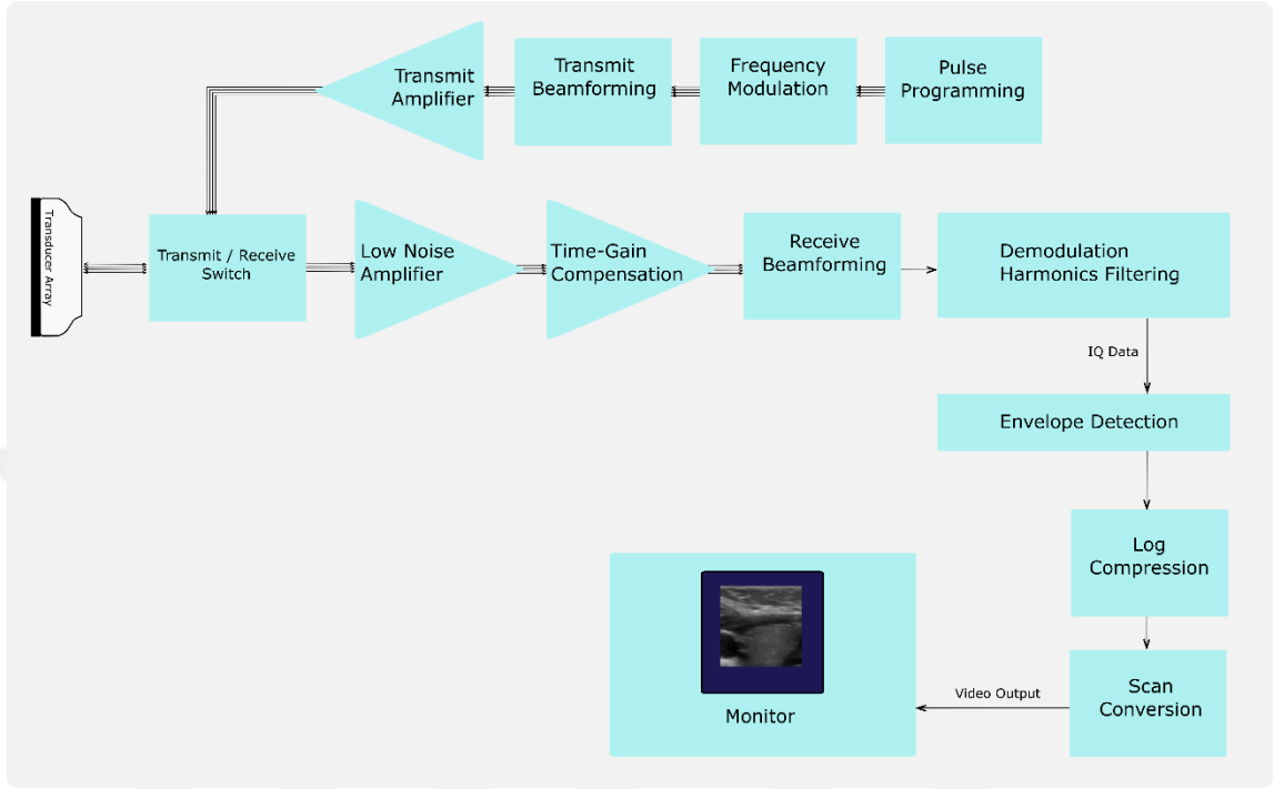
Figure 12: Steps of B-Mode image formation. Figure was previously published in (Cüneyitoğlu Özkul & Mumcuoğlu, 2018).
