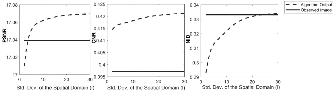
Figure 37: Parameter optimization for BF, using synthetic phantom with respect to objective evaluation metrics.
