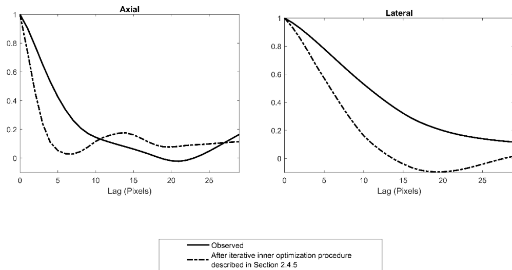
Figure 31: Autocorrelation was observed to be reduced by the inner optimization scheme mentioned in Optimization section (2.4.5).
