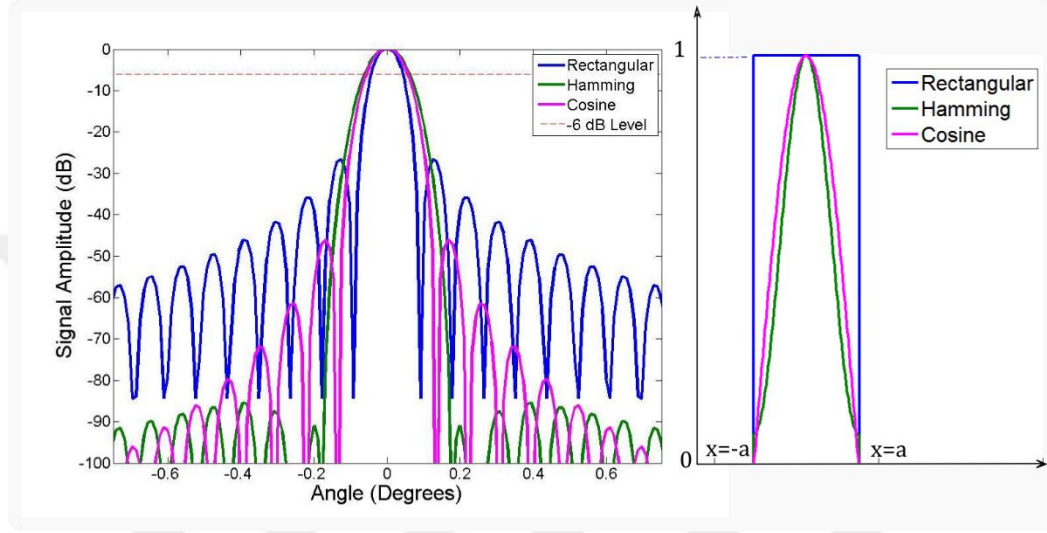
Figure 8: The beam plot for the selected transmit and receive aperture function and the apodization. Figures were previously published in (Cüneyitoğlu Özkul & Mumcuoğlu, 2018).
