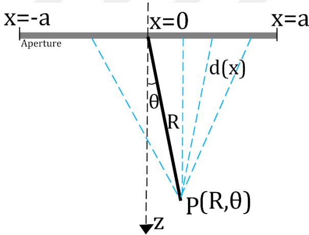
Figure 6: Distance function from a point to transducer surface is defined. Figure was previously published in (Cüneyitoğlu Özkul & Mumcuoğlu, 2018).
