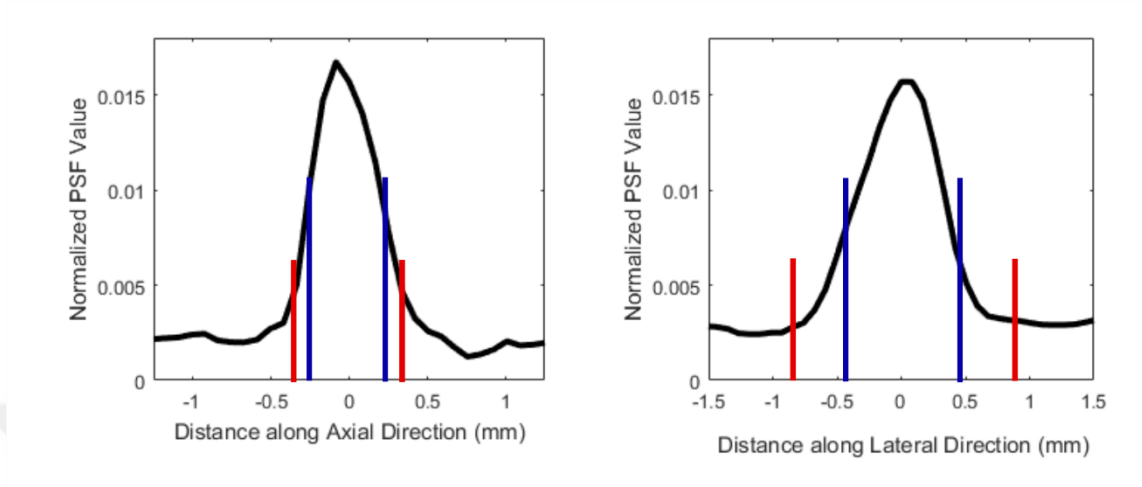
Figure 28: Cross sections from the PSF estimates. Along axial and lateral directions, image observation method using tissue-mimicking phantom data was used. Blue lines mark FWHM and red lines mark the extent of the PSF.
