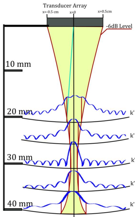
Figure 9: Beam plots at several depths form the curve that defines overall lateral resolution (yellow area) for a single focus placed at 30 mm. Figure was previously published in (Cüneyitoğlu Özkul & Mumcuoğlu, 2018).
