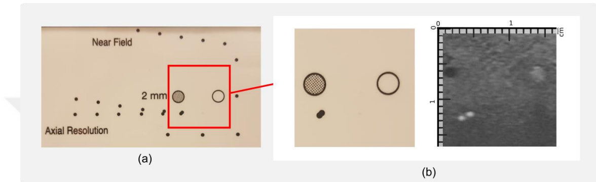
Figure 20: Tissue-mimicking resolution phantom CIRS 044 (a) Picture of imaged area; (b) Selected 180x180 pixels (16.2x16.2 mm) region.
