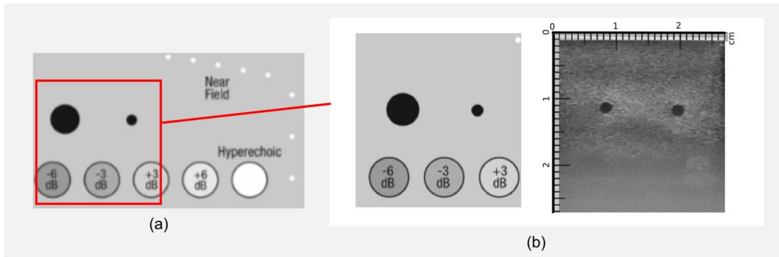
Figure 19: Tissue-mimicking resolution phantom CIRS 040GSE (a) Drawing of all imaged area from CIRS Tissue Simulation & Phantom Technology (2019); (b) Selected 300x300 pixels (27x27 mm) region from acquired images. The radii of the anechoic targets are stated to vary along elevation, this is why the target to the left side differs from drawing.
