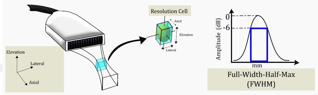
Figure 7: Ultrasound image axes, resolution cell and full-width-half-maximum (FWHM). Figures were previously published in (Cüneyitoğlu Özkul & Mumcuoğlu, 2018).
