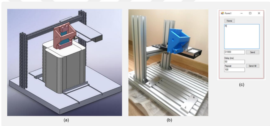
Figure 23: The designed system for 1D scanning (a) Computer aided design of 1D scanning system in Solidworks® 2008 environment – Red part: 3D printed probe holder, blue part: ultrasound probe, white box: bounding box for tissue-mimicking phantom; (b) Manufactured and assembled system; (c) Simple control interface program written in C#.
