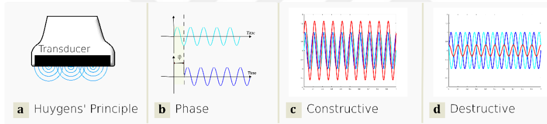
Figure 1: Huygens' principle, illustration of phase, constructive and destructive interference of waves. Figures were previously published in (Cüneyitoğlu Özkul & Mumcuoğlu, 2018).
