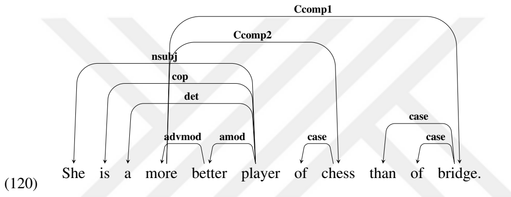
Figure 6.8: Our Output Parse for a Nominal Comparative with Prepositional Comparatives
