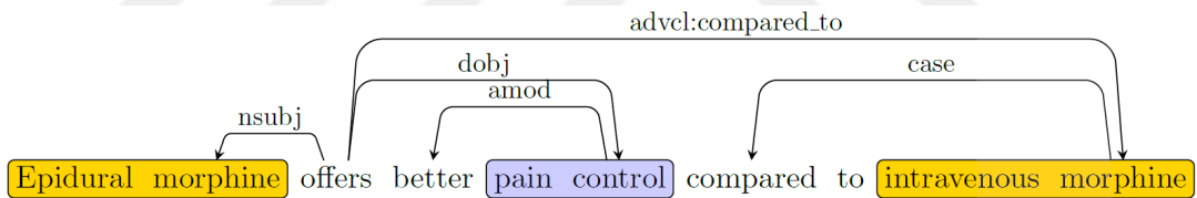
Figure 4.7: Comparative adjectives as noun modifier (Gupta et al., 2017)
