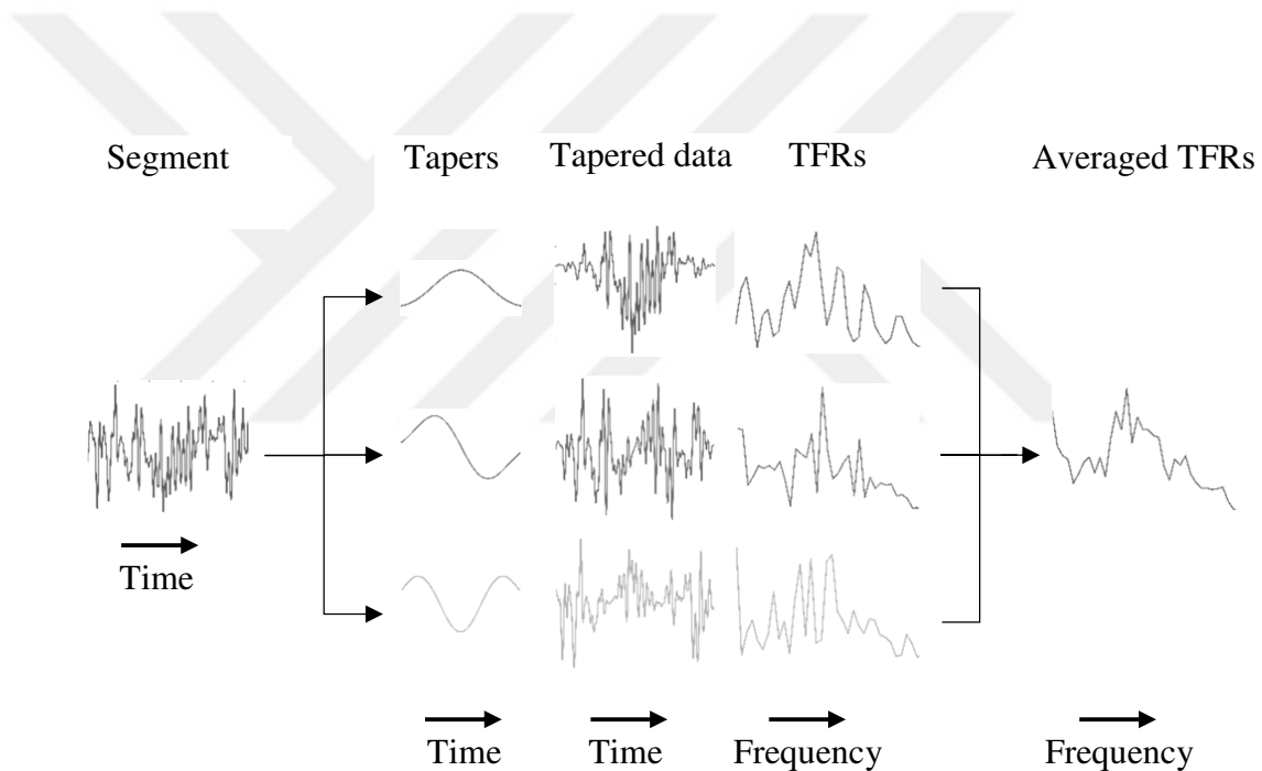
Figure 6: Diagram illustrating the steps applied by the multitapering method.
