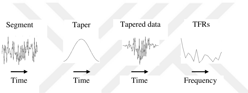
Figure 5: Temporally localized frequency decomposition: Diagram of the processing of a segment of the trial.
