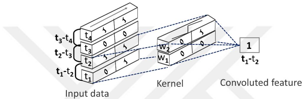
Figure 44: Illustration of the convolution operation for time series data. Input shape is (1,4,2) , i.e., one sample of four time points, each item having two channels. The kernel shape is (2,2) .
