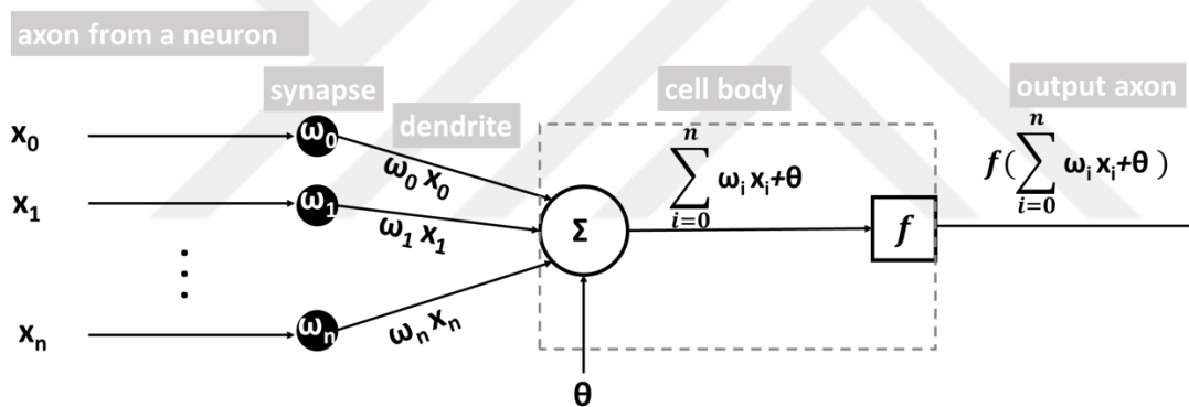
Figure 40: Biological inspiration for neural networks. Here x_i represents i th input, n represents the number of elements in neuron sets which is greater than zero. \omega_i represents the weights associated with the i th connection, \theta is the bias term. The output is computed by applying the activation function f to the weighted sum of the input signals. The gray background labels represent the parts of biological neurons corresponding to the related structure of the mathematical model presented below them.
