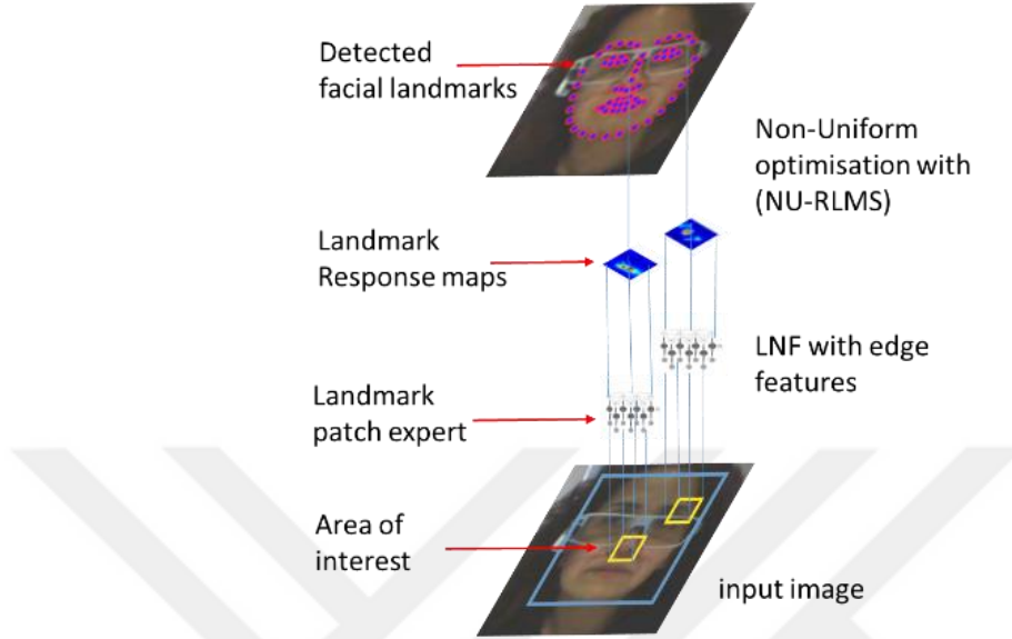
Figure 15: A demonstration of OpenFace methodology, adapted from Baltrušaitis et al. (2013). Here it is intentionally limited to two landmarks for illustrative purposes
