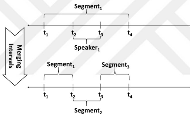
Figure 4: Merging intervals of segments and speakers
