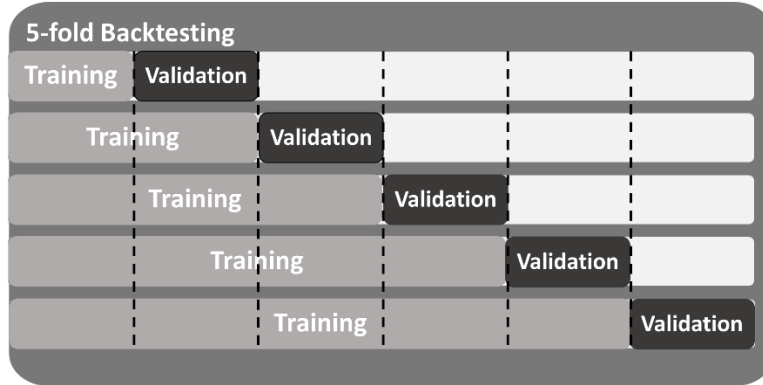
Figure 46: Illustration of 5-fold Backtesting.
