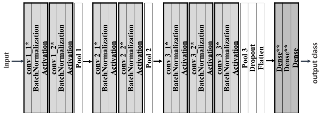
Figure 48: GazeVGG architecture with batch normalization, regularization and pooling. * L2 kernel and L2 bias regularizers were applied. **L2 kernel regularizer was applied.
