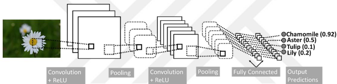
Figure 42: A simple CNN model. The output is one of the four flowering plants, image adapted from LeCun et al., 1998
