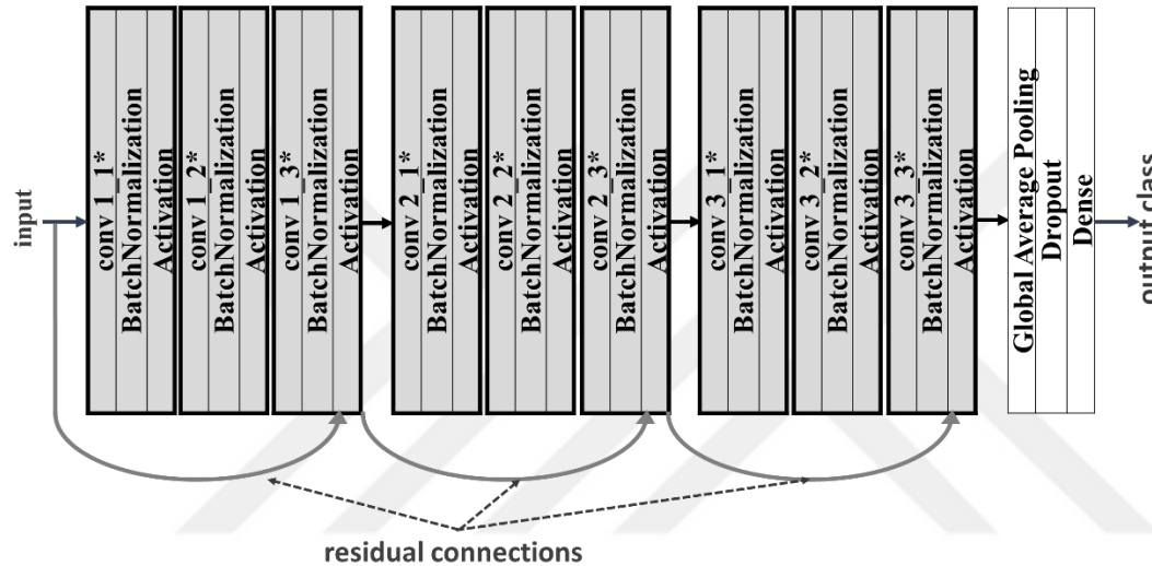
Figure 49: Simplified ResNet architecture with batch normalization, regularization, and pooling. There is a convolution between blocks and a residual connection between the last item of the previous block and the current one, which means the training in between layers is omitted. * L2 kernel and L2 bias regularizers are applied.
