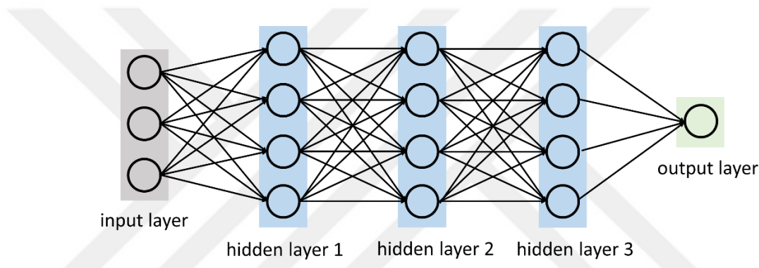
Figure 41: DNN structure with three hidden layers
