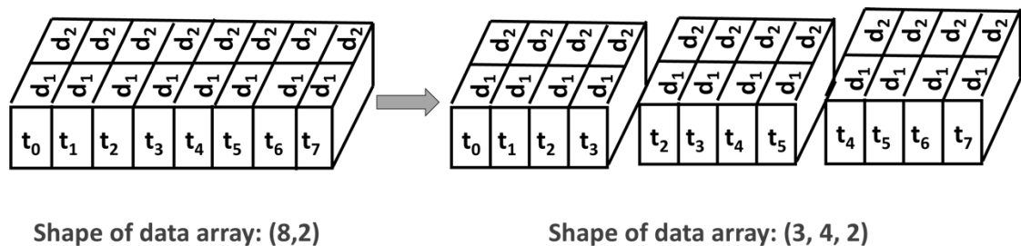
Figure 45: Shape of the time series array. On the left, the shape of data is (8,2) where the number of data points is eight and the number of dimensions is two. On the right-hand side, the shape has changed to (3,4,2) where the timestamp is four and the step distance is two.
