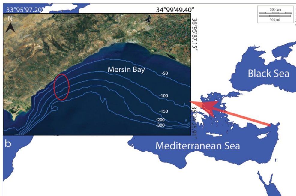
Figure 3 Sampling region
