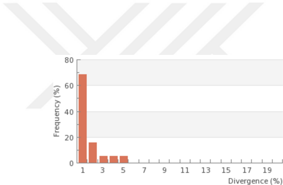
Figure 9 Histogram for mean intraspecific distances for the fish dataset.
