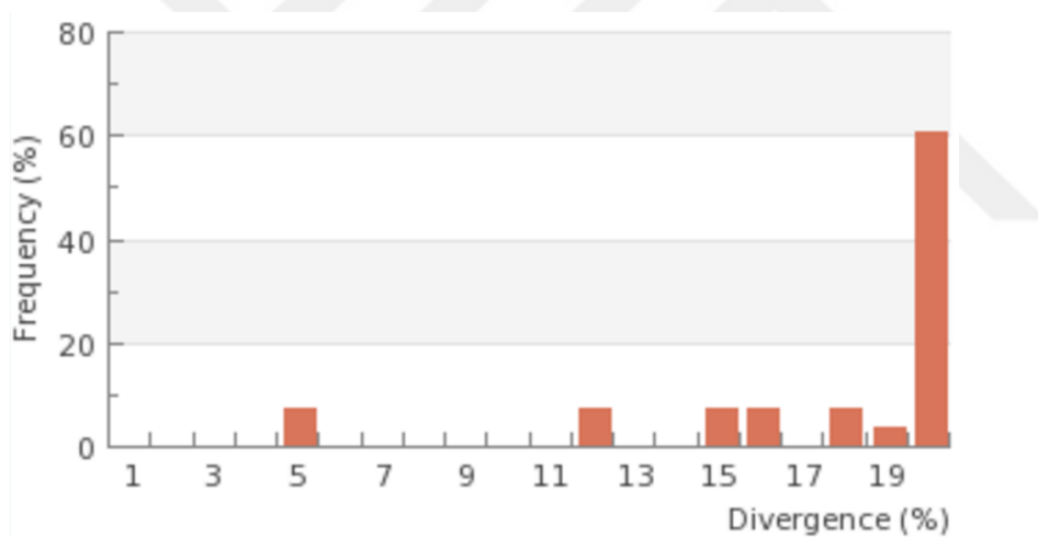
Figure 20 Histogram for distances to the nearest neighbors for the invertebrate and ascidian dataset.
