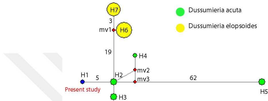
Figure 24 Network analysis for Dussumieria species including the barcode records in BOLD database together with the present study samples.
