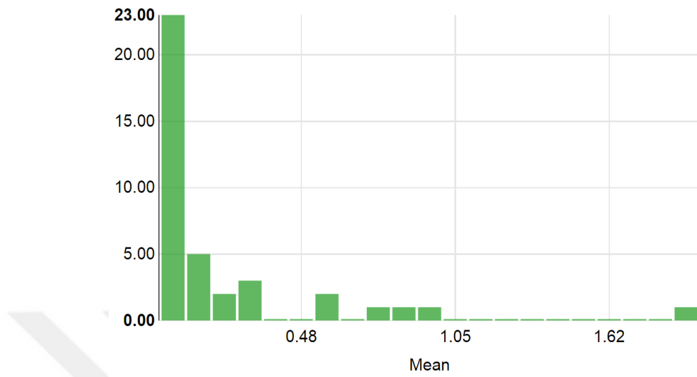
Figure 11 Histogram for mean within OTU distances for the fish dataset.
