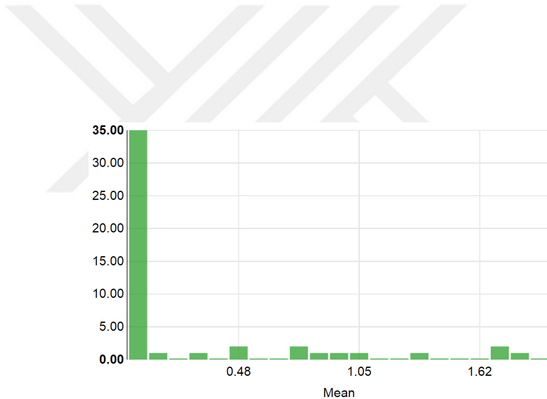
Figure 21 Histogram for mean within OTU distances for the invertebrate and ascidian dataset.
