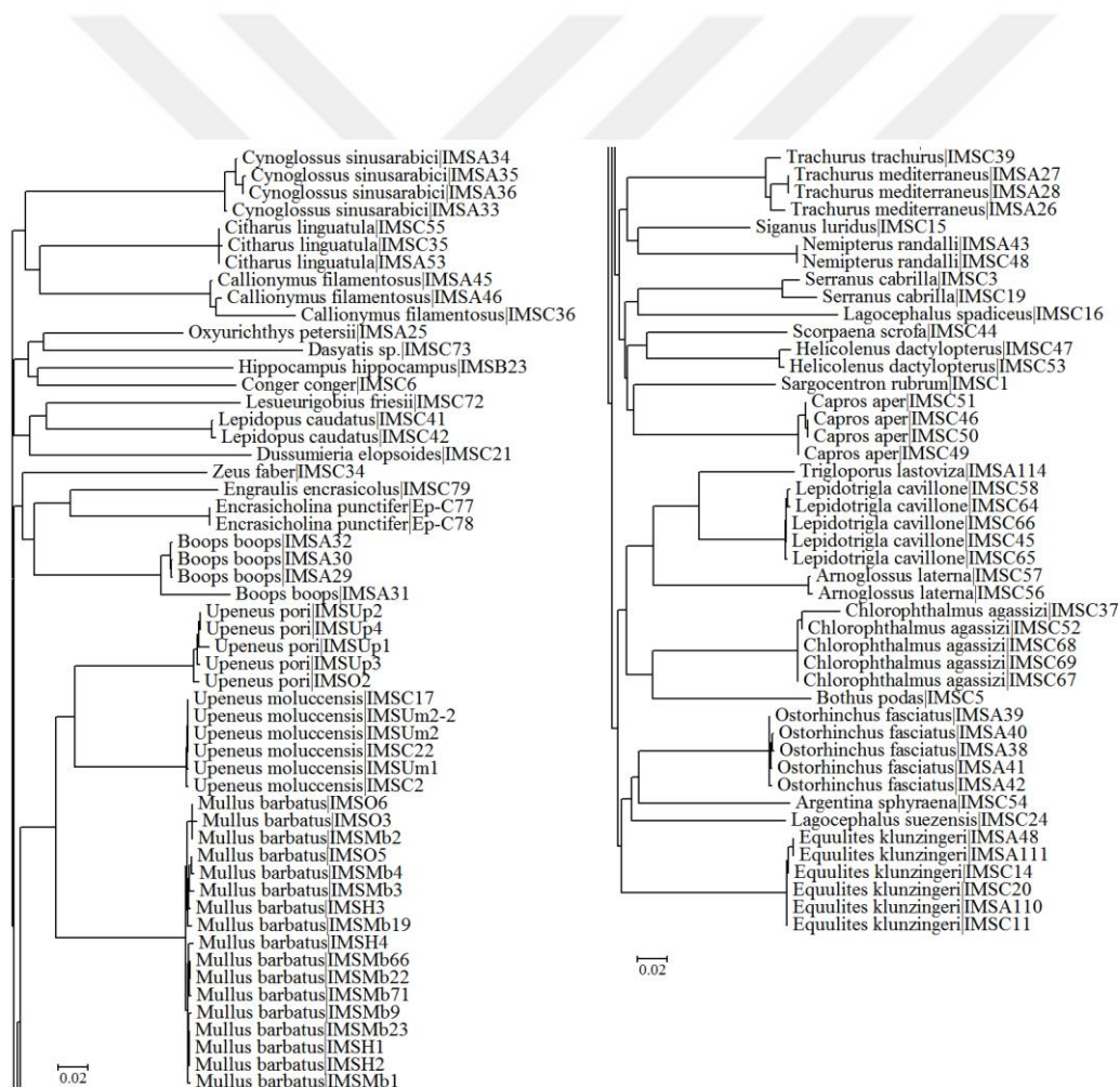
Figure 13 Neighbor joining tree including all haplotypes of 36 fish species from Mersin Bay given with sample ID's.
