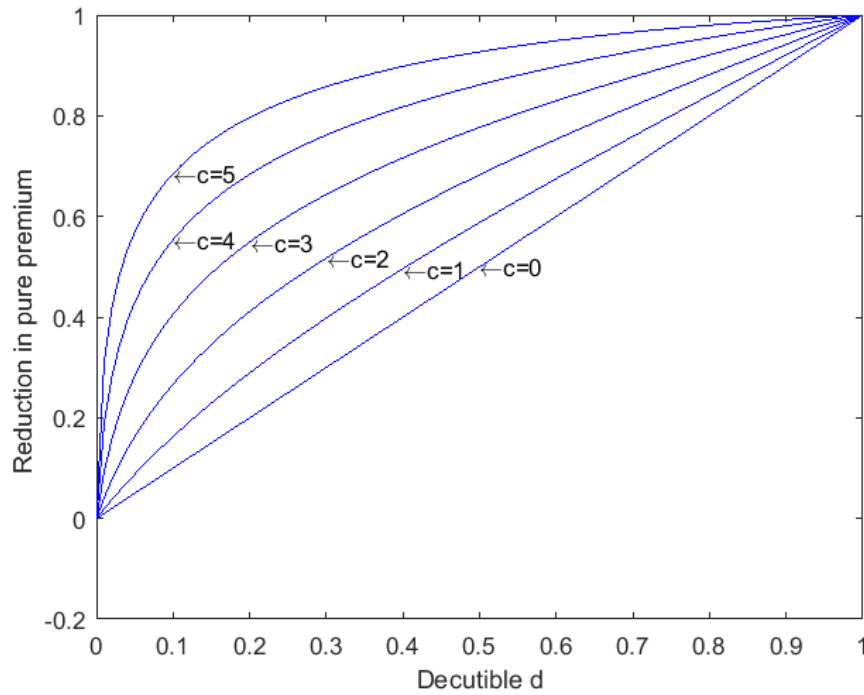
Figure 3.6: Exposure curves based MBBEFD distributions for c = 0, 1, 2, 3, 4, 5 .
