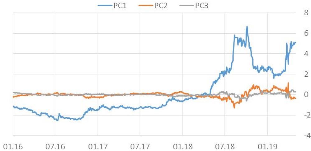
Figure 4.1: Principal Components
