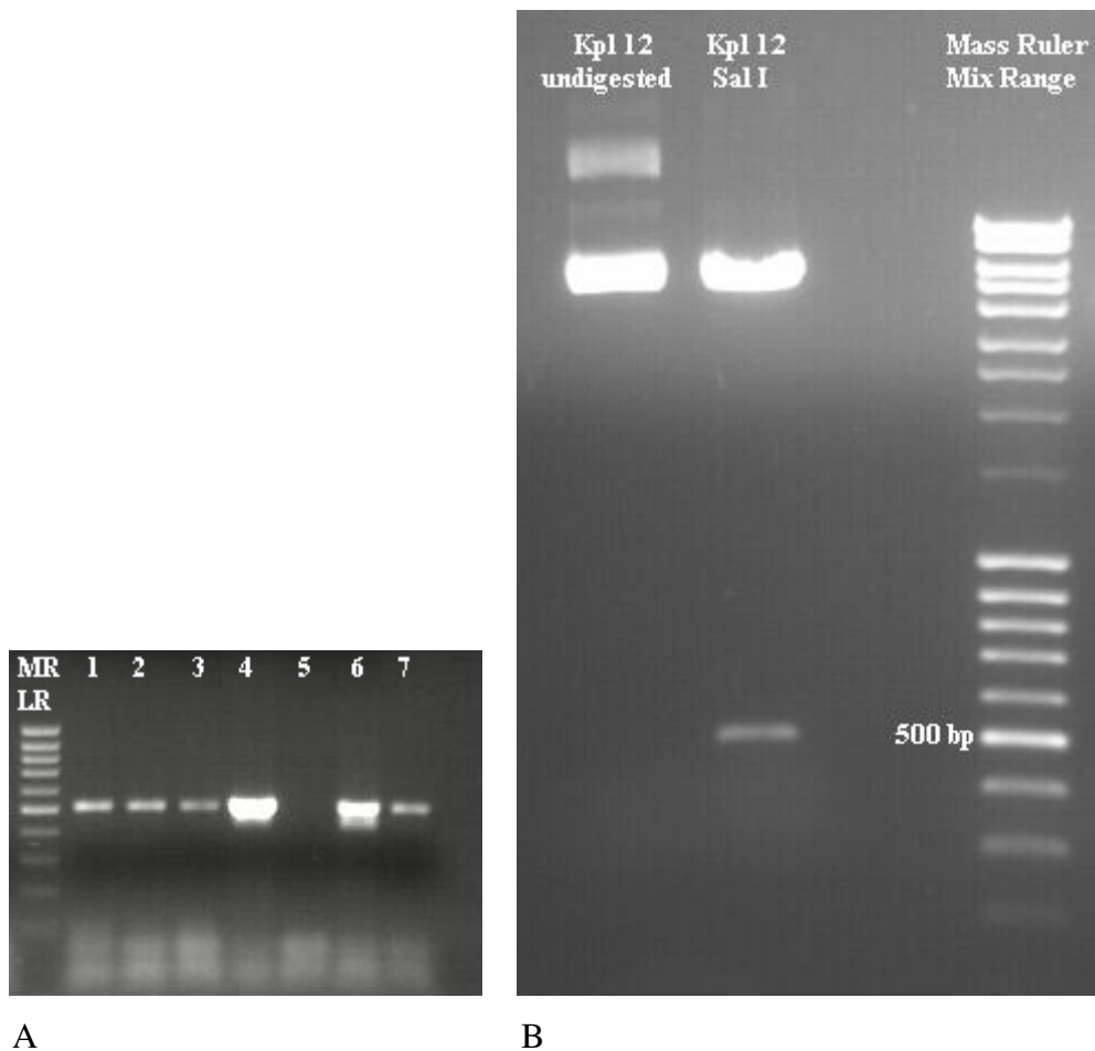
Figure 4.19: Colony PCR (A) and Sal I digestion (B) of pGL3fos-Kpl12 vector.
