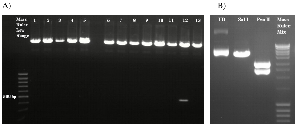
Figure 4.13: Colony screening and diagnostic digestions for Kpl7 insert A) Sal I digestion of plasmids isolated from colonies for screening Kpl7 insertion into pGL3fos. B) Analysis of Sal I and Pvu II digestions of constructed pGL3fos-Kpl7 vector. UD represents undigested plasmid.
