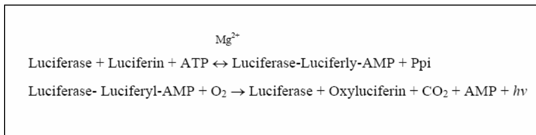
Figure 1.5: Reaction catalyzed by firefly luciferase.
