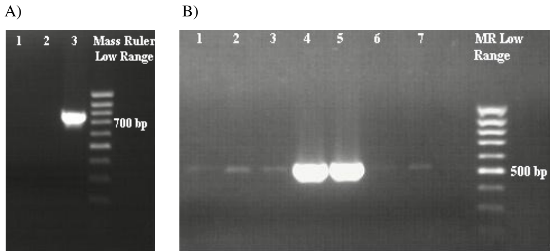
Figure 4.17: Analysis of colony PCR results for Kpl11 (A) and Kpl13 (B) insertions into pGL3fos vector.
