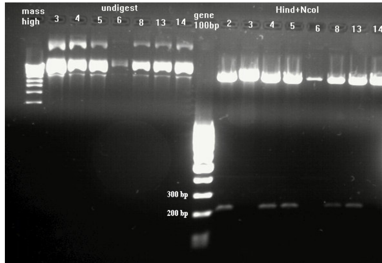
Figure 4.10: Analysis of Hind III-Nco I double digest of isolated plasmids. The 211 bp fragment contains fos promoter that is cut out from pGL3fos vector.
