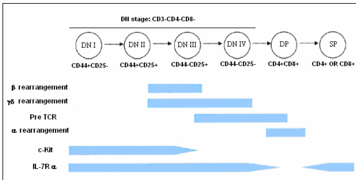
Figure 1.4: Developmental stages and IL-7R \alpha expression of T-lymphocytes (adapted from Fry and Mackall, 2002).
