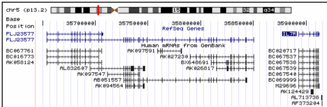
Figure 4.3: Human IL-7R gene and upstream region including Kpl2 homologous gene FLJ23577.
