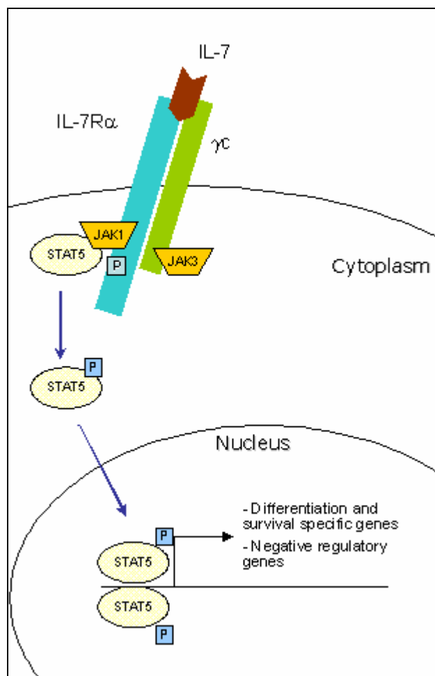
Figure 1.2: General representation of interleukin-7 activated signal transduction pathway (adapted from Kang and Der, 2004).
