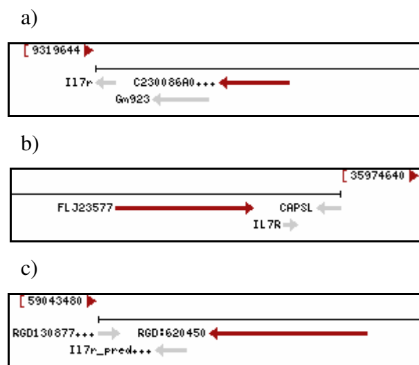
Figure 4.1: Genomic locations of IL-7R and upstream neighbouring genes or gene predictions. C230086A09 and Gm923 on mouse chromosome-15 (a), FLJ23577 on human chromosome-5 (b) and RGD:620450 (Kpl2) on rat chromosome-2 (c) are all homologous to Kpl2 gene.
