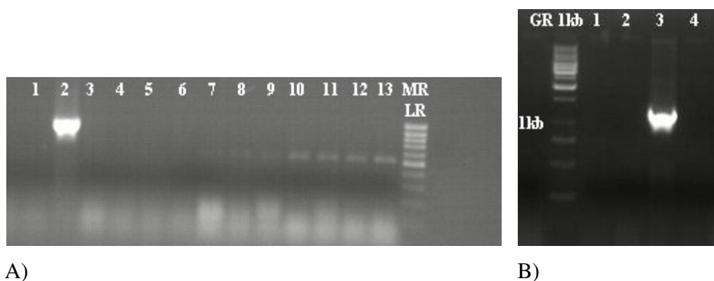
Figure 4.15: Colony PCR results for screening Kpl9 (A) and Kpl10 (B) insertions into pGL3fos. Mass Ruler Low Range and Gene Ruler 1kb molecular weight markers are used respectively.
