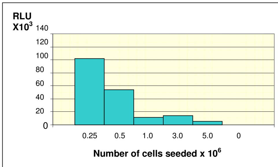
Figure 4.26: Luciferase activity of 293T cells transfected with pGL3 Control vector at different cell densities. X-axis shows the number of cells seeded 24 hours prior to transfection.
