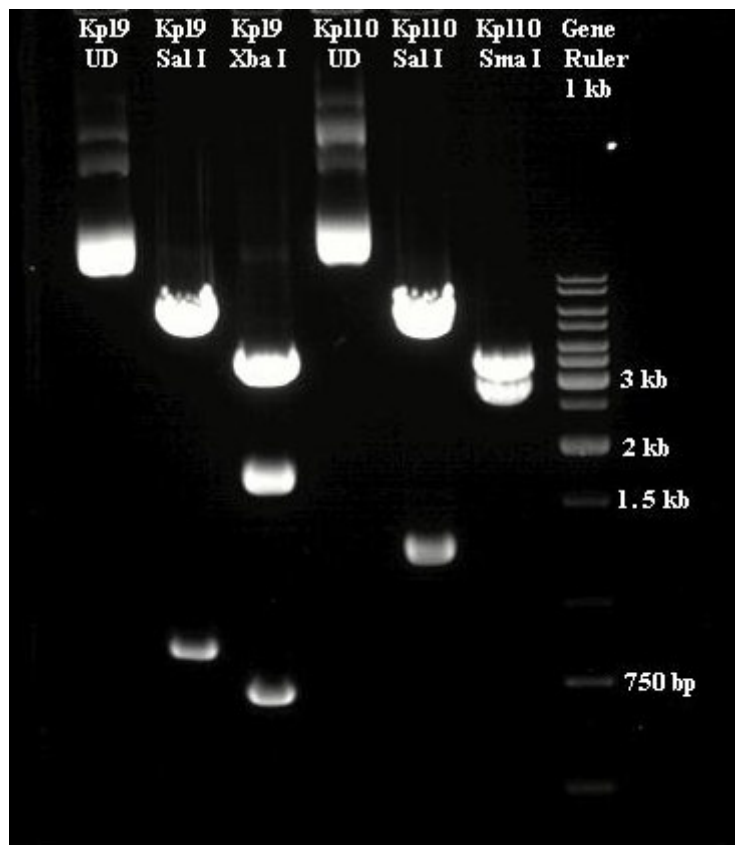
Figure 4.16: Restriction enzyme digestion analysis of pGL3fos-Kpl9 and pGL3fos-Kpl10 vectors.
