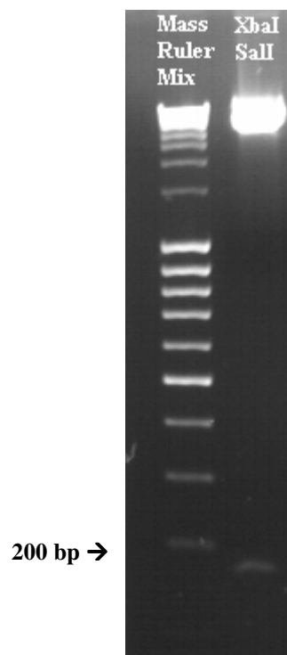
Figure 4.8: Xba I-Sal I double digestion of \Delta 56\text{fosCAT} plasmid.
