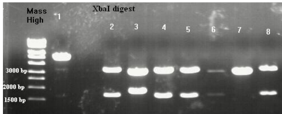
Figure 4.12: Analysis of Xba I digests of isolated plasmids.
