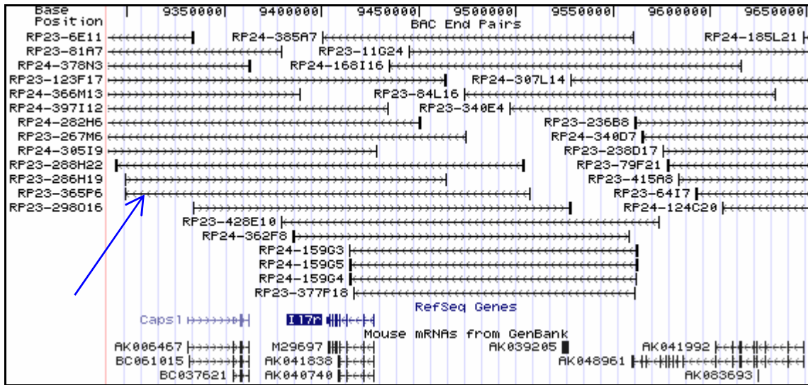
Figure 4.6: Mouse RP23-365P6 BAC clone (indicated with arrow) covers IL-7R gene and its 40 Kb upstream region.
