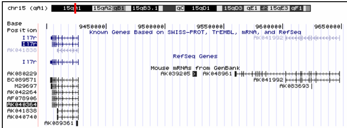
Figure 4.2: Mouse IL-7R gene and upstream region including Kpl2 homologous gene AK041992 and its variant mRNA AK048961.
