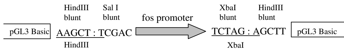
Figure 4.9: Blunt end ligation of fos promoter and pGL3 Basic vector. Hind III and Xba I sites are created on the construct vector are underlined.
