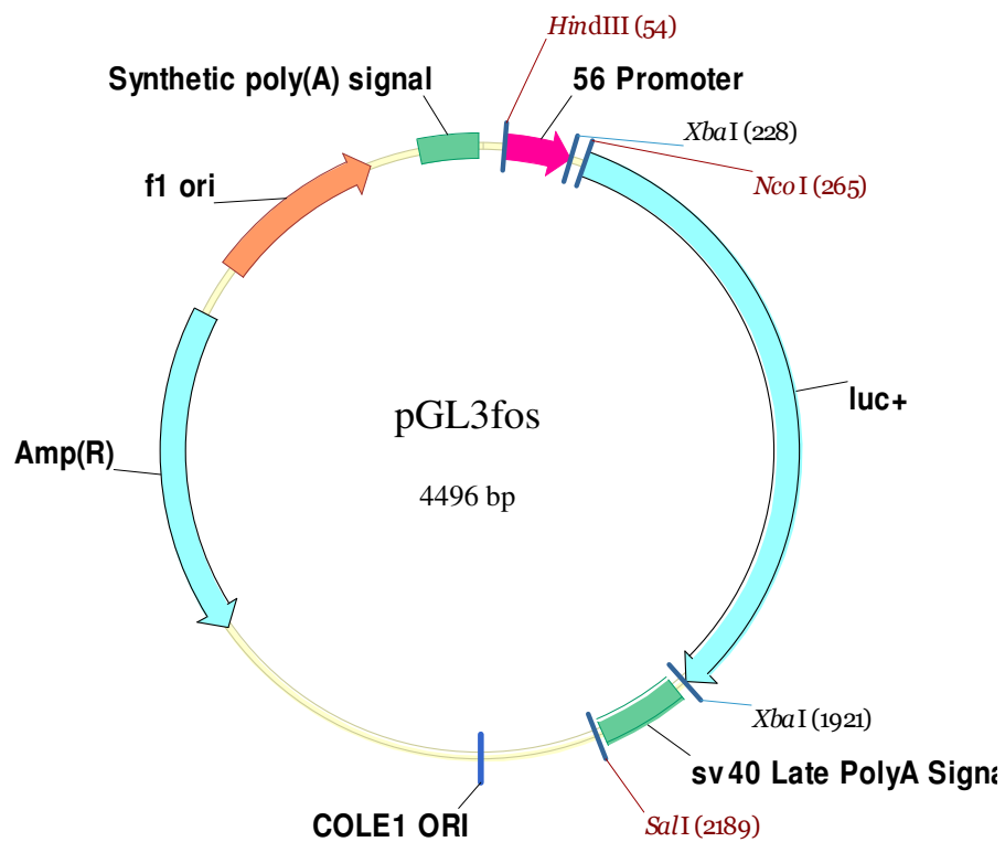
Figure 4.10: Analysis of Hind III-Nco I double digest of isolated plasmids. The 211 bp fragment contains fos promoter that is cut out from pGL3fos vector.
