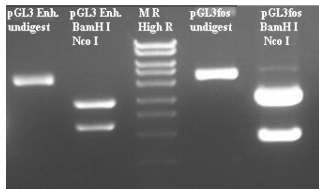
Figure 4.22: BamH I-Nco I double digestion for pGL3 Enhancer and pGL3fos vectors. Mass Ruler High Range was used as molecular weight marker.
