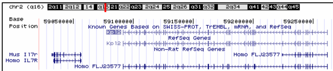
Figure 4.4: Rat genomic region corresponding to mouse and human IL-7R genes and upstream region including Kpl2 gene.
