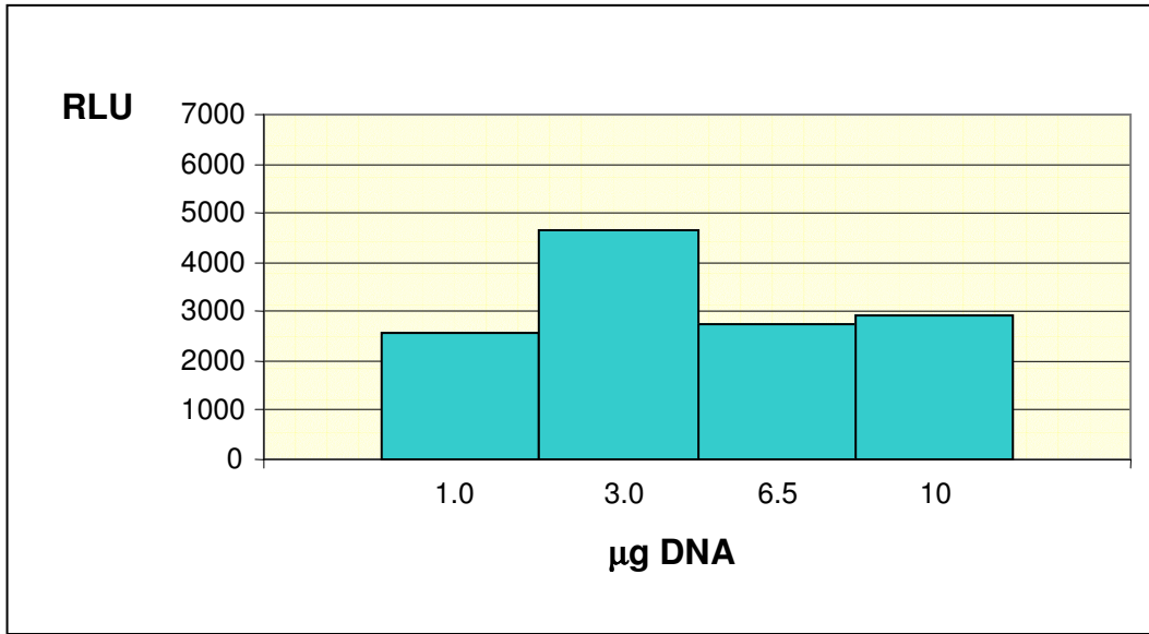
Figure 4.25: Luciferase activity of 293T cells transfected with different amounts of pGL3 Control vector.
