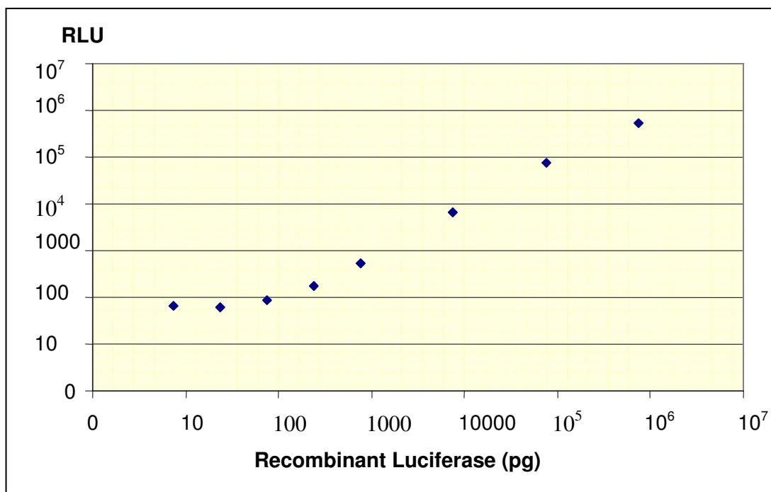
Figure 4.24: Standard curve for determination of linear range of luminescence detection. Note that values were plotted logarithmically.
