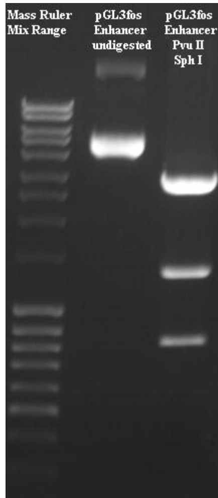
Figure 4.23: Analysis of Pvu II-Sph I double digestion of pGL3fos Enhancer vector.
