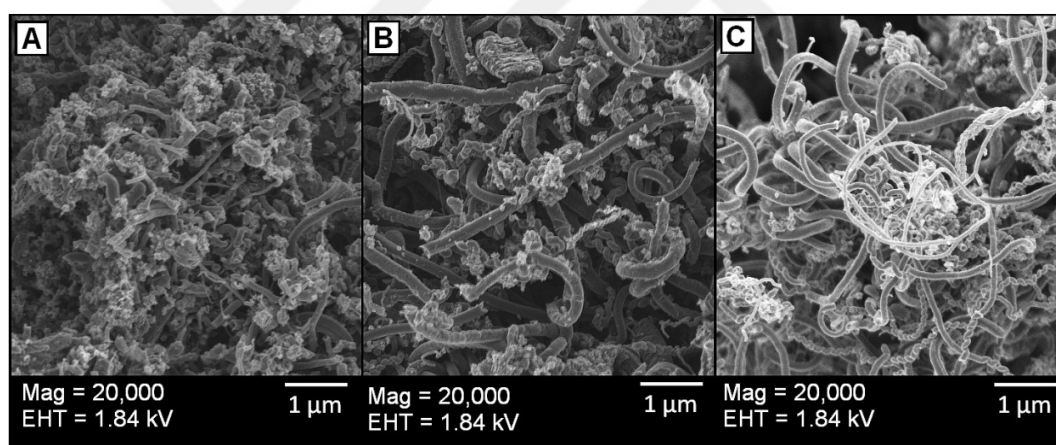
Figure 5-45 SEM micrographs of CNFs A) As received after CVD (CVD conditions; Ni tartrate/NaCl catalyst, acetylene/Ar gas mixture (80:20), at 500°C , flow rate of acetylene 3L/min) B) Water treated and C) Acid treated
