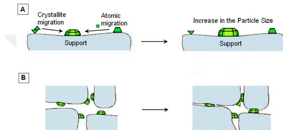
Figure 5-17 Catalyst deactivation mechanisms: A) Sintering of the active metal particles and B) Sintering and solid-solid phase transitions of the support and encapsulation of active metal particles. Adapted from Ref [322]
