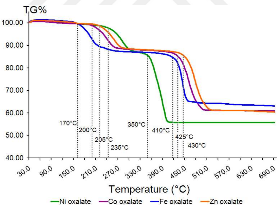
Figure 5-6 TGA thermogram of oxalate based catalysts
