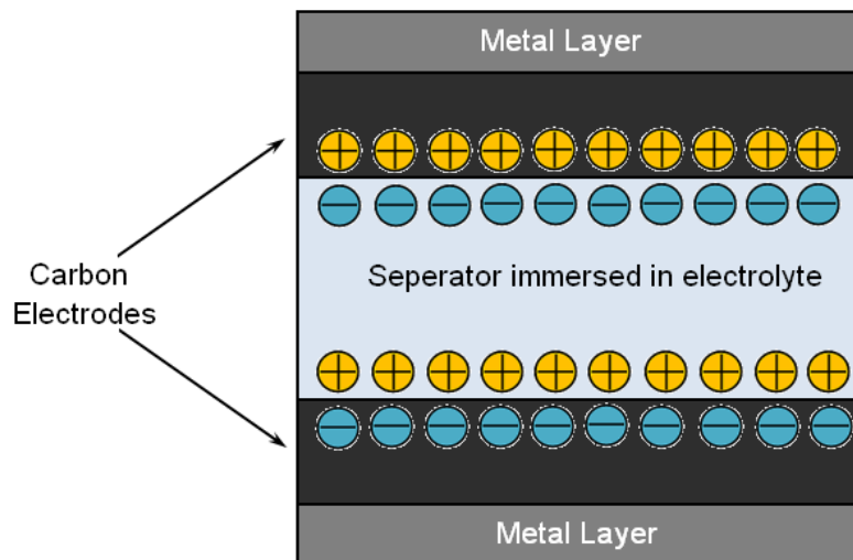
Figure 2-23 A double layer supercapacitor
