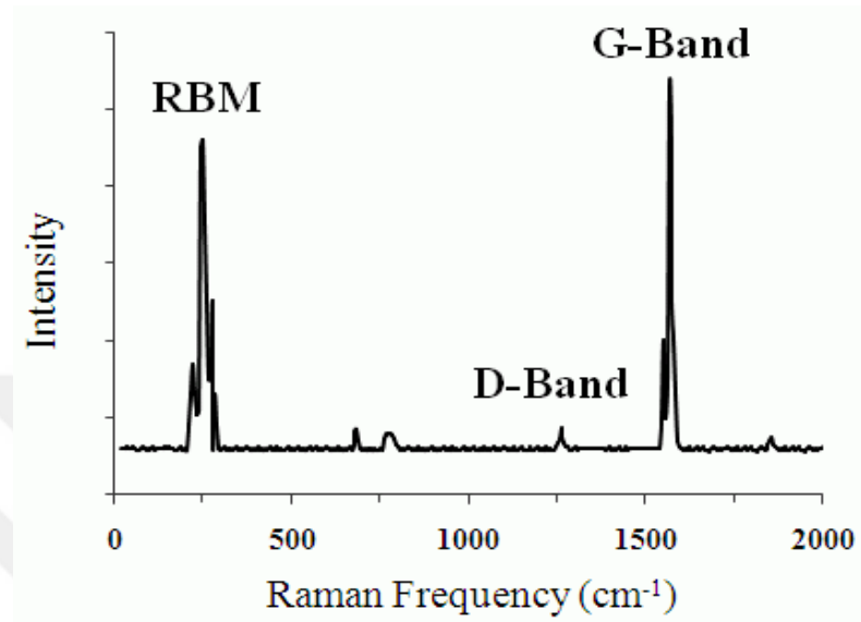
Figure 2-19 Illustration of Raman spectra of a SWNT. RBM, G and D Band characteristic peaks are seen.
