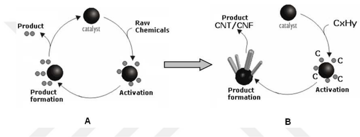
Figure 2-13 A. Classical catalytic cycle B. Catalytic route for Carbon material formation using CVD process.
