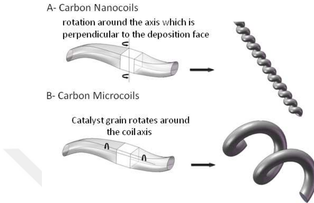
Figure 5-23 Formation of A) carbon nanocoils and B) carbon microcoils
