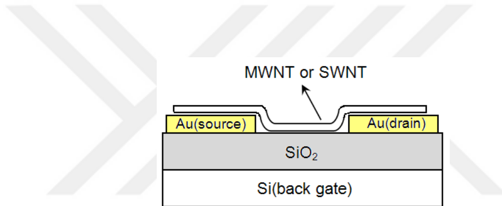
Figure 2-26 Schematic cross-section of a FET device.
