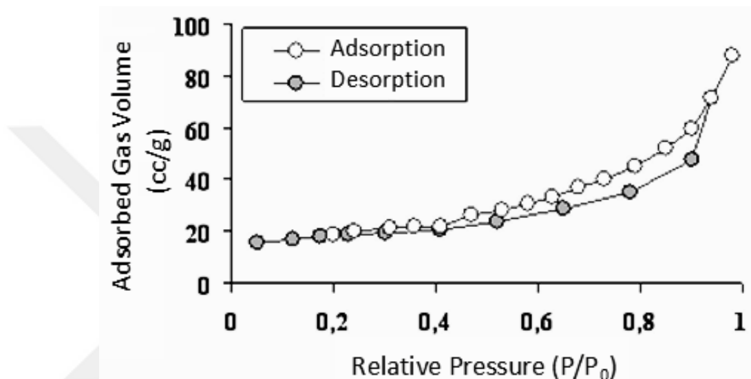
Figure 5-10 N 2 adsorption/desorption isotherm of Cobalt tartrate/NaCl catalyst (surface area = 140 m 2 /g)
