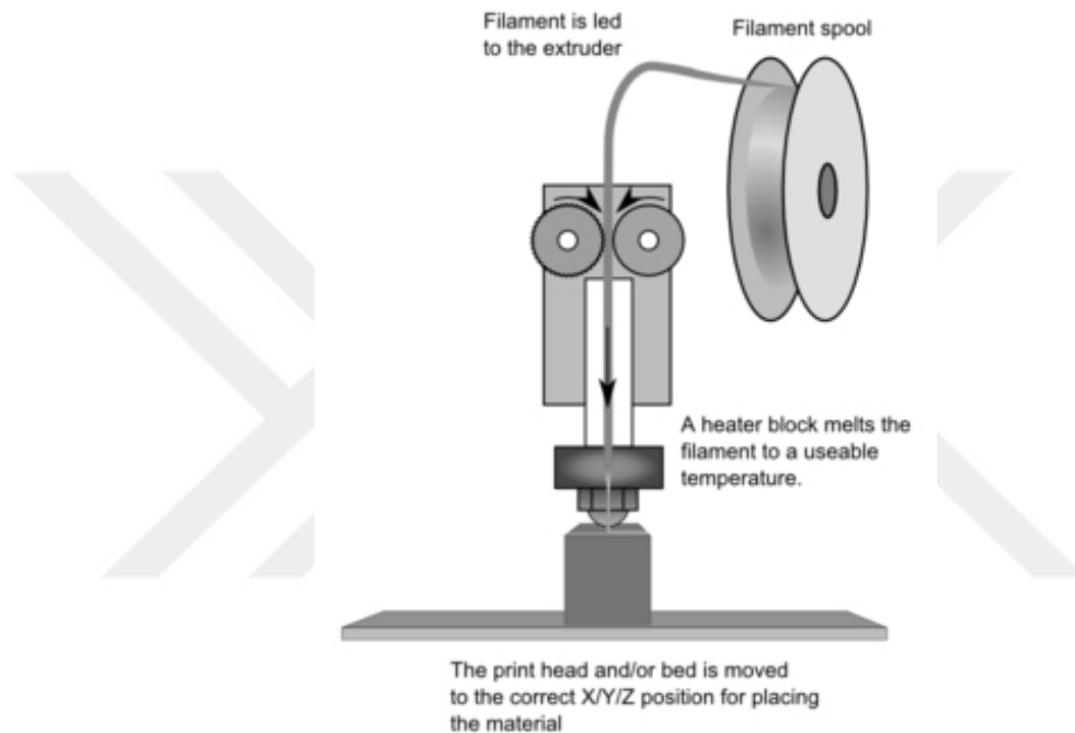
Figure 4.1: Working principle of FDM printers
