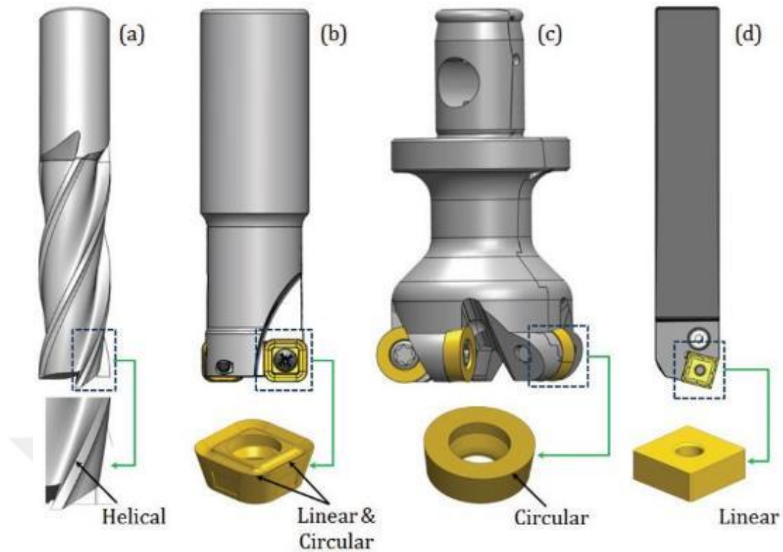
Figure 2-8 Cutting edges for: a) End mill tool. b) Indexable end mill. c) Face mill. d) Turning tool.
