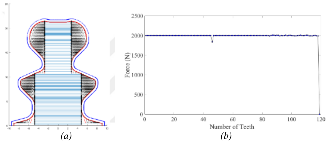
Figure 4-10 Rake and inclination angle is set to zero a) teeth shape b) tangential cutting force on each tooth.
