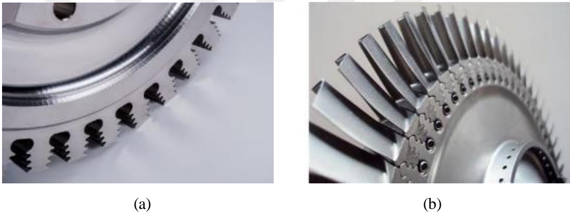
Figure 1-7. (a) Fir-tree slots on turbine disk (b) Turbine disk joints with blades.
