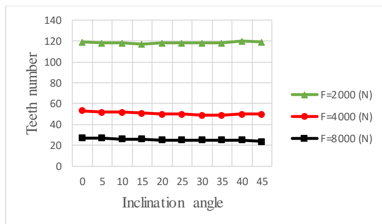
Figure 4-16 Inclination angle vs Teeth number.
