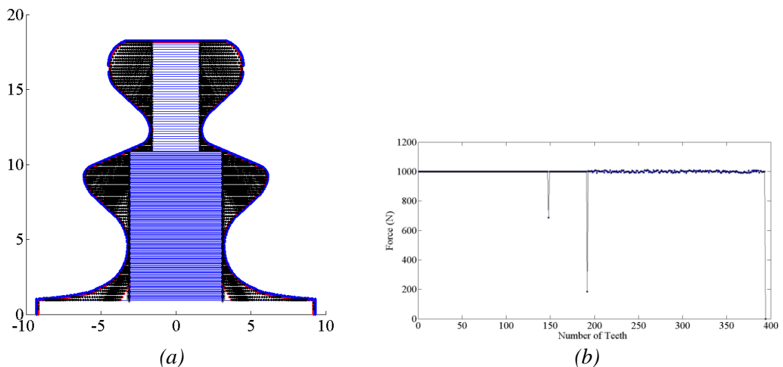
Figure 5-2 Simulation with developed algorithm. Limiting force at roughing and semi-finishing is set to 1000 N. rake and inclination angle is set to zero and approach angle is 25^\circ a) teeth shape b) tangential cutting force on each tooth.
