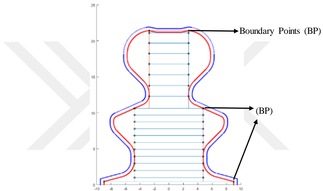
Figure 3-8 Boundary points on generated finishing curve with generated roughing teeth.
