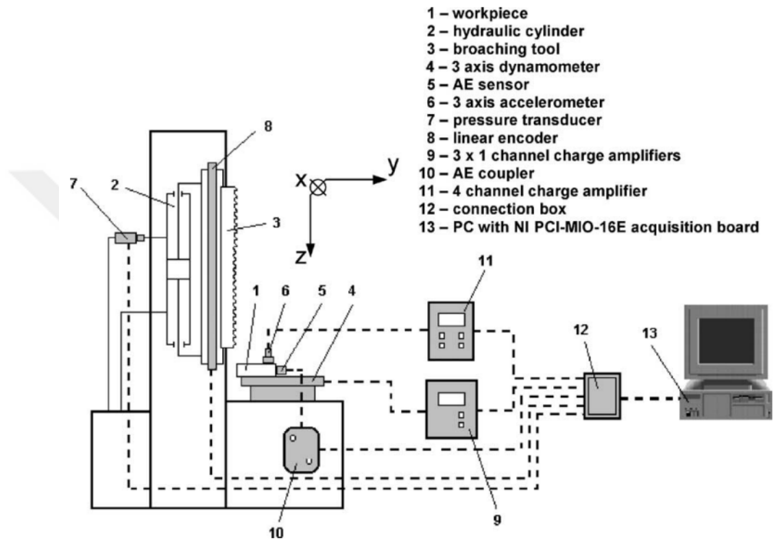
Figure 1-3. Schematic diagram of the monitoring system [7].
