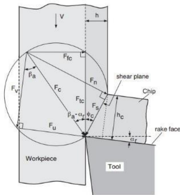
Cutting force diagram
