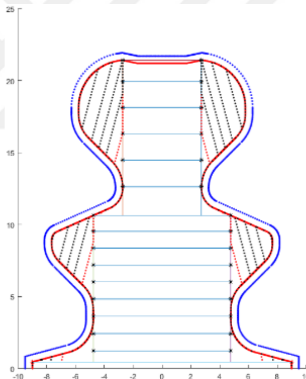
Figure 4-3 Broaching teeth simulation: Limiting cutting force in roughing and semi-finishing is selected as 10,000 N, rake and inclination angle is set to zero, approach angle is 15^\circ .
