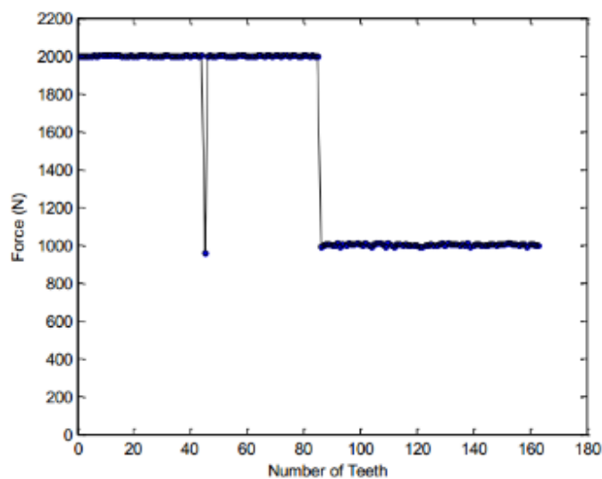
Figure 1-6 Constant cutting forces in roughing and semi-finishing step.
