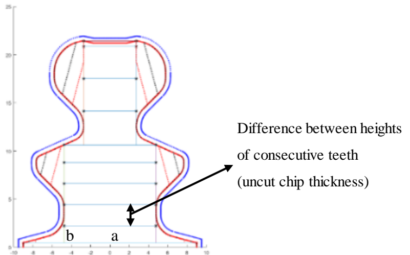
Figure 3-10 First teeth dimensions and uncut chip thickness at roughing step.
