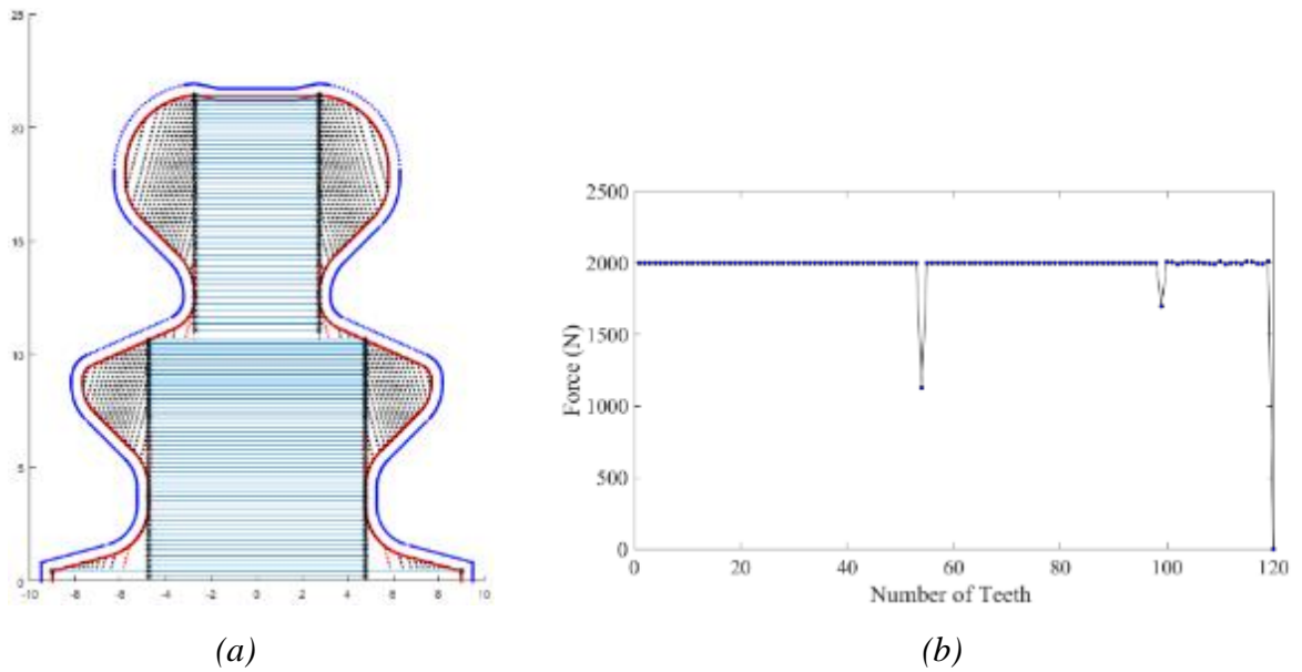
Figure 4-15 Inclination angle is 30^\circ and Rake angle is zero: a)teeth shape b)tangential cutting force on each tooth.
