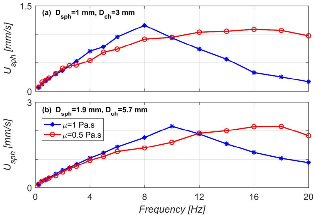
Figure 3.10 Swimmer velocity vs. magnetic field rotation frequency plotted for the silicone oil viscosities of \mu = 1 \text{ Pa.s} and \mu = 0.5 \text{ Pa.s} for the configurations a) D_{sph} = 1 \text{ mm}, D_{ch} = 3 \text{ mm} , and b) D_{sph} = 1.9 \text{ mm}, D_{ch} = 5.7 \text{ mm} where D_{ch}/D_{sph} ratio is 3
