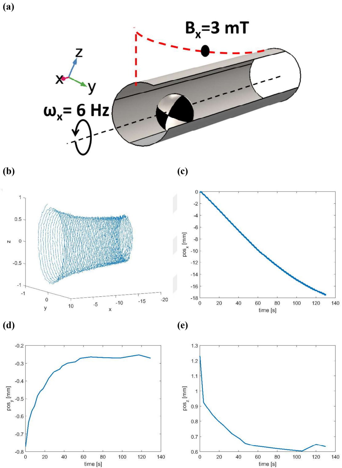
Figure 3.20 Visualization of the rotation of the sphere about x-axis under a magnetic field rotation frequency 6 Hz, following a helical trajectory under magnetic field along x-axis applied at 3mT from the wake of the sphere only. A decay in the radius of the helical trajectory is observed as the sphere migrates towards the center of the cylindrical channel. The sphere does not settle into a circular trajectory at the end of the workspace where the magnetic field applied in x-direction is still effective due to the greater magnitude applied.
