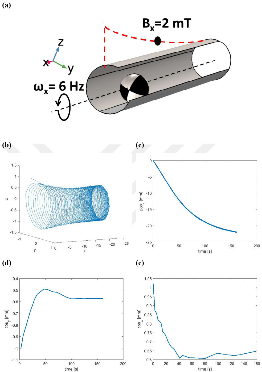
Figure 3.19 Visualization of the rotation of the sphere about x-axis under a magnetic field rotation frequency 6 Hz, following a helical trajectory under magnetic field along x-axis applied at 2 mT from the wake of the sphere only. A decay in the radius of the helical trajectory is observed as the sphere migrates towards the center of the cylindrical channel.
