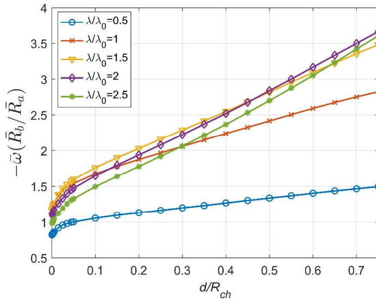
Figure 2.31 Velocity profile with respect to the changing thickness (screw type swimmer), obtained using the resistance coefficients.
