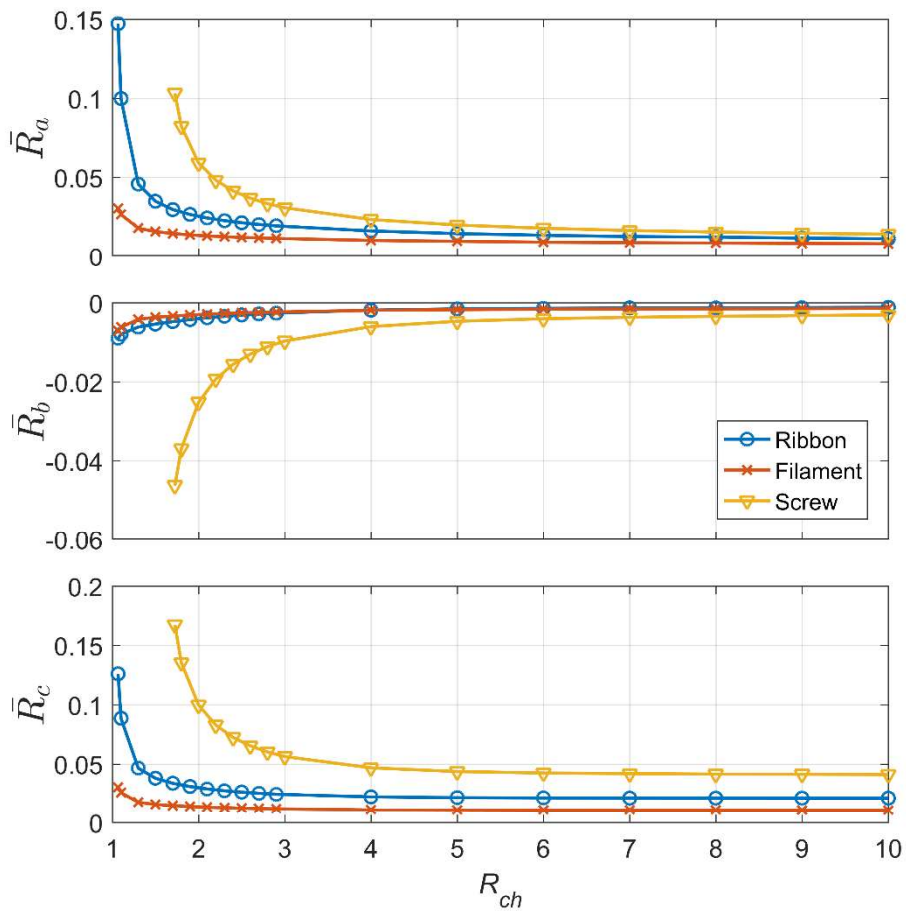
Figure 2.23 Translational, translation-rotation coupling, and rotational resistance coefficients plotted against channel diameter R_{ch} .
