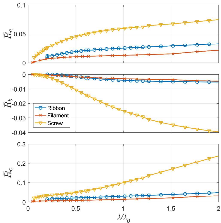
Figure 2.20 Translational, translation-rotation coupling, and rotational resistance coefficients plotted against the normalized wavelength \lambda/\lambda_0 .
