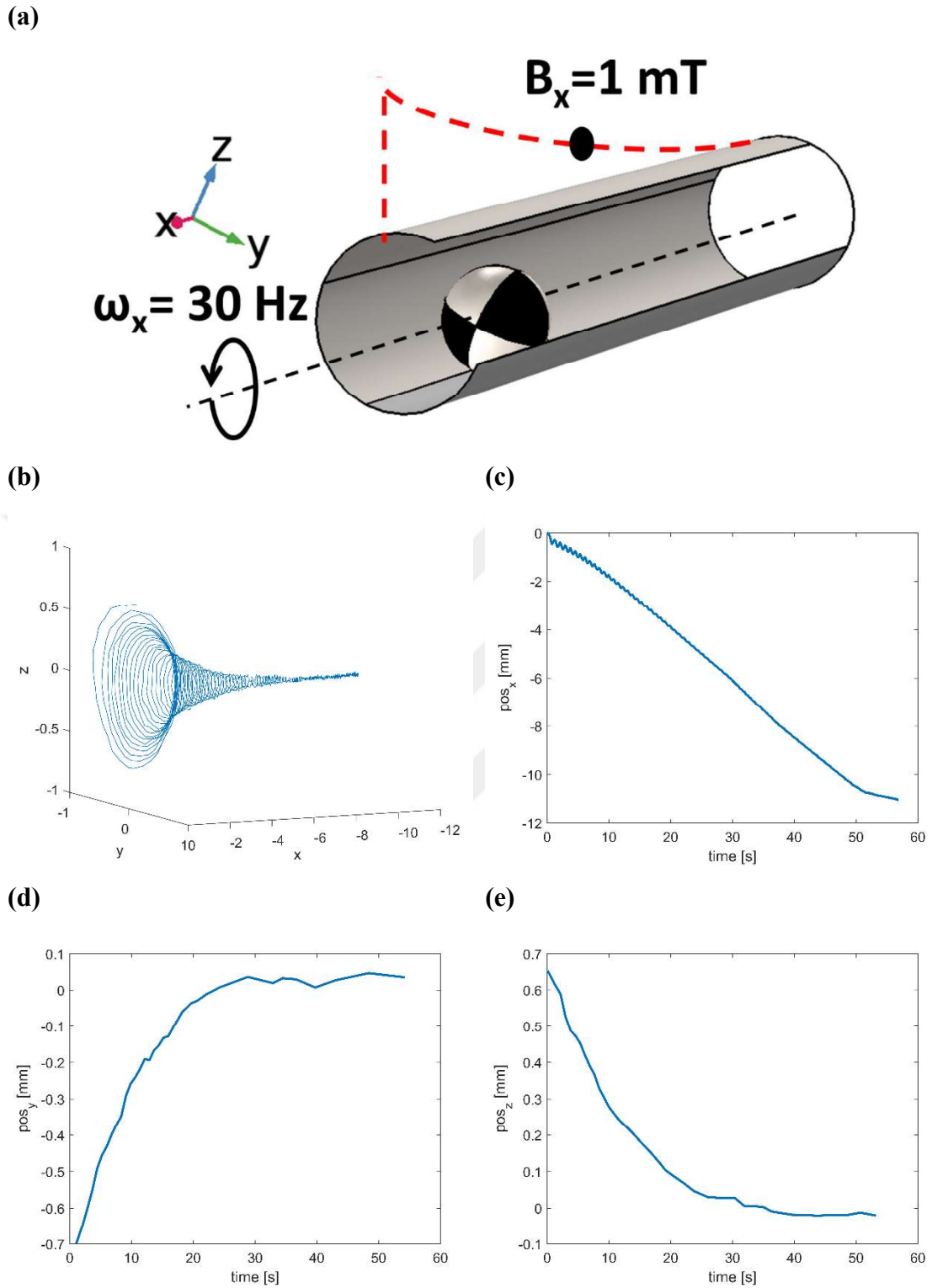
Figure 3.23 Visualization of the rotation of the sphere about x-axis under a magnetic field rotation frequency 30 Hz, following a helical trajectory under magnetic field along x-axis applied at 1 mT from the wake of the sphere only. Radius of the helical trajectory quickly converges to zero as the sphere settles down onto the central axis of the cylindrical channel.
