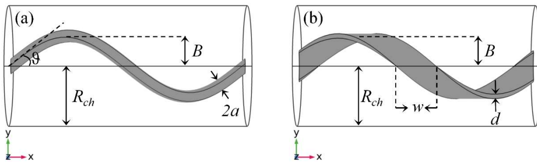
Figure 2.1 (a) Right-handed helical rod with a circular cross-section of diameter 2a ; (b) Helical ribbon with thickness d and width w .
