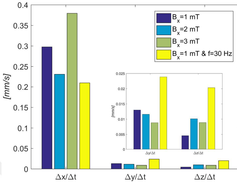
Figure 3.21 Velocities obtained by the sphere following a helical trajectory under different magnetic field gradients along x-axis.
