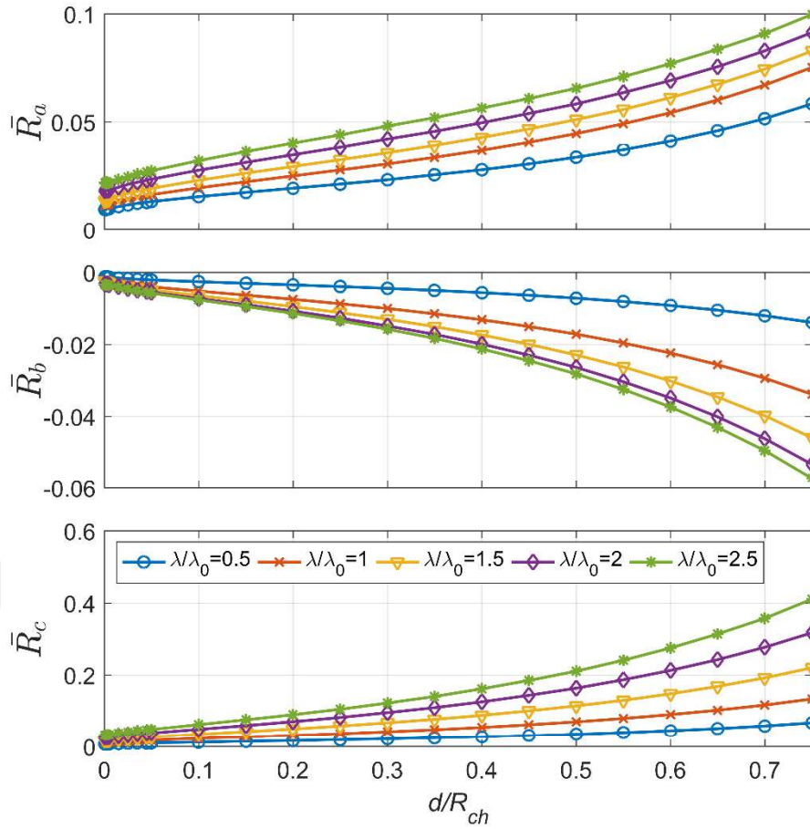
Figure 2.30 Translational, translation-rotation coupling, and rotational resistance coefficients plotted against normalized thickness d/R_{ch} for various wavelengths of the screw type swimmer.
