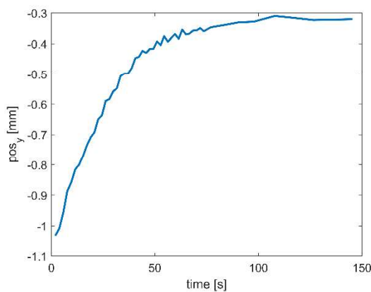
Figure 3.18 Visualization of the rotation of the sphere about x-axis under a magnetic field rotation frequency 6 Hz, following a helical trajectory under magnetic field along x-axis applied at 1 mT from the wake of the sphere only. Following the decay in the radius of the helical trajectory, the sphere starts to follow a circular path once the distance from the coil applying magnetic field in x-direction is sufficiently great.
