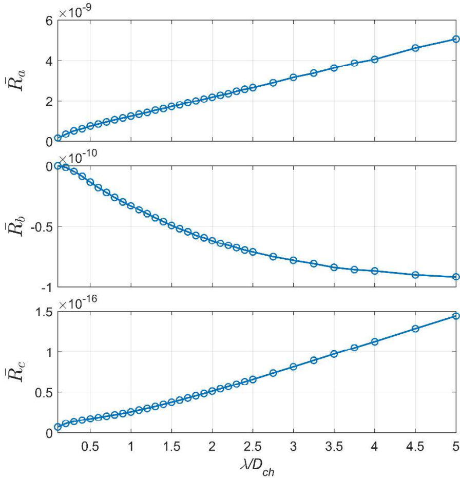
Figure 2.7 Translational, translation-rotation coupling, and rotational resistance coefficients plotted against normalized wavelength \lambda/D_{ch} .
