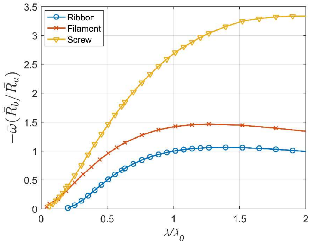
Figure 2.21 Velocity profile with respect to the changing wavelength, obtained using the resistance coefficients.
