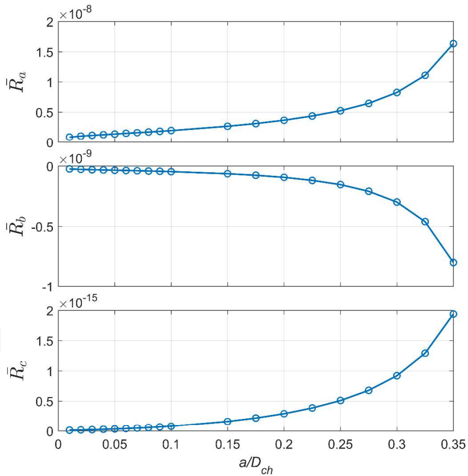
Figure 2.10 Translational, translation-rotation coupling, and rotational resistance coefficients plotted against normalized rod thickness a/D_{ch} .
