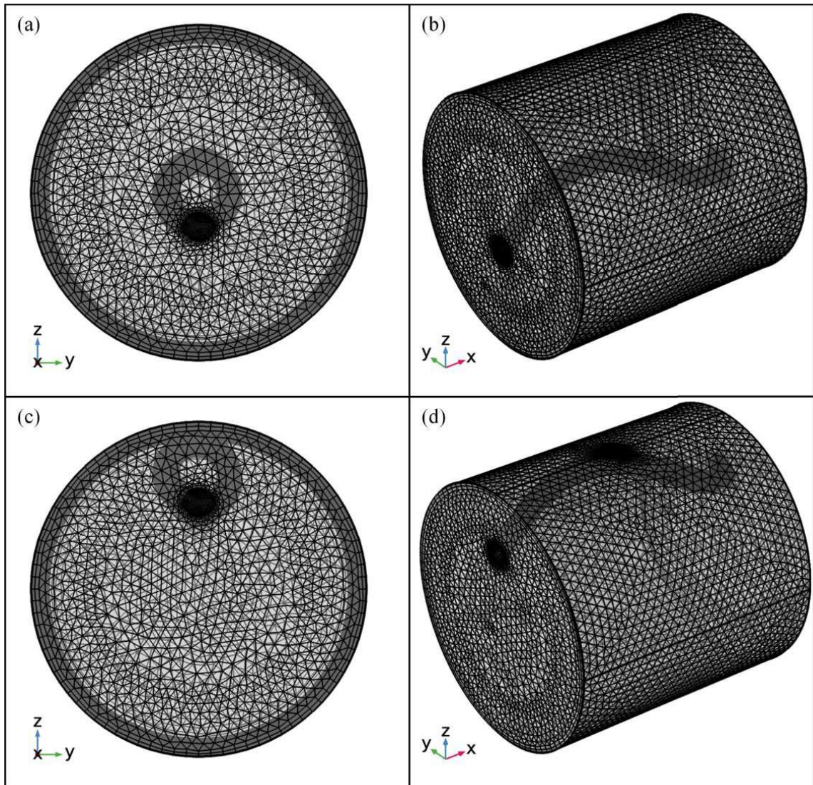
Figure 2.2 Finite-element meshes for the reference case (a) and (b); mesh refinement at the surface for the eccentric swimmer (c) and (d).
