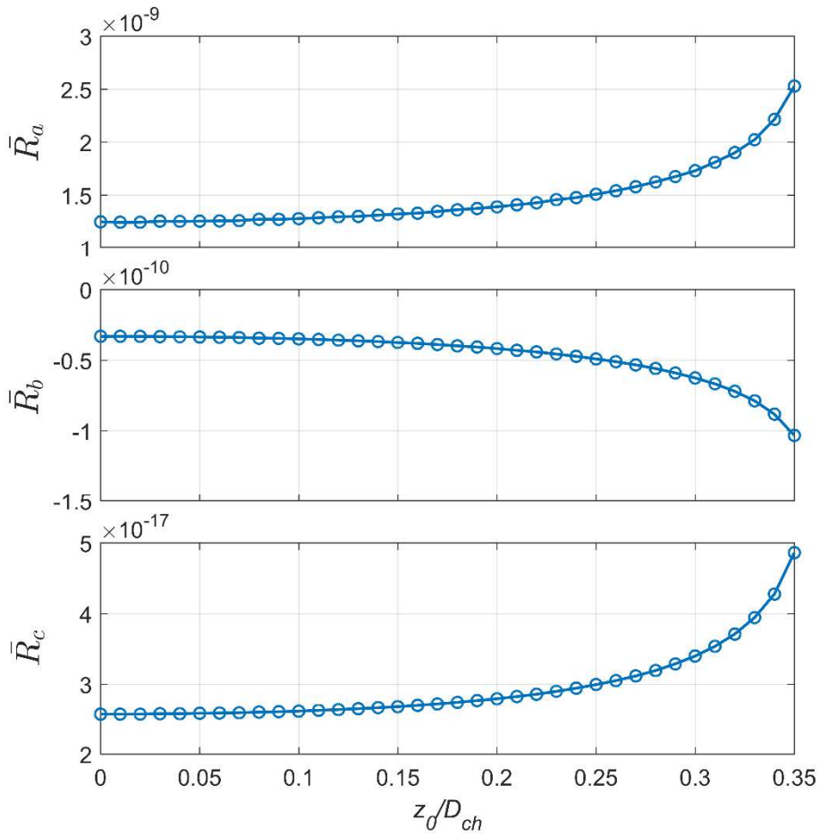
Figure 2.16 Translational, translation-rotation coupling, and rotational resistance coefficients plotted against normalized eccentricity z_0/D_{ch} .
