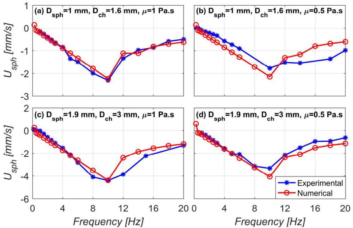
Figure 3.25 Comparison of the experimental results to the numerical predictions for D_{ch}/D_{sph} = 1.6 for two different silicone oil viscosities of \mu = 1\text{ Pa.s} and \mu = 0.5\text{ Pa.s} .
