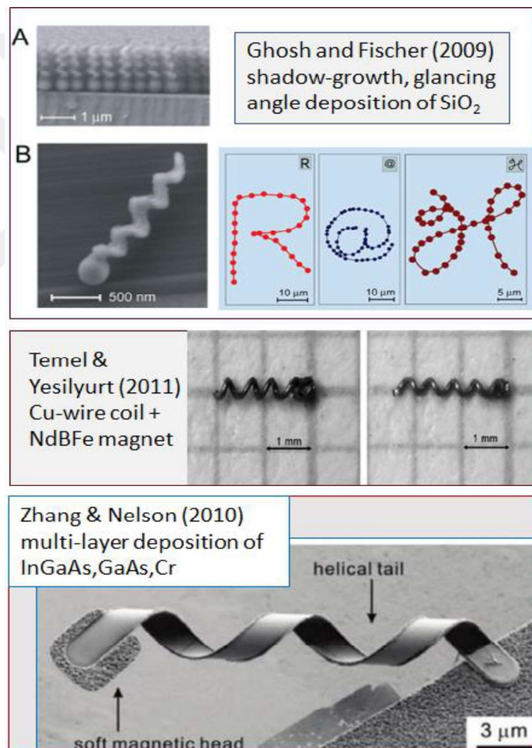
Figure 1.4 Various artificial helical micro swimmers. Ghosh and Fisher [19] presented the use of glancing angle deposition method to produce helical swimmers and demonstrated their accurate control, Temel and Yesilyurt [30] created swimmers with Cu wire and permanent magnets and magnetically actuated them, Zhang and Nelson [31] manufactured helical ribbon by multilayer deposition.
