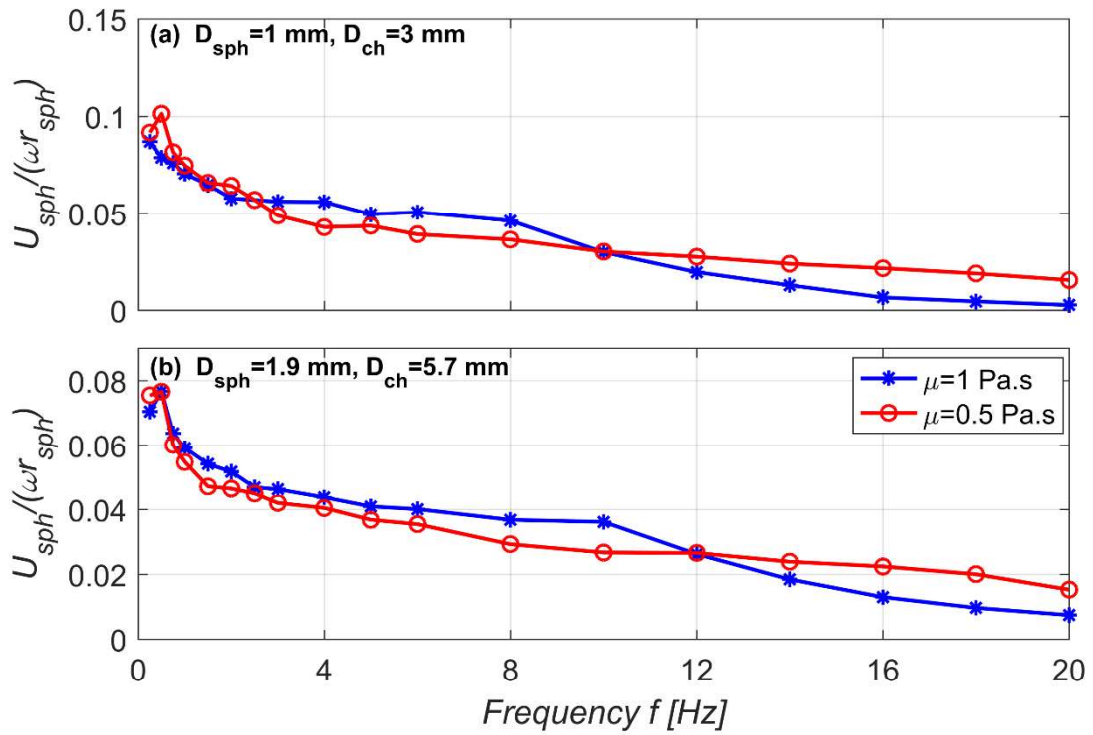
Figure 3.11 Swimmer velocity normalized with contact rolling velocity vs. magnetic field rotation frequency plotted for the silicone oil viscosities of \mu = 1 Pa.s and \mu = 0.5 Pa.s for the configurations a) D_{sph} = 1 mm, D_{ch} = 3 mm, and b) D_{sph} = 1.9 mm, D_{ch} = 5.7 mm where D_{ch}/D_{sph} ratio is 3
