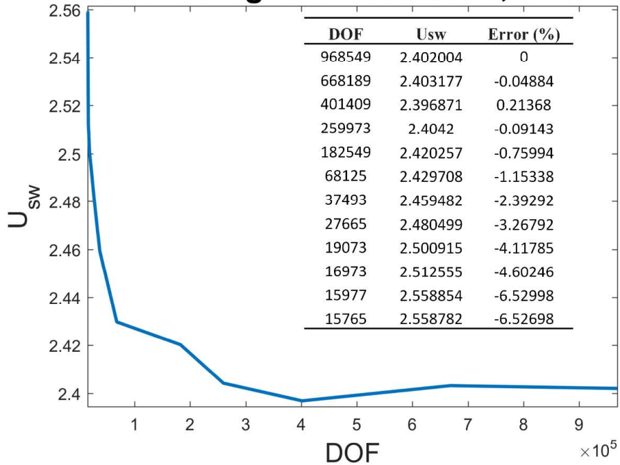
Figure 2.5 Convergence of the finite-element mesh for the filament.
