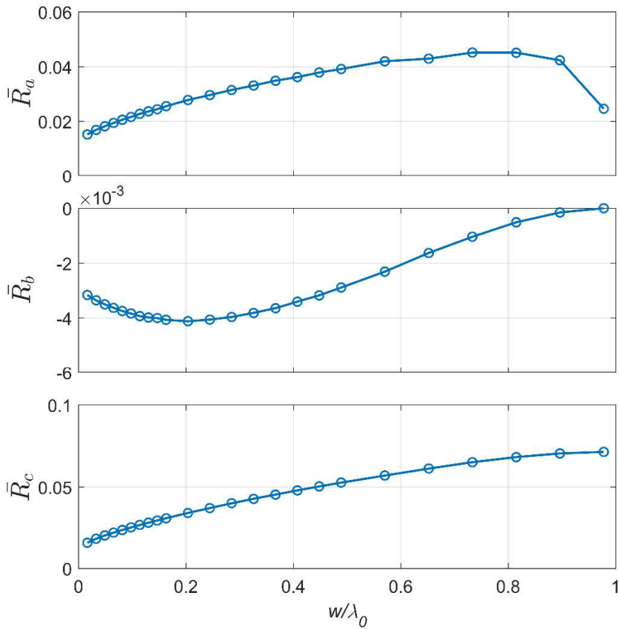
Figure 2.33 Translational, translation-rotation coupling, and rotational resistance coefficients plotted against normalized width w/\lambda_0 .
