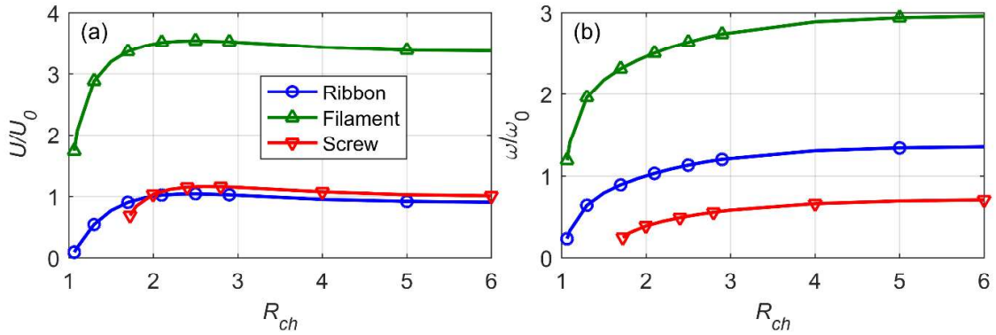
Figure 2.25 Effect of the channel radius on the swimming velocity (a), and angular velocity (b) for constant torque.
