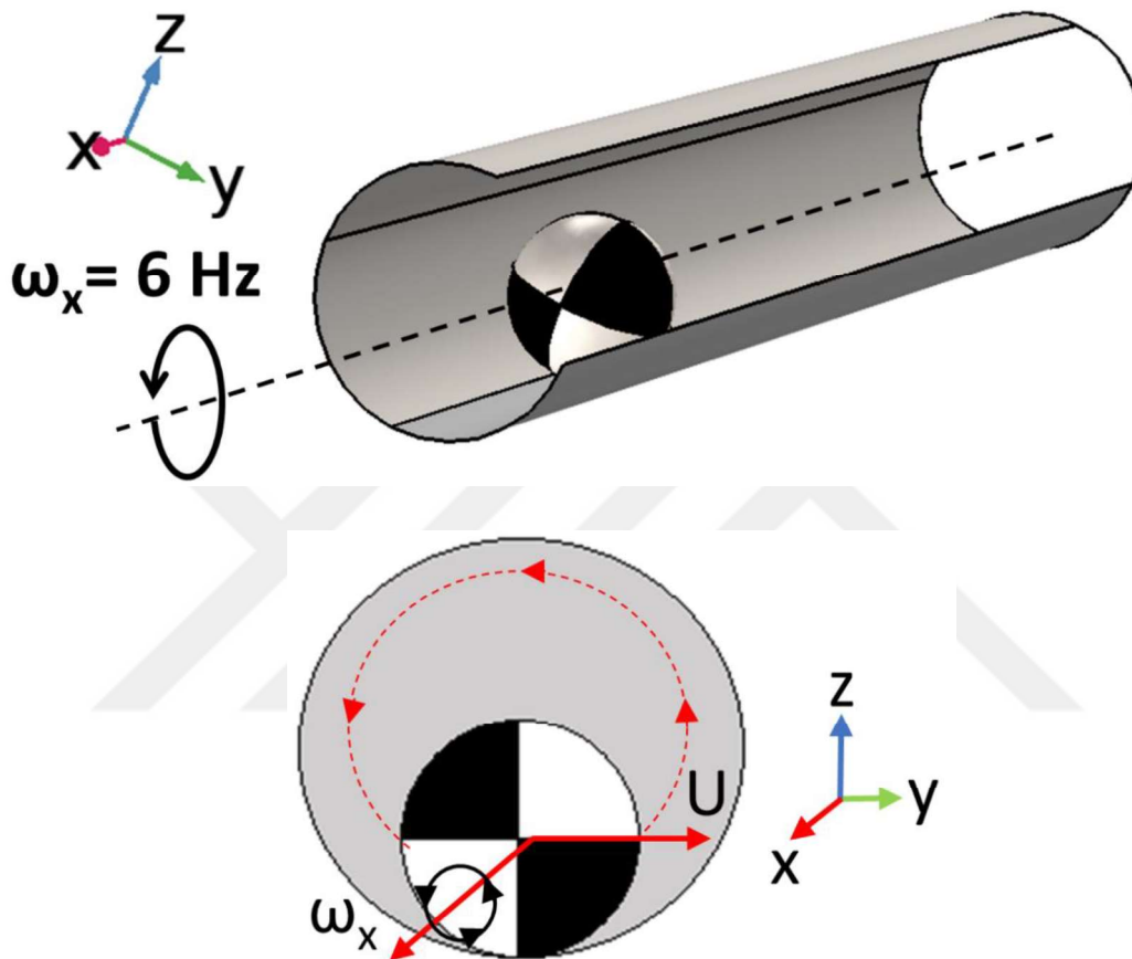
Figure 3.15 Visualization of the rotation of the sphere about x-axis under a magnetic field rotation frequency 6 Hz. No magnetic field gradient along x-axis is applied in this experiment.
