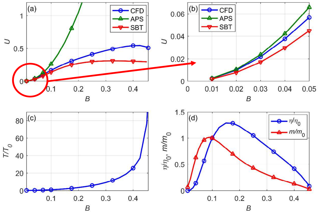
Figure 2.12 Effect of the helical amplitude, B , on the swimming velocity, U (a-b), normalized torque (c), normalized efficiency and normalized mobility (d).
