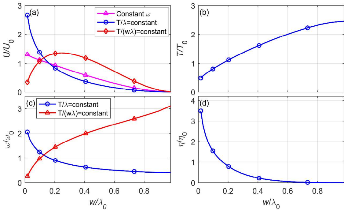
Figure 2.32 Effect of changing width, w , on swimming velocity (a), torque (b), angular velocity (c), and efficiency (d).
