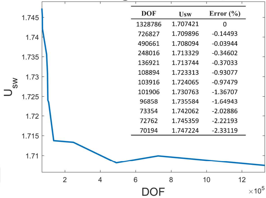
Figure 2.4 Convergence of the finite-element mesh for the ribbon with minimum thickness.
