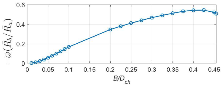
Figure 2.14 Velocity profile with respect to the changing helix radius, obtained using the resistance coefficients.
