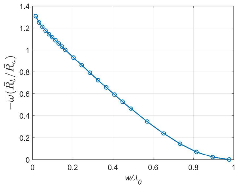
Figure 2.34 Velocity profile with respect to the changing width, obtained using the resistance coefficients.
