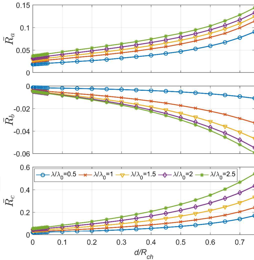
Figure 2.27 Translational, translation-rotation coupling, and rotational resistance coefficients plotted against normalized thickness d/R_{ch} for various wavelengths of the ribbon type swimmer.
