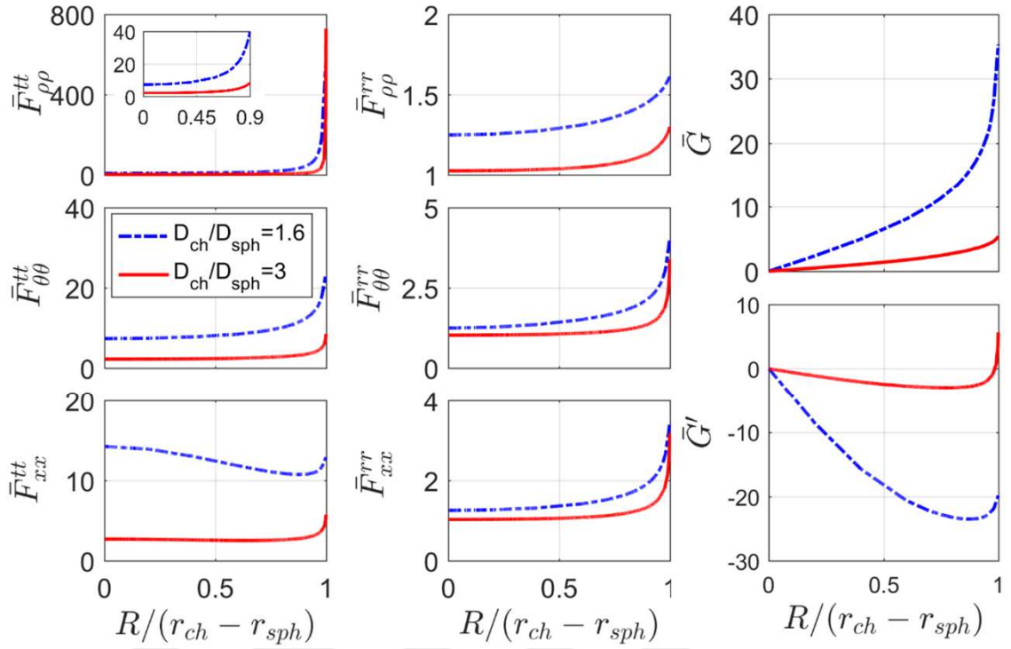
Figure 3.9 Resistance coefficients obtained using CFD model for D_{ch}/D_{sph} = 1.6 and D_{ch}/D_{sph} = 3 .
