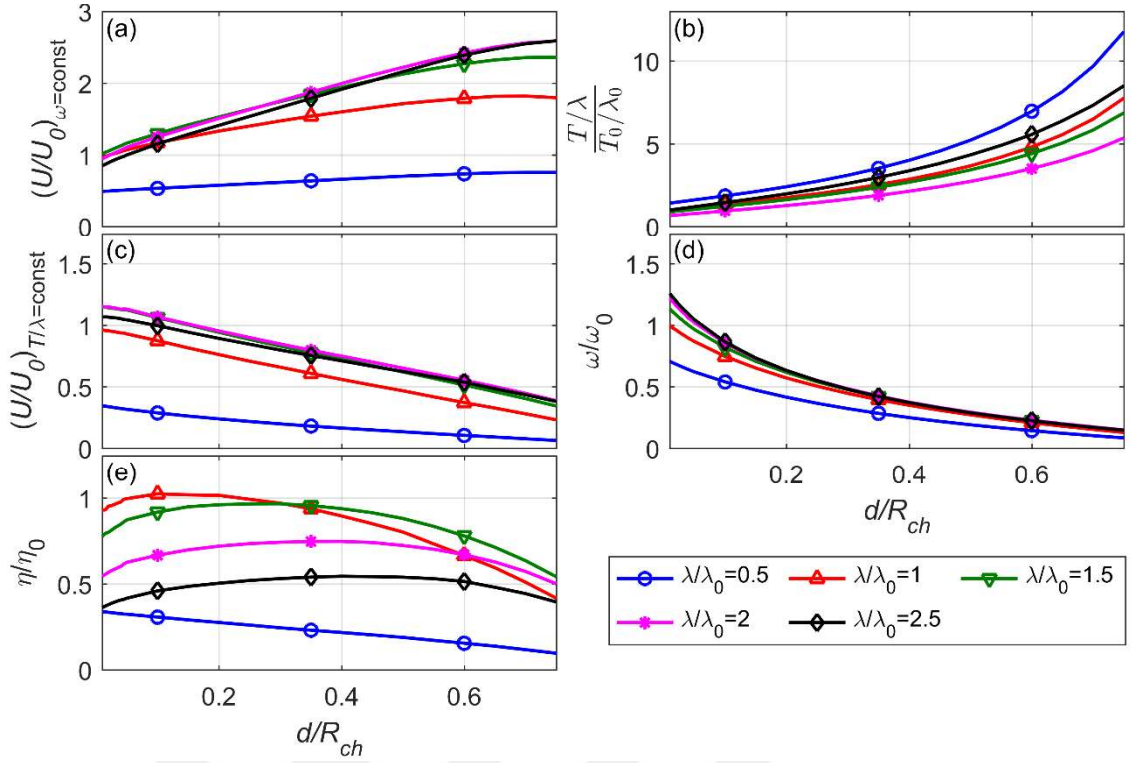
Figure 2.26 Effects of thickness and wavelength of the ribbon on the swimming velocity for constant \omega (a) and for constant torque (c); torque per wavelength for constant \omega (b); angular velocity for constant torque (d); and efficiency (e).
