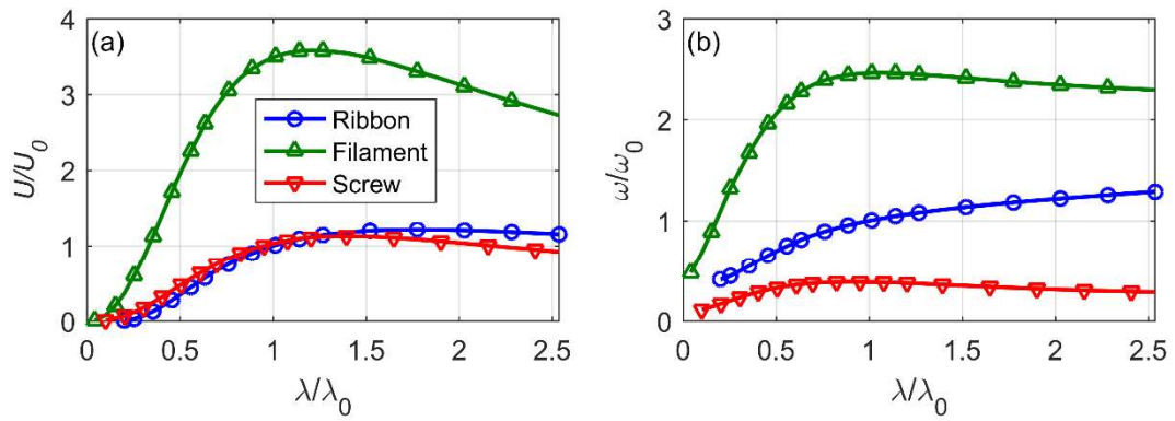
Figure 2.19 Effect of wavelength on the swimming velocity (a), and angular velocity (b) for constant torque per length.
