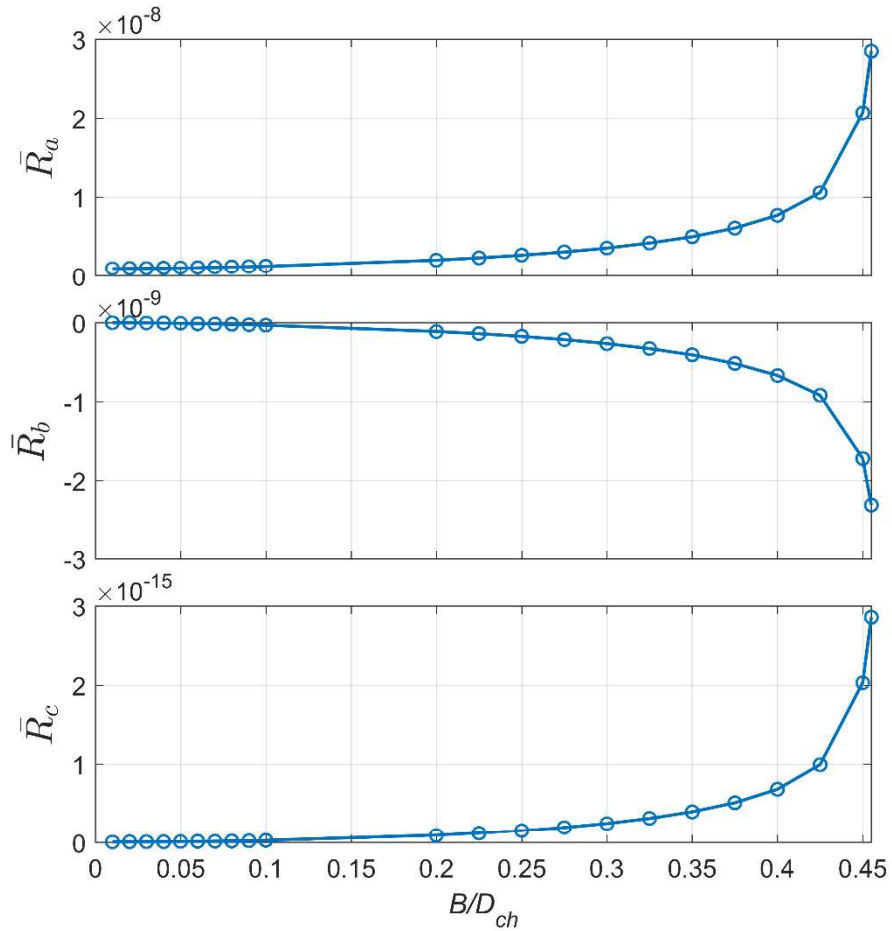
Figure 2.13 Translational, translation-rotation coupling, and rotational resistance coefficients plotted against normalized helix radius B/D_{ch} .
