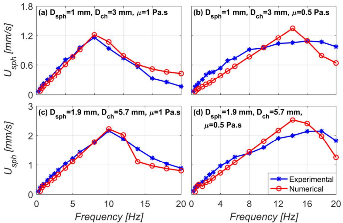
Figure 3.24 Comparison of the experimental results to the numerical predictions for D_{ch}/D_{sph} = 3 for two different silicone oil viscosities of \mu = 1 Pa.s and \mu = 0.5 Pa.s.
