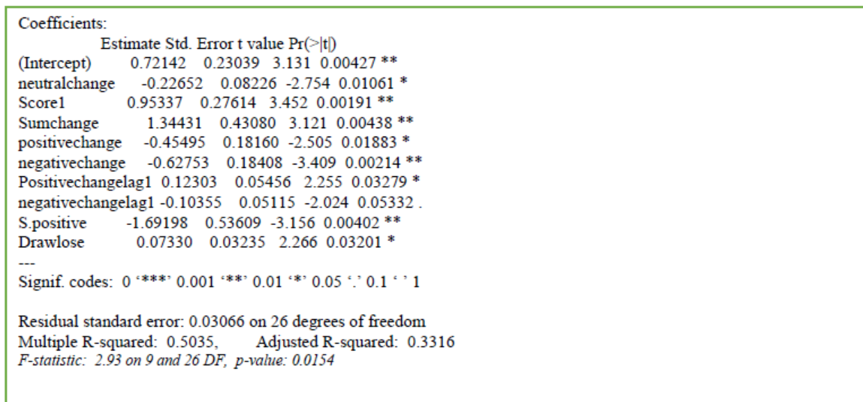
Figure 18: R output for Model 3 Trabzonspor
