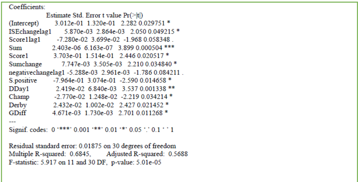
Figure 17: R output for Model 3 Galatasaray
