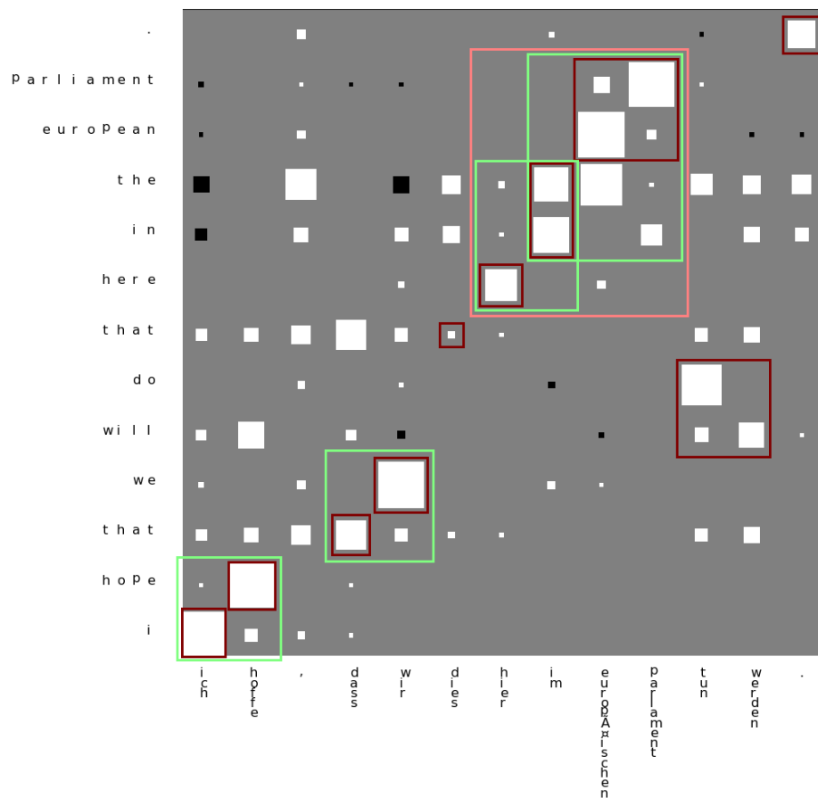
Figure 4.5: L_1 Regularized Regression for word alignment figure, FSR, with phrases identified, using 1000 training instances.
