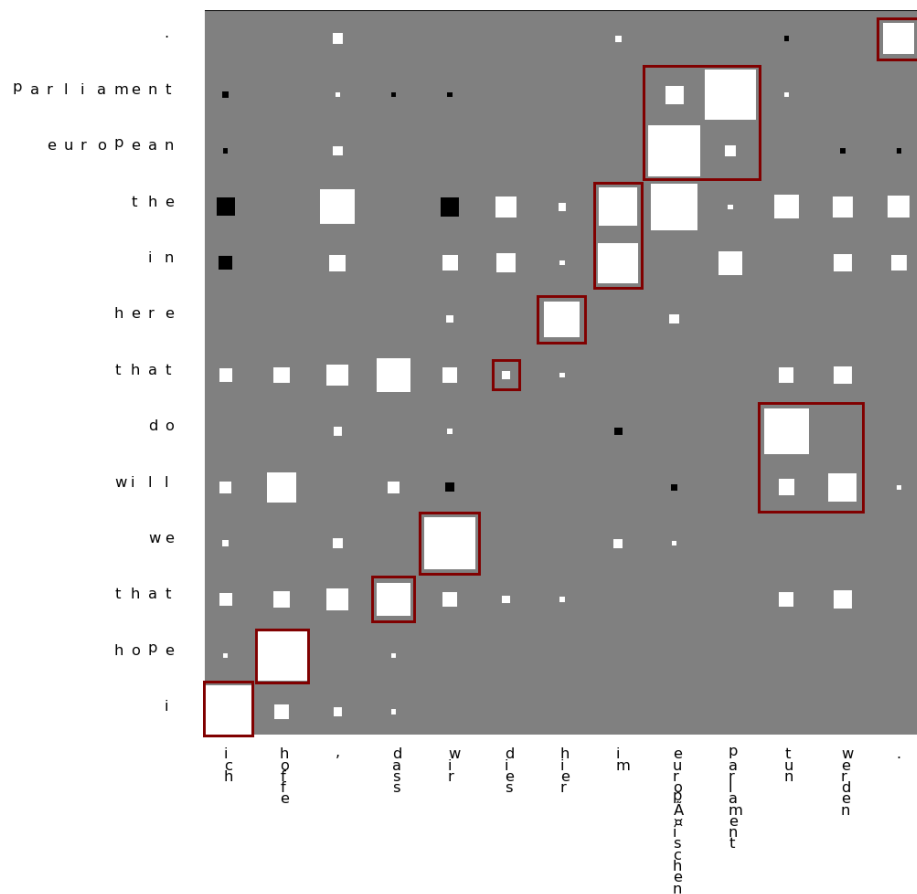
Figure 4.4: L_1 Regularized Regression for word alignment figure, FSR, 1000 training instances.
