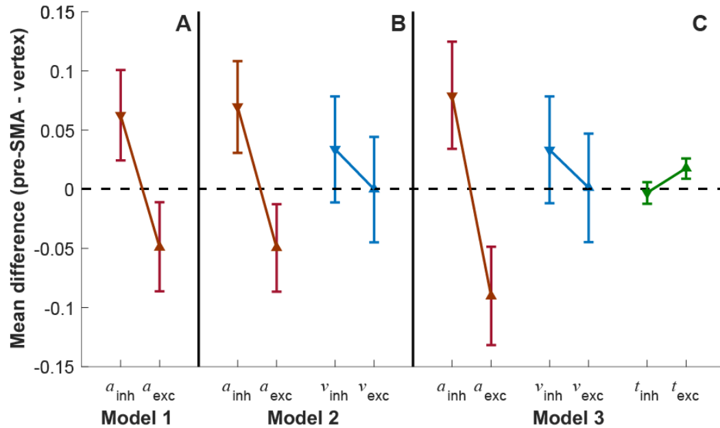
Figure 2. Mean difference in the threshold ( a ; red), drift rate ( v ; blue), and non-decision time ( t ; green) parameters between pre-SMA inhibition and control (up arrowhead) and pre-SMA excitation and control (down arrowhead) conditions for Models 1 (A), 2 (B), and 3 (C). Error bars indicate 95% credible intervals. Note that positive differences indicate higher values in the pre-SMA compared with vertex stimulation conditions, whereas negative values indicate lower values in pre-SMA compared with vertex stimulation conditions.
