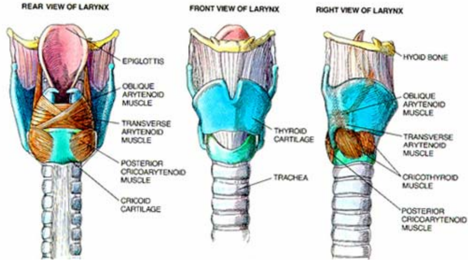
Şekil-13:Larinks ( www.pitt.edu/~crosen/voice/anatomy2.html )
