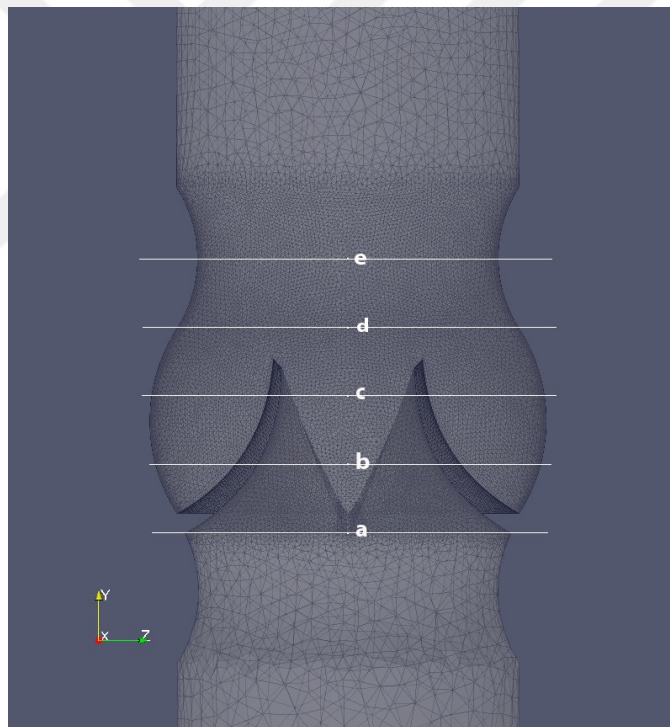
Figure 5.5 : Cross lines to observe flow parameters.
