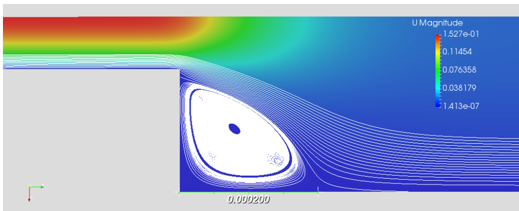
Figure 4.5 : Velocity contours of the numerical results for Re = 12.2 with 1% hardened human red cells ( d_p = 7.5 \mu m , \rho = 1.13 g/cm^3 ) dispersed in water ( \rho = 1.0 g/cm^3 , \mu = 0.01 P ).
