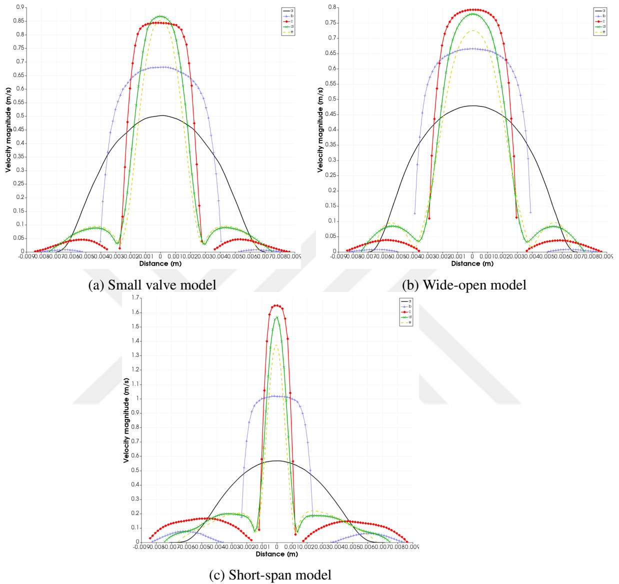
Figure 5.7 : Velocity profiles of RBCs on the sample lines.
