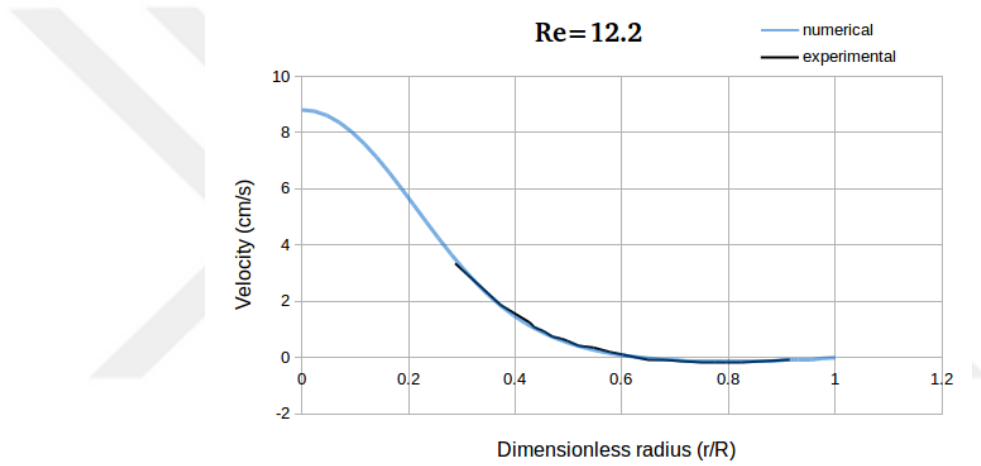
(a) Re = 12.2 and U_{inlet} = 75.7 \text{ mm/s}
