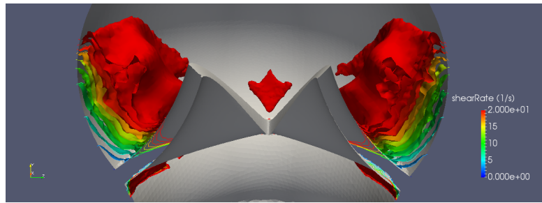
(a) Small valve model
