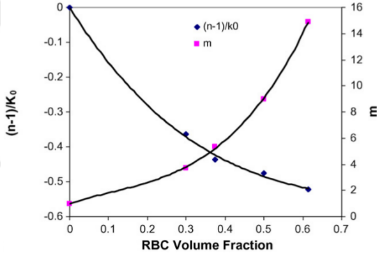
Figure 3.2 : m and n versus RBC volume fraction at low shear rates ( (1 + (\lambda\gamma)^2 \leq 1.5) ). Experimental data is marked by points at different hematocrits and shear rates, picture from [24].
