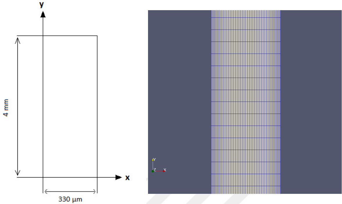
Figure 4.1 : The sizes and the mesh structure of the micro-channel model.
