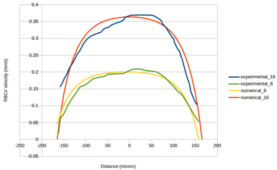
Figure 4.3 : The velocity profile of RBCs as a function of x on the sample line at y=2.5\text{ mm} , and depth z=16\mu m , z=8\mu m with the experimental data.
