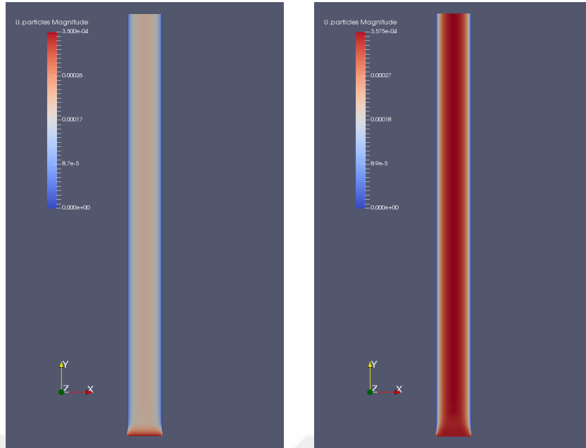
Figure 4.2 : Velocity contours of RBCs in the micro channel model for the cross section of 8\mu m and 16\mu m , respectively.
