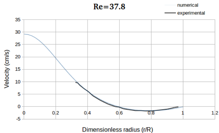
(b) Re = 37.8 and U_{inlet} = 233 \text{ mm/s}
