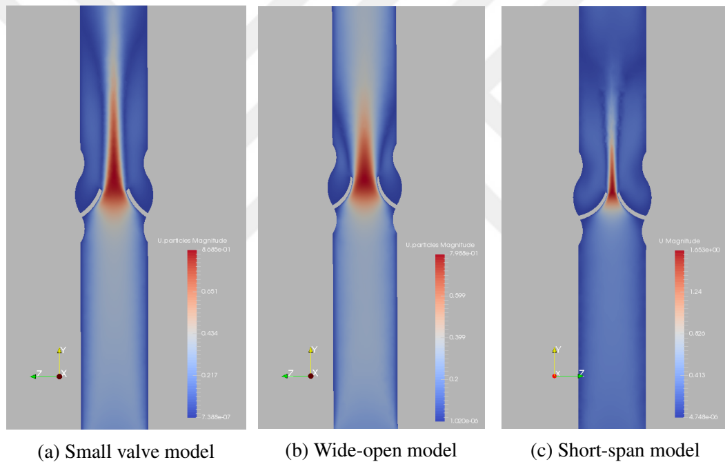
Figure 5.1 : RBCs' velocity profiles (m/s) at 1s.
