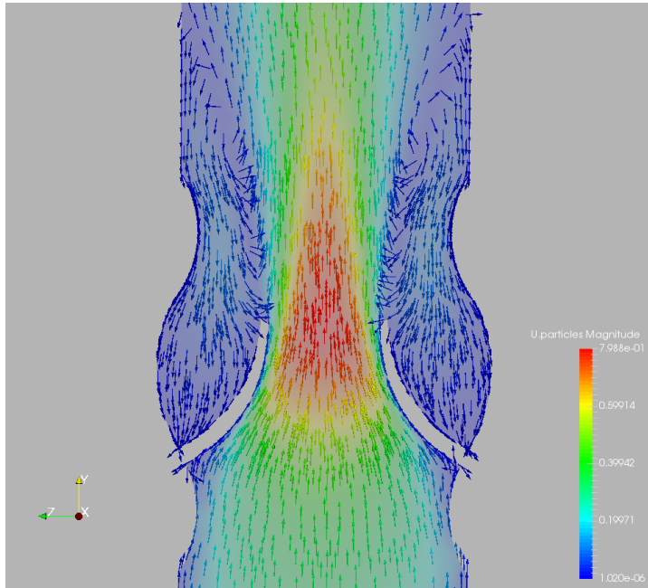
Figure 5.4 : Velocity vectors at 1s for the second model.
