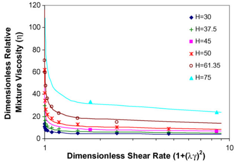
Figure 3.1 : Dimensionless relative blood viscosity versus dimensionless shear rate and hematocrit, experimental data from [51, 67], picture from [24].
