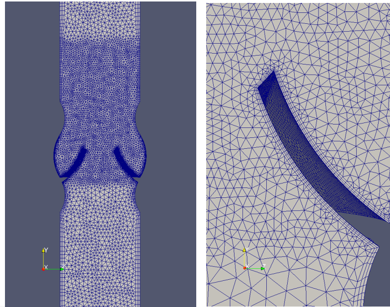
(a) Symmetry plane.
