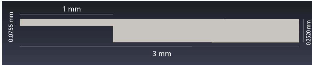
Figure 4.4 : Sizes of the expansion channel model
