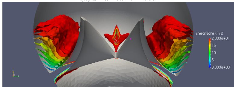
(b) Wide-open model
