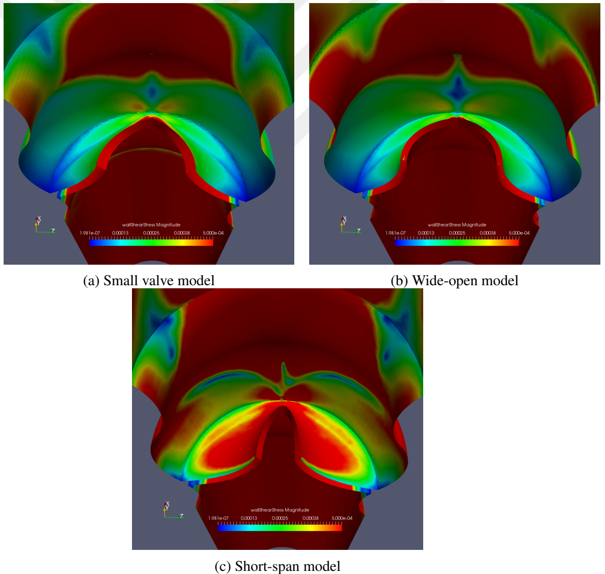
Figure 5.10 : Wall Shear Stress Contours near valve.
