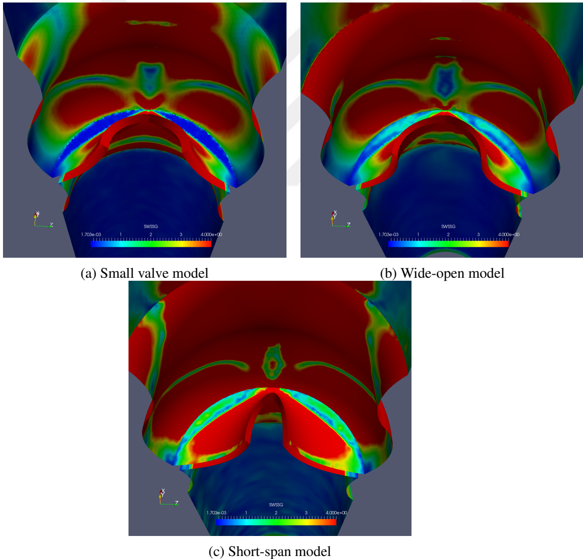
Figure 5.11 : Spatial Wall Shear Stress Gradient Contours near valve.
