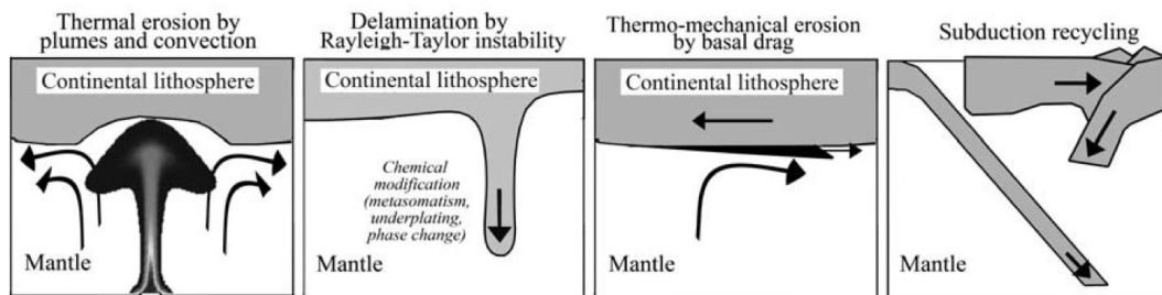
Figure 1.4 : The large-scale deformation types of lithosphere (Artemieva, 2011).
