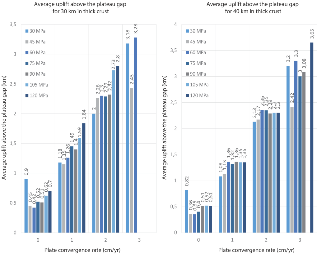
Figure 5.1 : The plot shows the average uplift amounts in the post-delamination break-off cases. 30 km and 40 km in thick upper crust is used and the values over the bars shows the amount of uplifted topography in 18 Myr.
