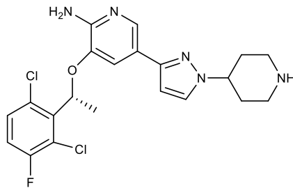
Crizotinib
