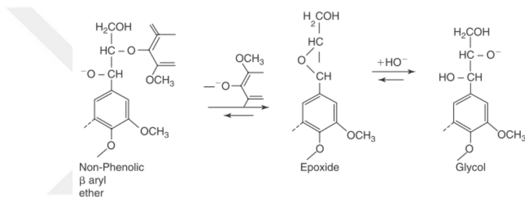
Figure 1.7: Main reactions leading to the formation of soda lignin (Gellerstedt and Henriksson, 2008)
