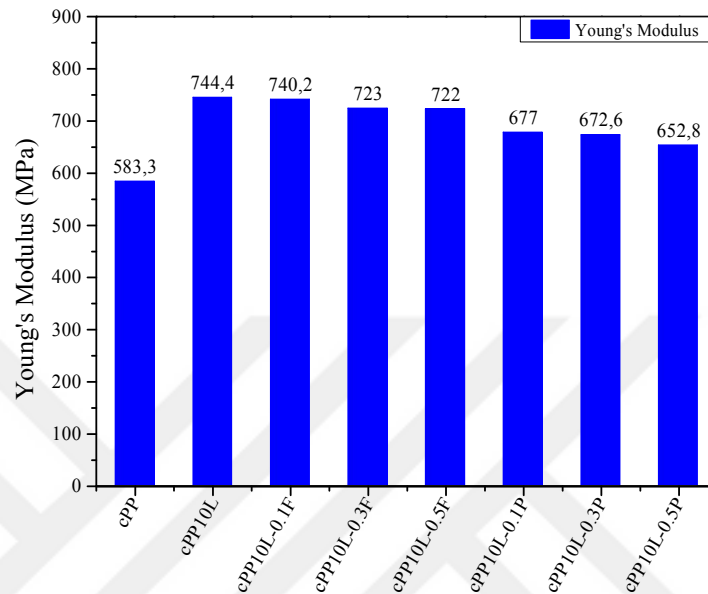
Figure 3.4: Young’s modulus of copolymer and composites
