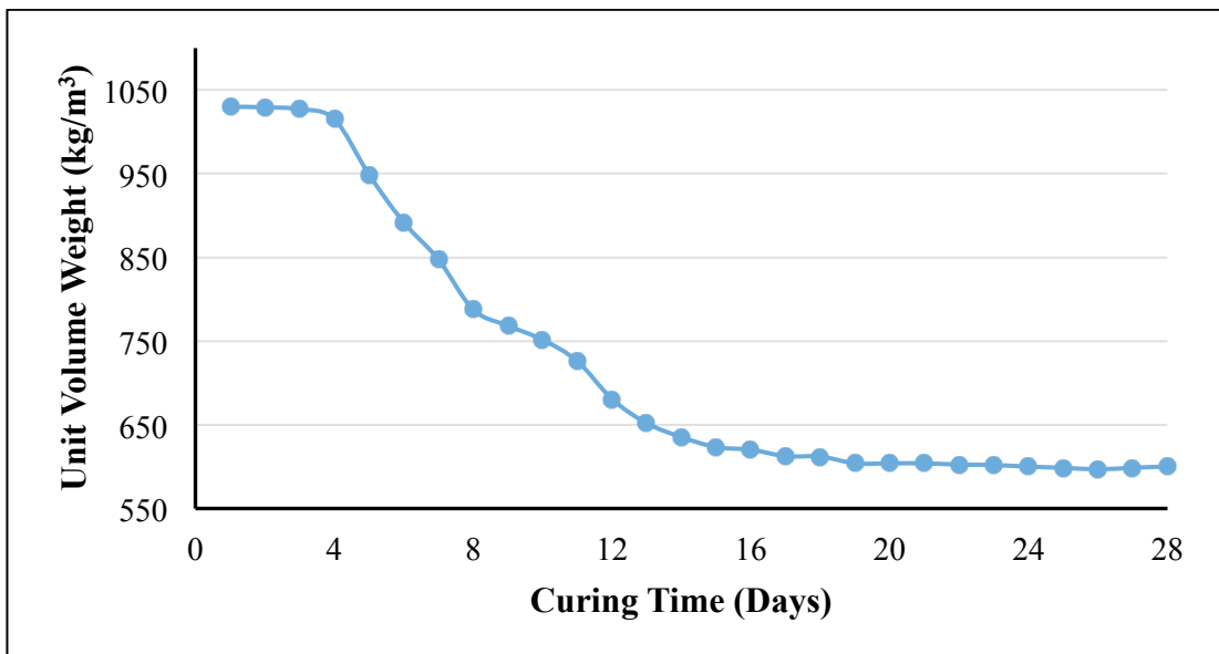
Figure 4.6 : UVW vs curing time for plaster containing 4.0% cotton fiber.
