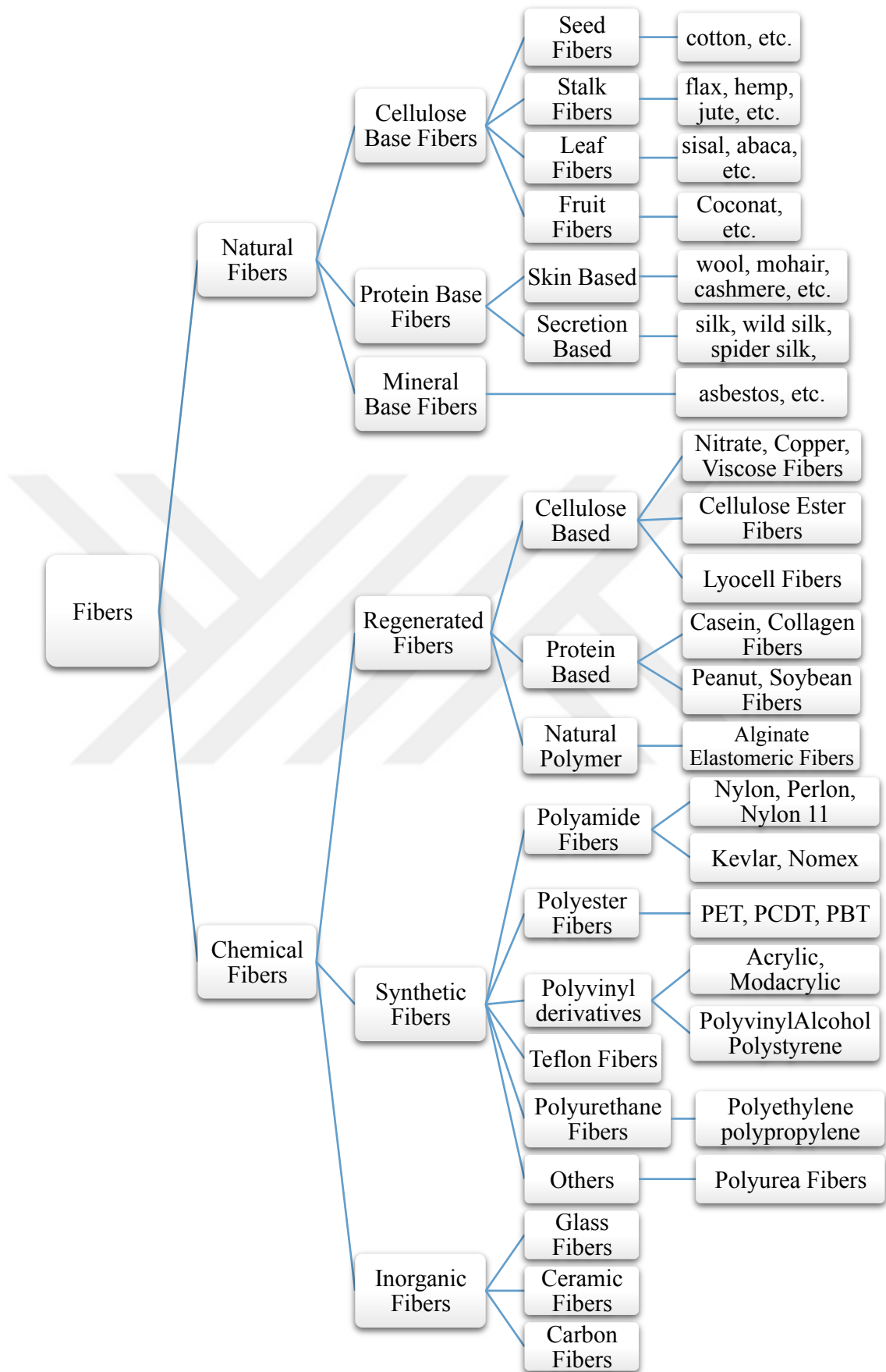
Figure 2.6 : Classification of textile fibers.
