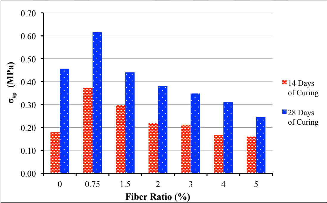
Figure 4.53 : The relation between splitting tensile strength and mixture of cotton+polyester+acrylic fiber ratio.
