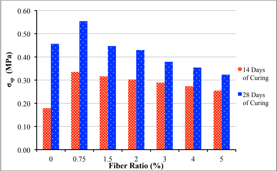
Figure 4.55 : The relation between splitting tensile strength and polyester fiber ratio.
