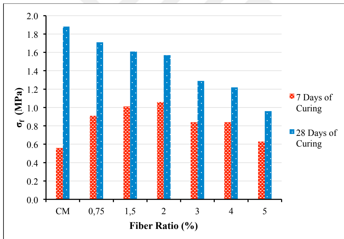
Figure 4.41 : Flexural strength vs cotton fiber ratio.
