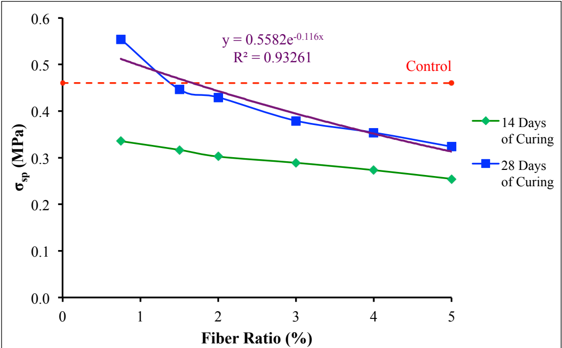
Figure 4.56 : The relation between splitting tensile strength and polyester fiber ratio.
