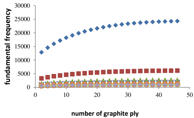
Figure 6.1 : fundamental frequency and cost of laminated composite for 28 and 48 ply depends on aspect ratio and number of graphite ply
