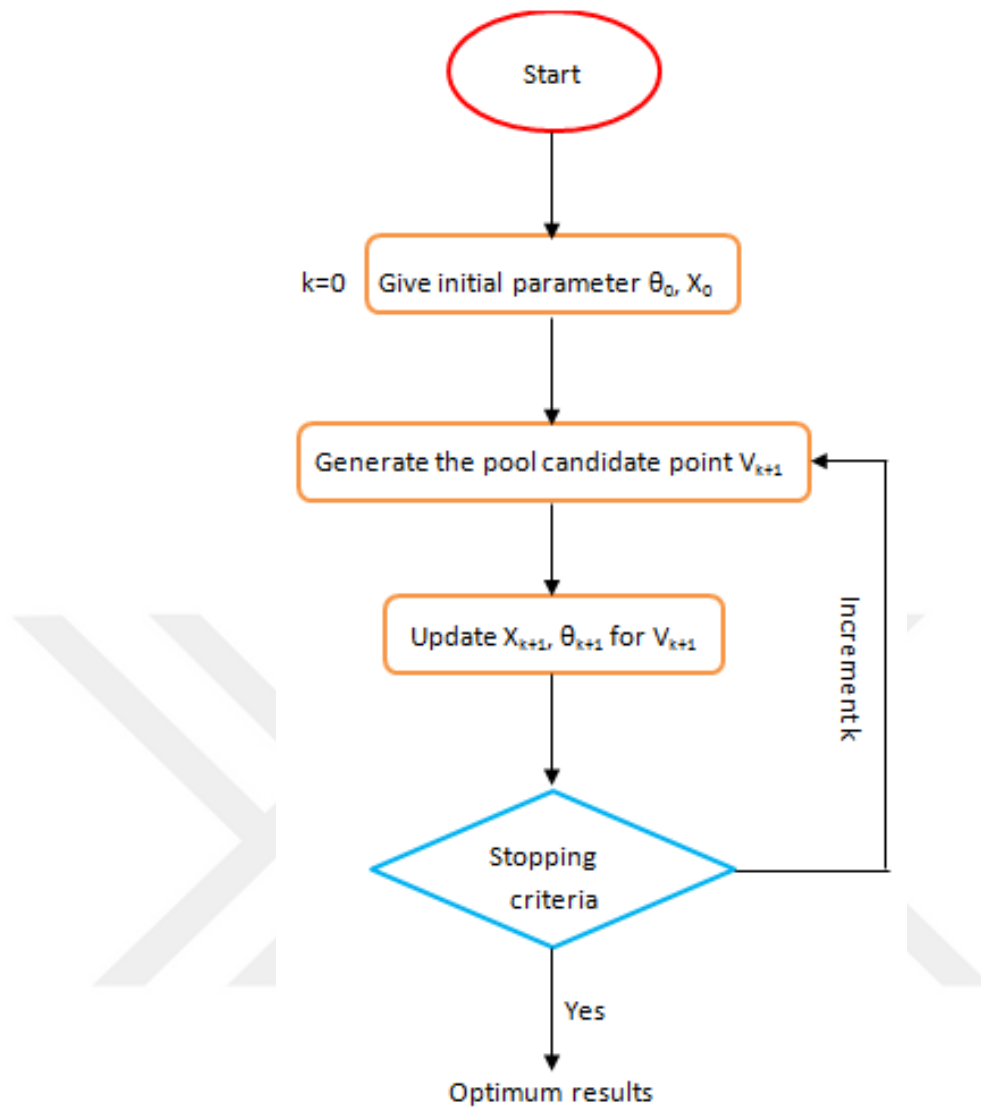
Figure 4.3 : Flowchart of the RS algorithm. (Adapted from Zabinsky, 2011)
