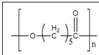
Figure 1.3 : Polycaprolactone formula.
