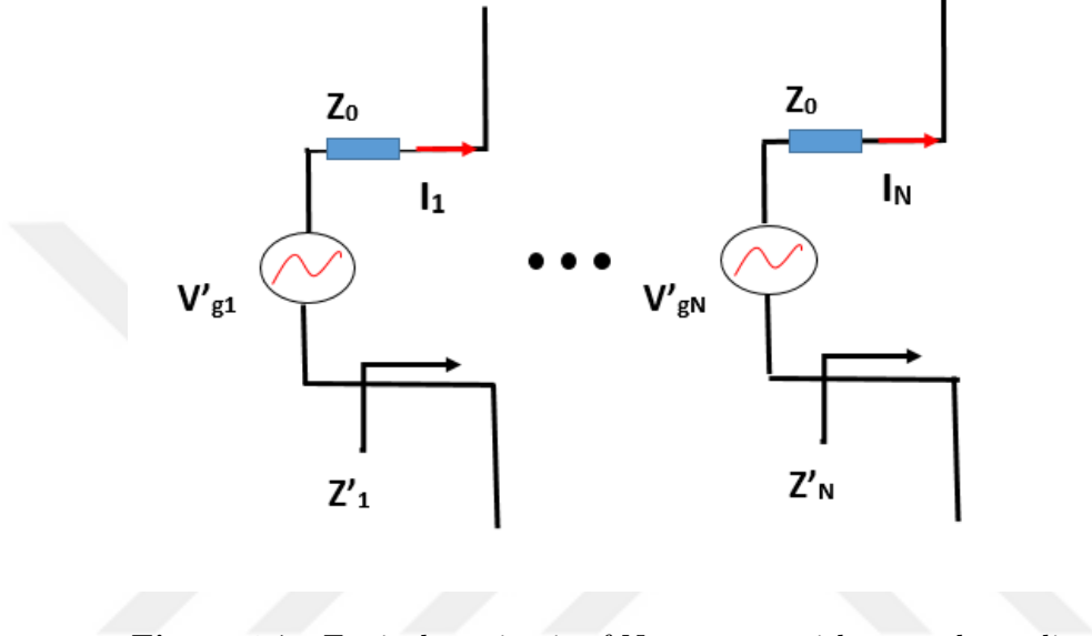
Figure 2.7: Equivalent circuit of N antennas with mutual coupling
