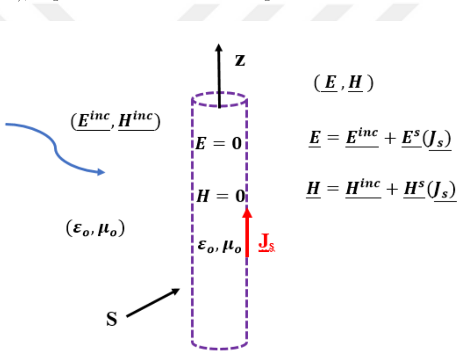
Figure A.2: Surface equivalence model with equivalent surface current density \underline{J}_s in free space.
