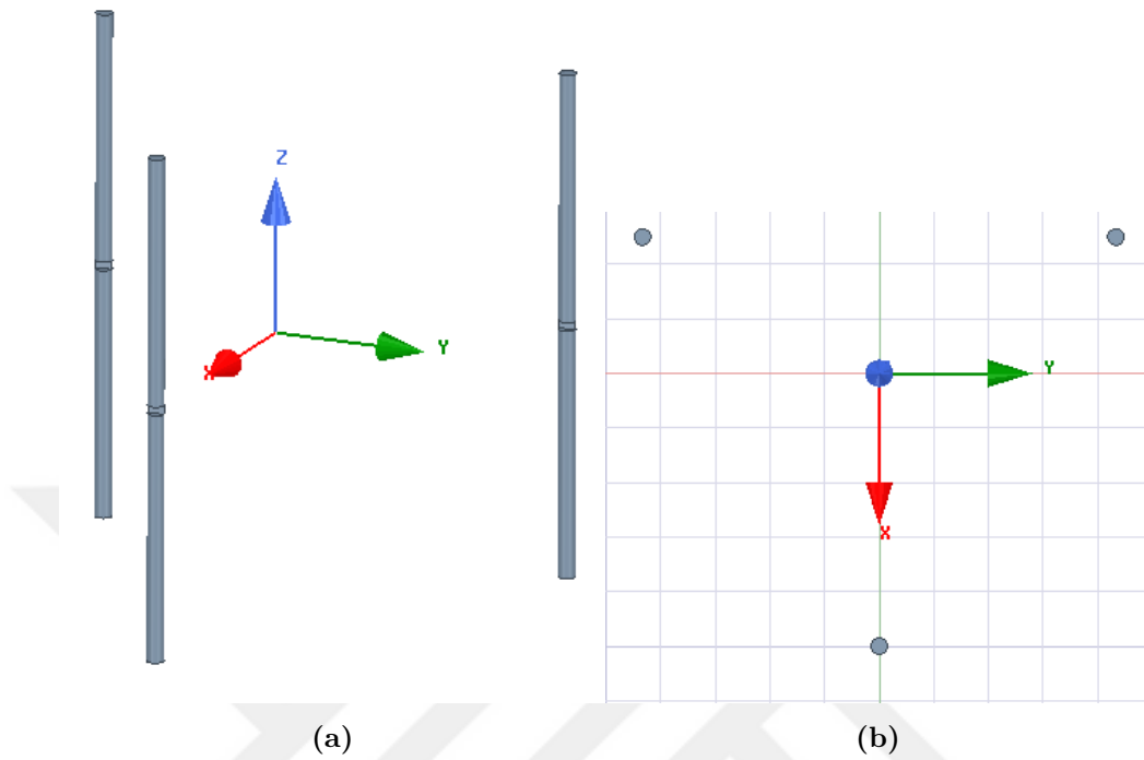
Figure 3.35: Triangular array of three dipole antennas. a) Side view. b) Top view.
