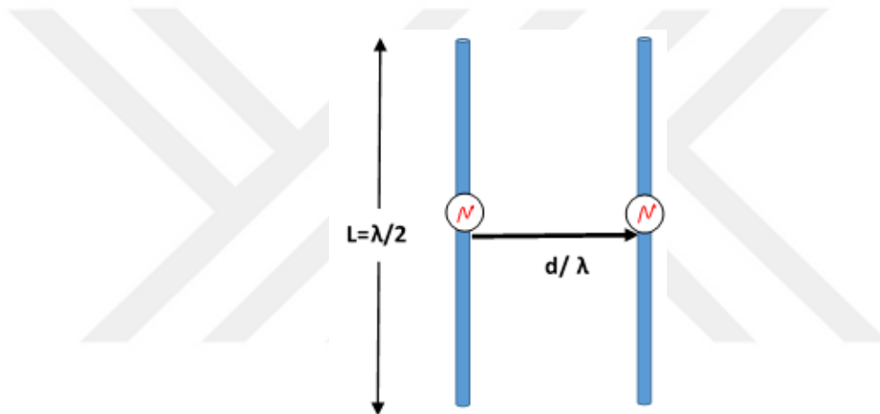
Figure 3.10: Two parallel antennas of length \lambda/2 with a = \lambda/200 .
