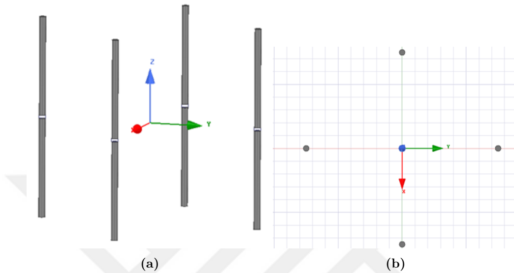
Figure 1.1: Circular array of four half-wave dipoles with radius of circle \lambda/4 . a) Side View. b) Top View.
