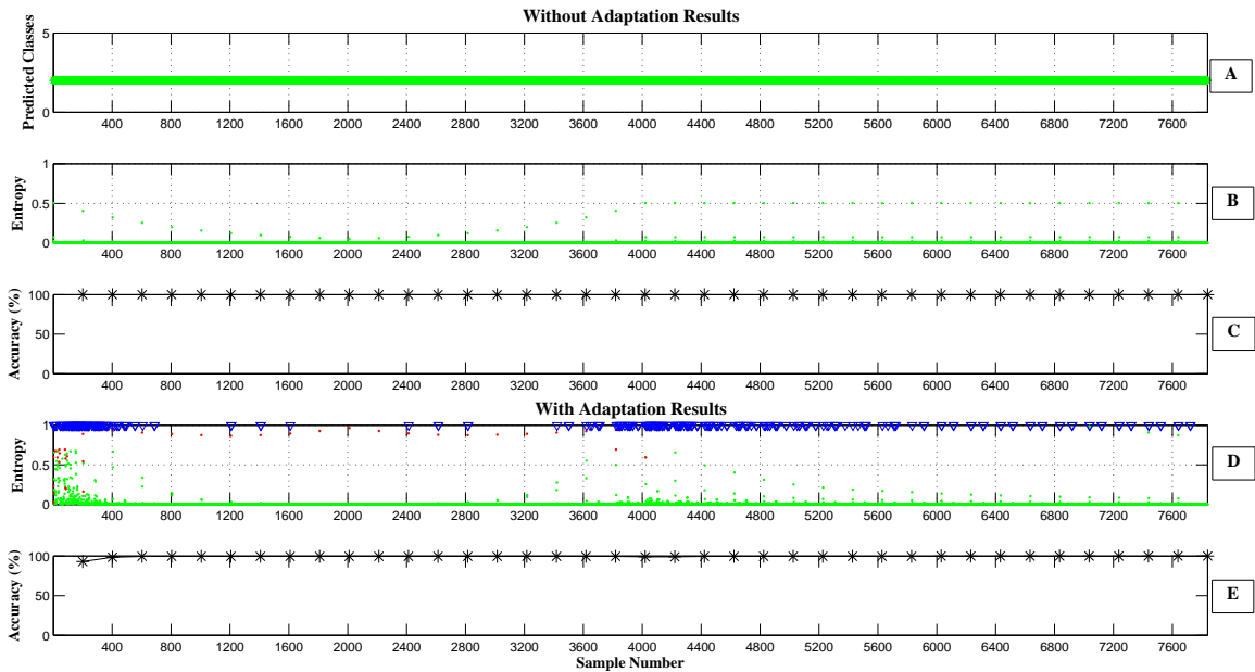
Figure 2.17: The classification accuracy results for type 2 distorted (DT2) for wrist extension movement. The classification results where no adaptation is applied are shown in graphs A, B and C. A) The output class labels of the network for each data point(sample). Class labels are represented by numbers 1 to 4 for wrist flexion, wrist extension, hand close, hand open movements, respectively. Green stars and red stars represent true and wrong classified samples by the classifier, respectively. B) Entropy after each decision of the classifier. C) Classification accuracy calculations shown by black stars for every 200 samples. Classification results where adaptation is applied are shown in graphs D & E. D) Entropy after each classification (adaptation is applied during classification). E) Classification accuracy calculations for every 200 samples shown by black stars. The samples where the adaptation applied marked by blue vertical triangles.
