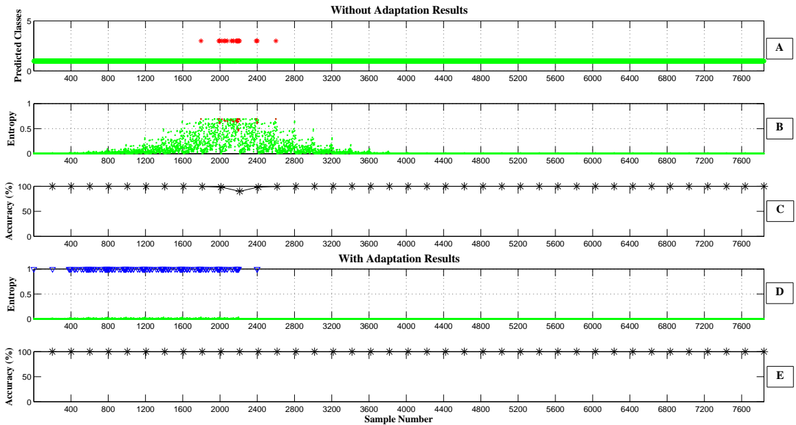
Figure 2.15: The classification accuracy results for type 2 distorted (DT2) for wrist flexion movement. The classification results where no adaptation is applied are shown in graphs A, B and C. A) The output class labels of the network for each data point(sample). Class labels are represented by numbers 1 to 4 for wrist flexion, wrist extension, hand close, hand open movements, respectively. Green stars and red stars represent true and wrong classified samples by the classifier, respectively. B) Entropy after each decision of the classifier. C) Classification accuracy calculations shown by black stars for every 200 samples. Classification results where adaptation is applied are shown in graphs D & E. D) Entropy after each classification (adaptation is applied during classification). E) Classification accuracy calculations for every 200 samples shown by black stars. The samples where the adaptation applied marked by blue vertical triangles.
