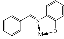
ON tipi ligand
